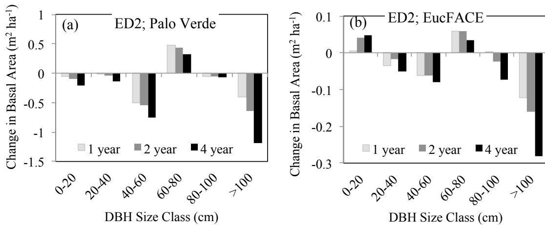
Figure S3. Change in basal area ( \text{m}^2 \text{ha}^{-1} ) immediately following either 1, 2, or 4 year droughts for six increasing size class bins (DBH, cm) as predicted by the ED2 model for (a) the Palo Verde site, with 90% precipitation removed, and (b) the EucFACE site with 50% precipitation removed.
