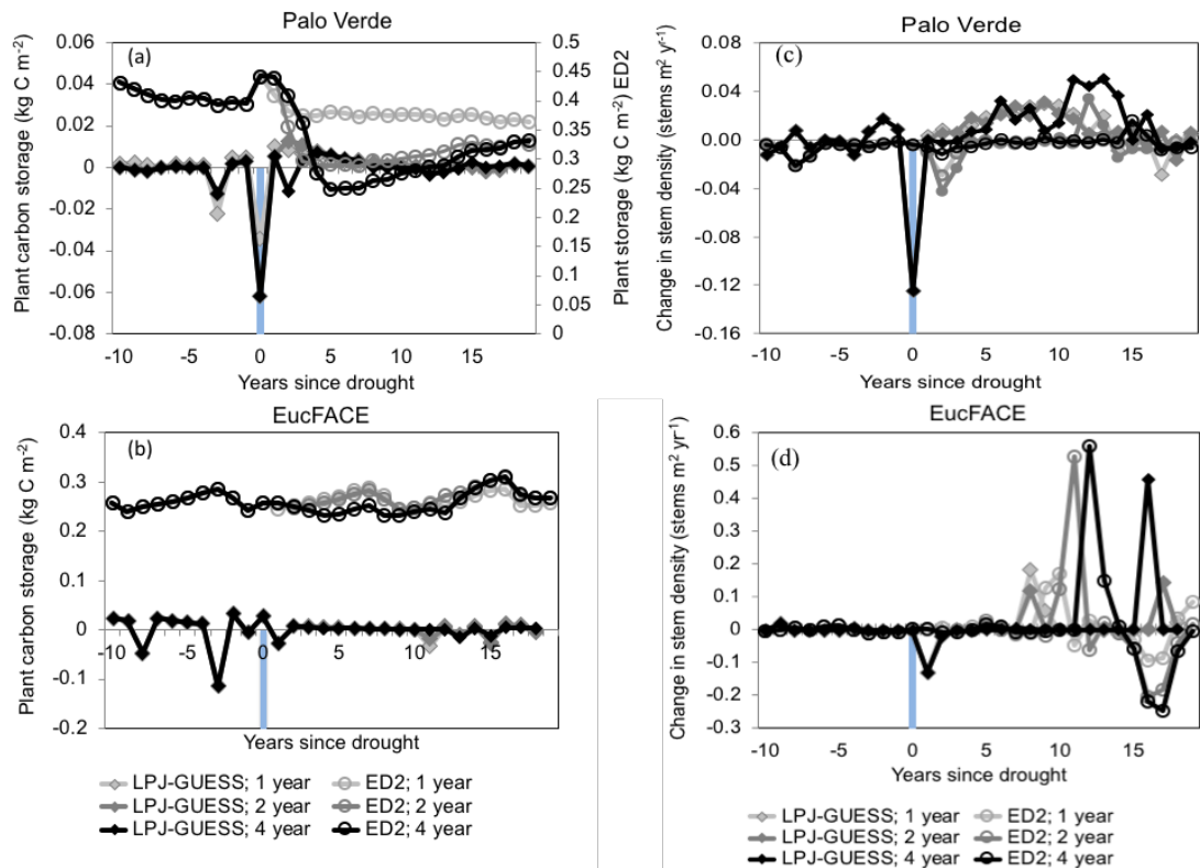
Figure S2. Change in plant carbohydrate storage ( \text{kg C m}^{-2} ) (a-b) and change in stem density ( \text{stems m}^{-2} \text{yr}^{-1} ) (c-d) as a result of three drought durations events (1 year, 2 year, and 4 year durations) compared to the pre-drought period (i.e. negative years) and over a 20-year recovery period, for both the LPJ-GUESS and ED2 demography models at the Palo Verde site and EucFACE site. The modeled drought intensity at Palo Verde was 90% precipitation removed, and 50% precipitation removed at EucFACE.
