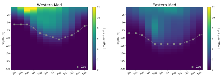
Figure S2: Hovmöller plot of net primary production in western (left) and eastern Mediterranean (right) in 1999-2019 reanalysis simulation. Gray squares represent the euphotic depth (Zeu), i.e. the depth at which the modelled PAR is 1% of its surface value.
