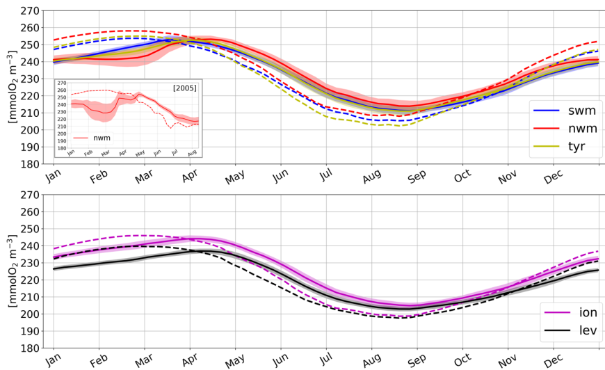
Figure A1: Modelled oxygen concentration (solid lines) and oxygen saturation (dashed lines) at the surface in selected open-sea aggregated subbasins in the western (top) and eastern (bottom) Mediterranean Sea, computed over the climatological year (i.e., by temporally averaging values over the 1999-2019 period). Shaded bands represent the temporal variability of surface oxygen computed as the standard deviation of annual means. The box at the top of the top figure represents the modelled oxygen and its saturation at the surface in the nwm subbasin in 2005, with shaded bands representing the spatial variability of surface oxygen within the subbasin.
