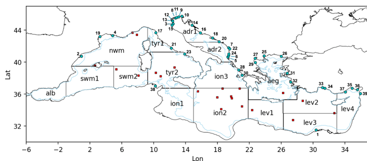
200 Figure 2: Mediterranean Sea domain, with the bathymetric contour at 200 m (light blue line) and cyan dots with numbers corresponding to the main river mouth positions: Nile (1), Ebro (2), Po (3), Rhone (4), Vjosë (5), Seman (6), Buna/Bojana (7), Piave (8), Tagliamento (9), Soca/Isonzo (10), Livenza (11), Brenta-Bacchiglione (12), Adige (13), Lika (14), Reno (15), Krka (16), Arno (17), Nerveta (18), Aude (19), Trebisnjica (20), Tevere (21), Mati (22), Volturno (23), Shkumbini (24), Struma/Strymonas (25), Meric/Evros/Maritsa (26), Axios/Vadar (27), Arachtos (28), Piniös (29), Acheloos (30), Gediz (31), Büyük Menderes (32), Kopru (33), Manavgat (34), Seyhan (35), Ceyhan (36), Gosku (37), Medjerda (38), Asi/Orontes (39). Subbasins used in the validation procedure are indicated by black contours and acronyms. According to data availability and to ensure the consistency and robustness of the metrics, aggregated subbasins were also used: swm = swm1+swm2; tyr = tyr1+tyr2; adr = adr1+adr2; ion = ion1+ion2+ion3; lev = lev1+lev2+lev3+lev4. Red squares indicate the sampling locations of planktonic metabolism observations. 205
