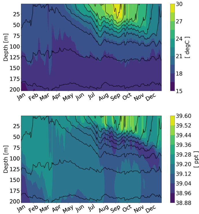
Figure S1: Hovmöller plot of model-derived temperature (top) and salinity (down), with density contours (in black) in E area (Fig. 7) in 2014.
