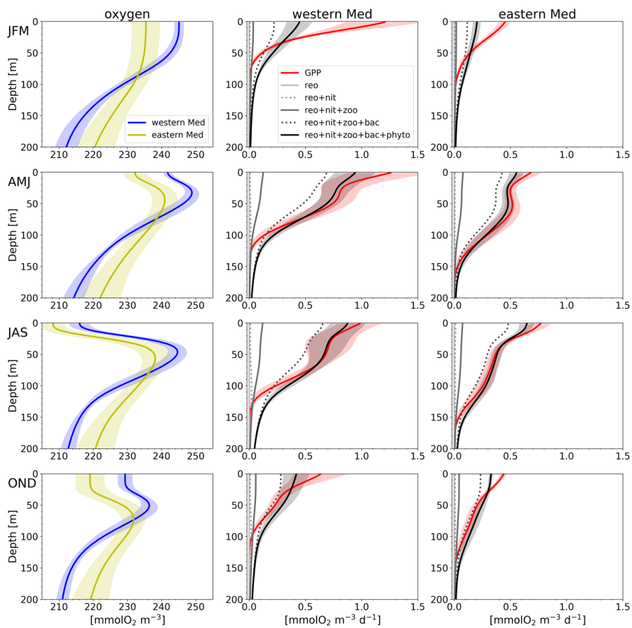
485 Figure 5: Modelled climatological profiles in the epipelagic layer for the oxygen concentration (first column) and daily rate of oxygen concentration associated with biological processes in the western Mediterranean Sea (western Med, second column) and eastern Mediterranean Sea (eastern Med, third column) in the winter (JFM), spring (AMJ), summer (JAS) and fall (OND) seasons, 490 corresponding to the four rows. Biological processes represented are gross primary production (red solid line) and cumulative consumption (alternating solid and dotted lines, in greyscale): reoxidation of reduction equivalents (reo), nitrification (nit) and zooplankton (zoo), bacterioplankton (bac) and phytoplankton (phyto) respiration. Shaded bands represent the spatial variability computed as the standard deviation of the climatological profiles in the western Med and eastern Med. The northern Adriatic Sea was excluded from the computation since its depth is mostly lower than 200 m.
