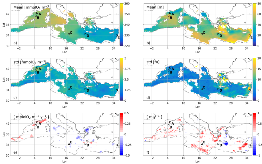
Figure 6: Mean concentration (a) and depth (b) for the modelled SOM in summer, computed by averaging the annual maximum vertical values of the mean oxygen concentration in the JAS months and their associated depths, respectively, in the period of 1999-2019; standard deviation of the annual maximum values (c) and their depths (d), in the same period; trends evaluated in concentration (e) and depth (f) by the Theil-Sen method and provided only if significant as obtained from Mann-Kendall test ( p=0.05 ), in the same period. Areas A-E delimited by black squares are hereafter defined as follows: A = Gulf of Lion, B = Balearic front, C = central Ionian, D = western Cretan gyre, E = eastern Levantine (area). Coastal areas (i.e., with depths higher than 200 m) are masked.
