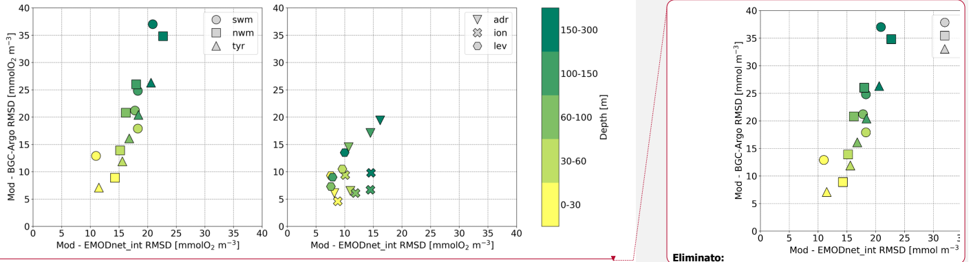
Figure 4: Mean RMSD between modelled oxygen outputs and BGC-Argo floats versus mean RMSD of modelled oxygen outputs and the EMODnet_int dataset in open-sea aggregated subbasins in the western (left) and eastern (right) Mediterranean Sea. Metrics are computed for selected layers (0-30 m, 30-60 m, 60-100 m, 100-150 m, and 150-300 m) and averaged over the 1999-2019 time period.
