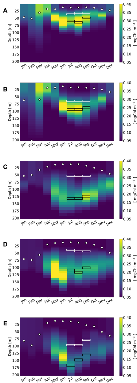
Figure S3: Hovmöller plot of mean model-derived monthly chlorophyll concentration in the Mediterranean areas indicated in Fig. 6 in 2014. White circles indicate the depth of the mixed layer, black and white rectangles the depth of DCM and SOM in the summer period (JAS months), respectively.
