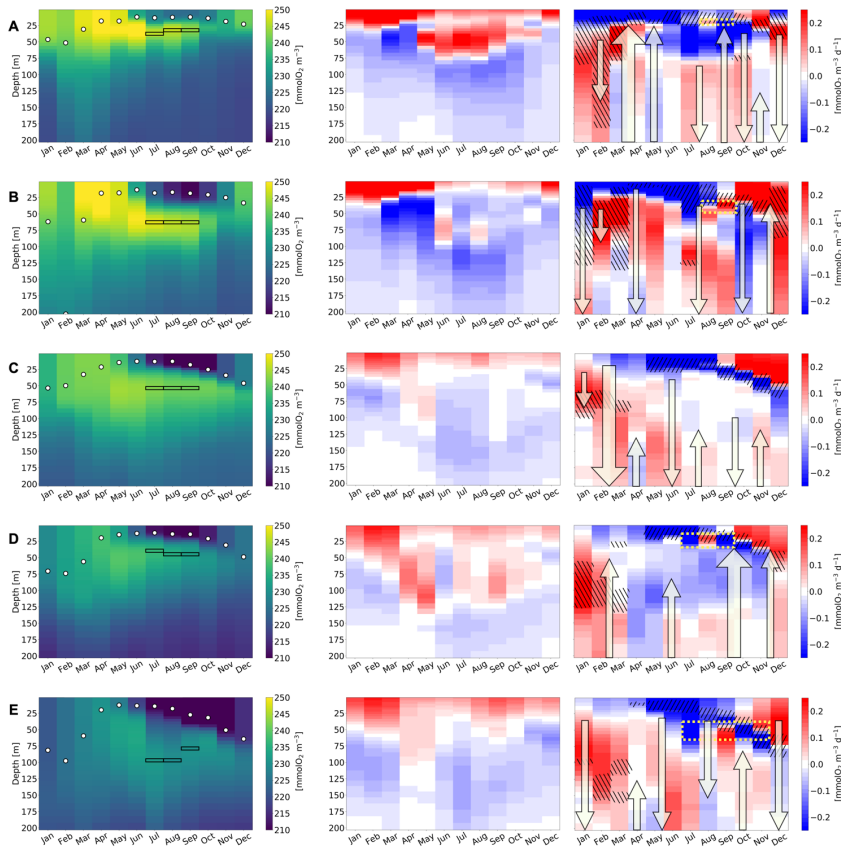
635 Figure 7: Hovmöller plot of monthly variables computed in areas A-E (Fig. 6) in 2014: oxygen concentration, with the depth of the maximum in summer months indicated by black rectangles and the mixed layer depth by white circles (left column), with the biological derivative in \text{mmolO}_2 \text{ m}^{-3} \text{ d}^{-1} (central column) and the physical derivative in \text{mmolO}_2 \text{ m}^{-3} \text{ d}^{-1} (right column). In the right
