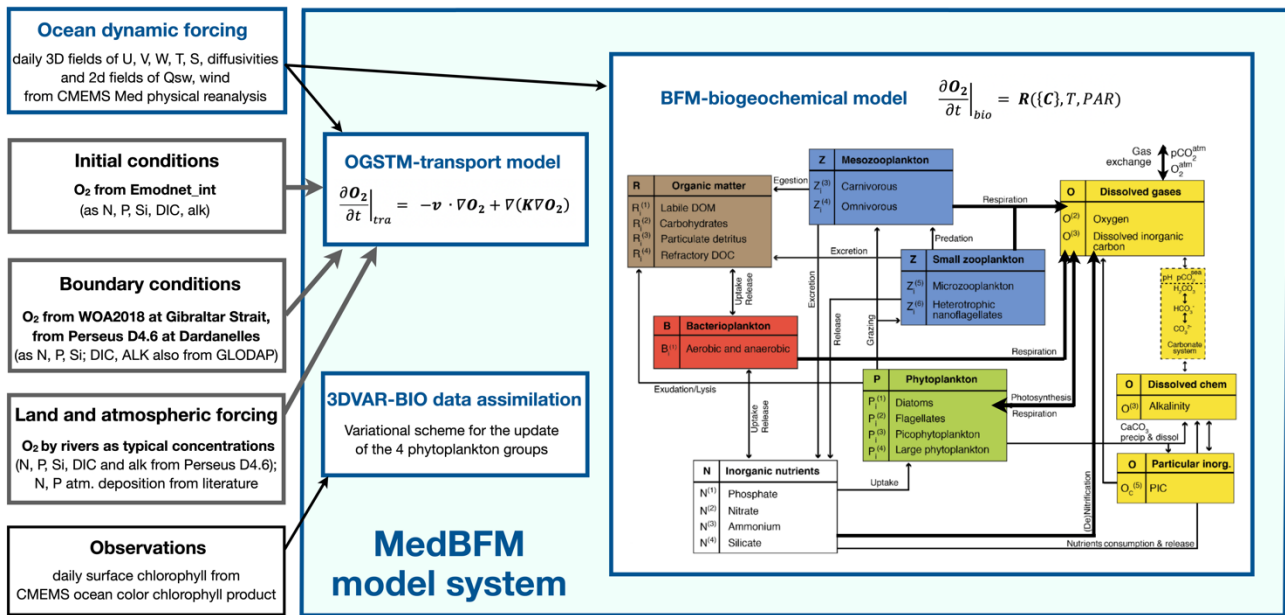
125 Figure 1: MedBFM model system used to simulate oxygen dynamics depicted with its interfaces with other CMEMS system components, where sources/references for modelled oxygen are highlighted in bold. Oxygen as a tracer variable is advected/diffused (OGSTM-transport model), and its concentration varies with other biogeochemical and environmental variables (BFM- biogeochemical model). The main biogeochemical processes that change the oxygen concentration (i.e., photosynthesis, respiration, (de)nitrification, and air-sea fluxes) within BFM components are highlighted by thick arrows. In the figure, i=C,N,P, Si, Chl is for 130 phytoplankton and i=C,N,P for bacteria, zooplankton and organic matter (but i=C,N,P, Si is for R (4) ). References are given in the text, and further details can be found in Cossarini et al. (2021).
