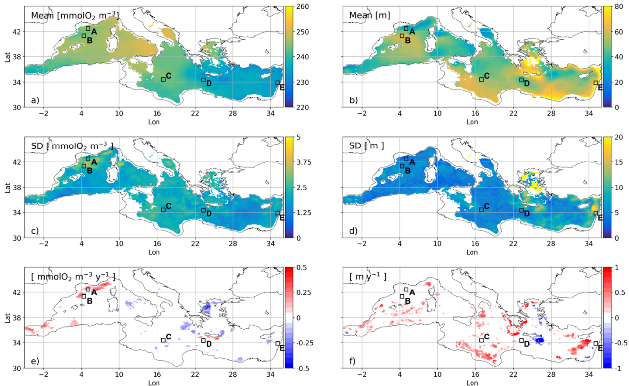
370 Figure 6: Mean concentration (a) and depth (b) for the modelled SOM in summer, computed by averaging the annual maximum vertical values of the mean oxygen concentration in the JAS months and their associated depths, respectively, in the period of 1999- 2019; standard deviation of the annual maximum values (c) and their depths (d), in the same period; trends evaluated in concentration (e) and depth (f) by the Theil-Sen method and provided only if significant as obtained from Mann-Kendall test ( p=0.05 ), in the same period. Areas A-E delimited by black squares are hereafter defined as follows: A = Gulf of Lion, B = Balearic front, C = central Ionian, D = western Cretan gyre, E = eastern Levantine (area). Coastal areas (i.e., with depths shallower than 200 375 m) are masked.
