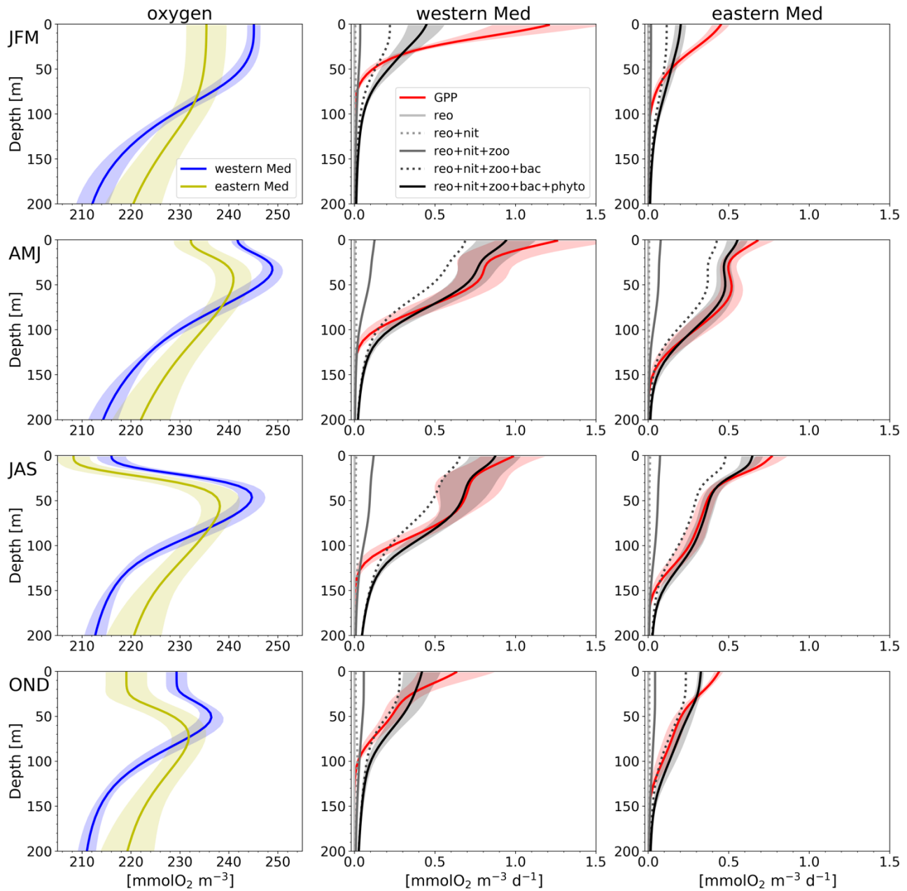
340 Figure 5: Modelled climatological profiles in the epipelagic layer for the oxygen concentration (first column) and daily rate of oxygen concentration associated with biological processes in the western Mediterranean Sea (western Med, second column) and eastern Mediterranean Sea (eastern Med, third column) in the winter (JFM), spring (AMJ), summer (JAS) and fall (OND) seasons, corresponding to the four rows. Biological processes represented are gross primary production (red solid line) and cumulative consumption (alternating solid and dotted lines, in greyscale): reoxidation of reduction equivalents (reo), nitrification (nit) and zooplankton (zoo), bacterioplankton (bac) and phytoplankton (phyto) respiration. Shaded bands represent the spatial variability computed as the standard deviation of the climatological profiles in the western Med and eastern Med. The northern Adriatic Sea was excluded from the computation since its depth is mostly lower than 200 m.
