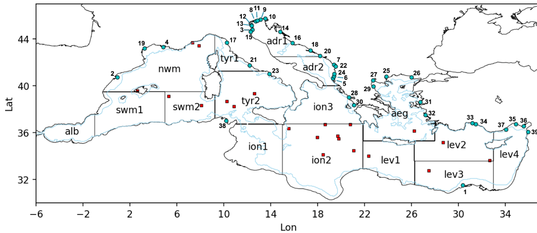
195 Figure 2: Mediterranean Sea domain, with the bathymetric contour at 200 m (light blue line) and cyan dots with numbers corresponding to the main river mouth positions: Nile (1), Ebro (2), Po (3), Rhone (4), Vjosë (5), Seman (6), Buna/Bojana (7), Piave (8), Tagliamento (9), Soca/Isonzo (10), Livenza (11), Brenta-Bacchiglione (12), Adige (13), Lika (14), Reno (15), Krka (16), Arno (17), Nerveta (18), Aude (19), Trebisjnica (20), Tevere (21), Mati (22), Volturno (23), Shkumbini (24), Struma/Strymonas (25), Meric/Evros/Maritsa (26), Axios/Vadar (27), Arachtos (28), Pinios (29), Acheloos (30), Gediz (31), Buyuk Menderes (32), Kopru (33), Manavgat (34), Seyhan (35), Ceyhan (36), Gosku (37), Medjerda (38), Asi/Orontes (39). Subbasins used in the validation procedure are indicated by black contours and acronyms. According to data availability and to ensure the consistency and robustness of the metrics, aggregated subbasins were also used: swm = swm1+swm2; tyr = tyr1+tyr2; adr = adr1+adr2; ion = ion1+ion2+ion3; lev = lev1+lev2+lev3+lev4. Red squares indicate the sampling locations of planktonic metabolism observations. 200
