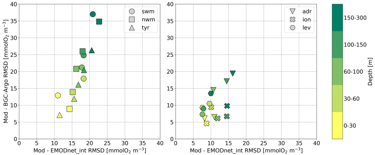
250 Figure 4: Mean RMSD between modelled oxygen outputs and BGC-Argo floats versus mean RMSD of modelled oxygen outputs and the EMODnet_int dataset in open-sea aggregated subbasins in the western (left) and eastern (right) Mediterranean Sea. Metrics are computed for selected layers (0-30 m, 30-60 m, 60-100 m, 100-150 m, and 150-300 m) and averaged over the 1999-2019 time period.
