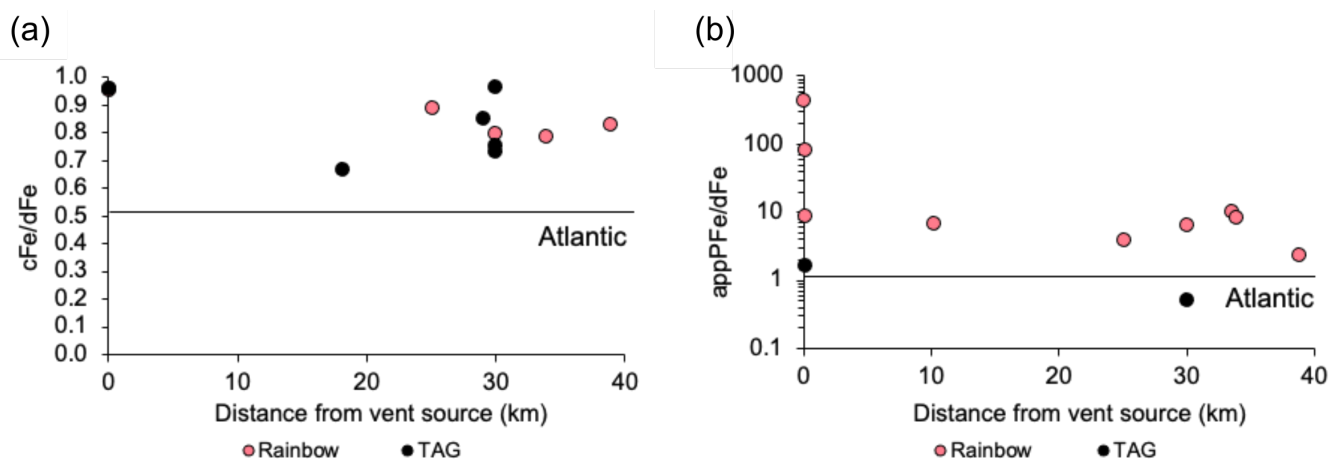
320 Figure 6. (a) Change in integrated cFe/dFe (where cFe = dFe – sFe) and (b) appPFe/dFe of the plume with distance from Rainbow and TAG where appPFe = TDFe – dFe (b). Note the log scale on the y-axis of (b). Solid black lines shows the same ratios for open Atlantic deep waters taken from Milne et al. (2017) for appPFe/dFe and Kunde et al. (2019b) for cFe/dFe.
