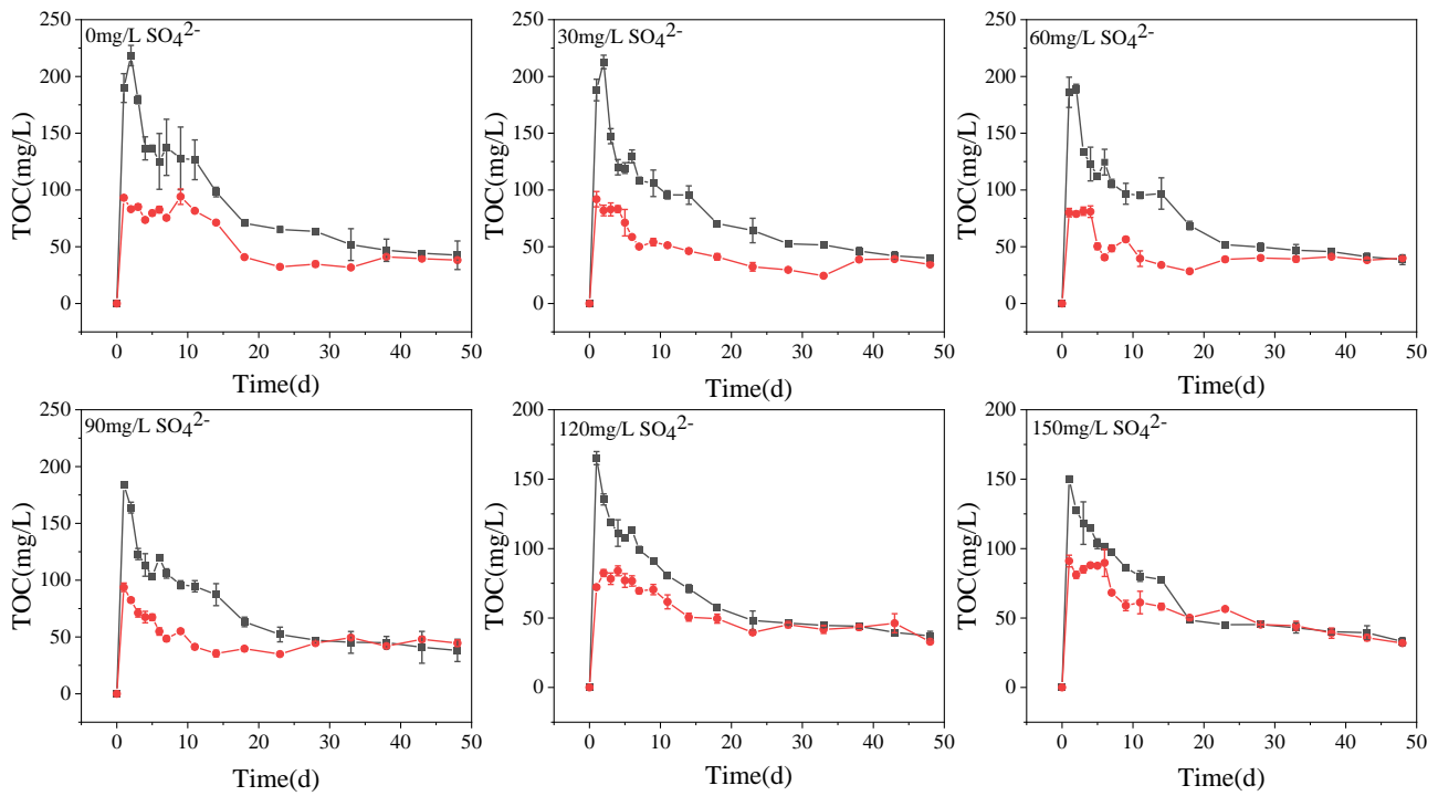
Figure S2. Dynamic change of TOC in the water column during the incubation
