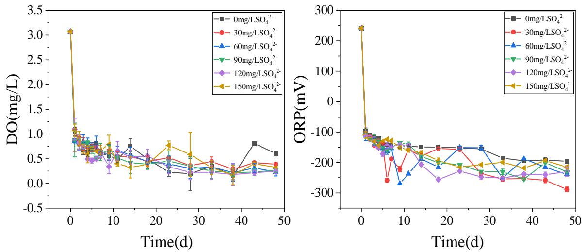
Figure S1. Dynamic change of DO and ORP in the water column during the incubation
