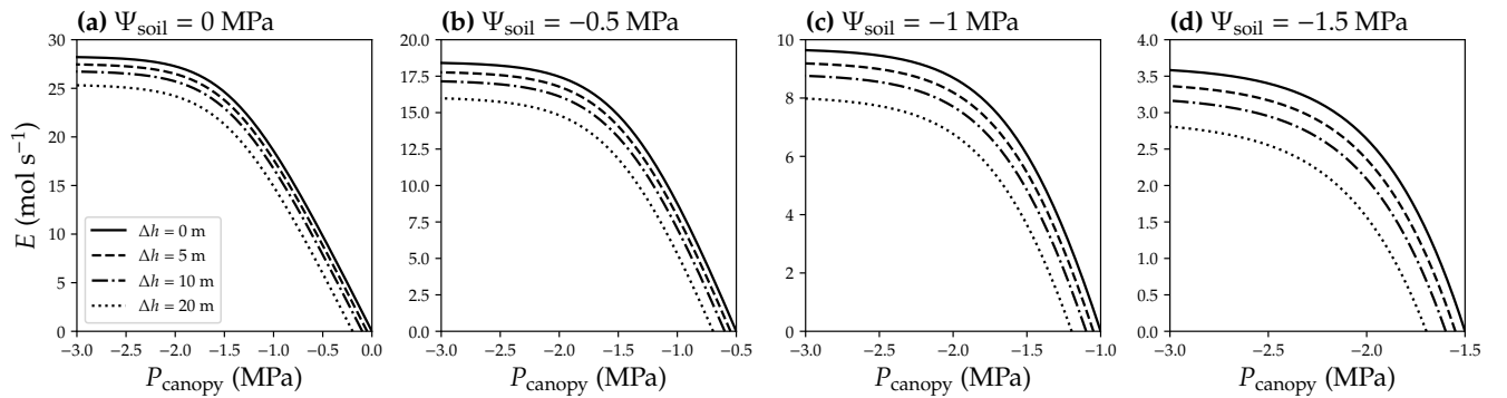
Figure 4. Water supply curve at different \Psi_{\text{soil}} for xylem with different height change. The simulation is done assuming there is no drought legacy effect from previous xylem embolism. See Table 1 for the list of symbols.
