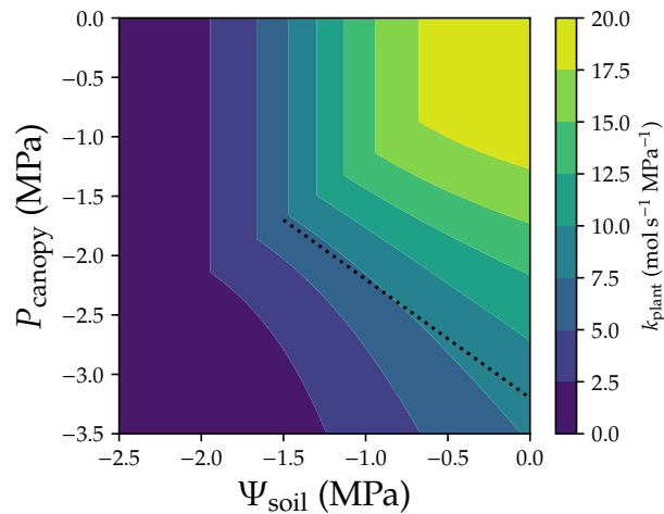
Figure 5. Whole-plant vulnerability surface. Whole-plant hydraulic conductance is computed using k_{\text{plant}} = \frac{E}{\Psi_{\text{soil}} - P_{\text{canopy}} - \rho gh} . The dotted line plots the scenario when mean xylem water pressure is -1.6 MPa. The simulation is done assuming there is no drought legacy effect from previous xylem embolism. See Table 1 for the list of symbols.
