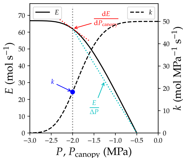
Figure 2. Difference between quantities used in plant hydraulics. The simulation is done for a plant with soil water potential of -0.5 MPa, no gravity term, and no drought legacy effect from previous xylem embolism. See Table 1 for the list of symbols.
