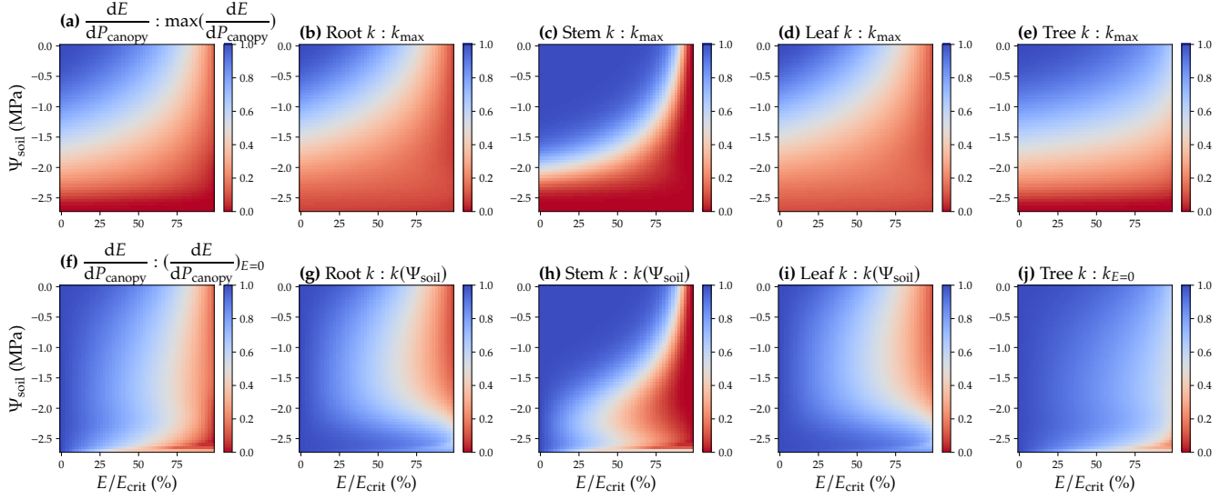
Figure 3. Comparison of different risk measures of stomatal opening. (a)–(e) Values are relative to the maximum when soil water potential is 0 and transpiration rate is 1.0. (f)–(j) Values are relative to the maximum when transpiration rate is 0 at the given soil water potential. The simulation is done assuming there is no drought legacy effect from previous xylem embolism. For the simulation, the plant has a root:stem:leaf resistance ratio of 2:1:1; root and stem height change are 1 and 10 m, respectively; VCs are represented using a Weibull function; Weibull B in MPa and C are 1.879 and 2.396 for root, 2.238 and 9.380 for stem, and 1.897 and 2.203 for leaf (data from Wang et al., 2019). See Table 1 for the list of symbols.
