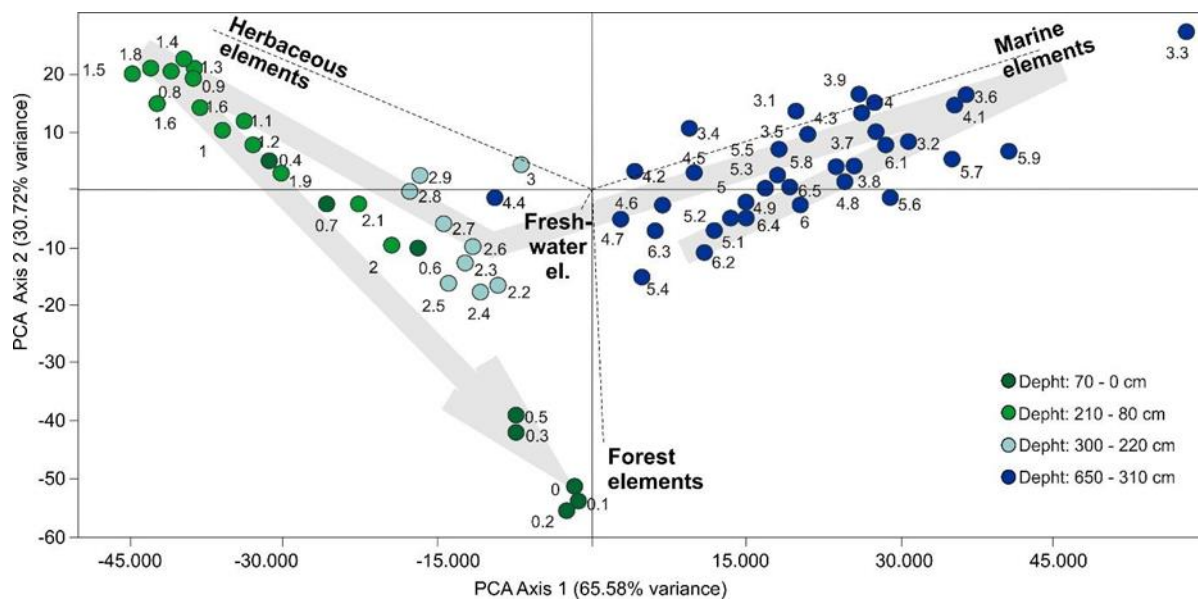
Fig. 9. Biplot of the two main PCA axes with indication of palynomorph groups ordination. Numbers next to the circles indicate the depths of the samples (m).
