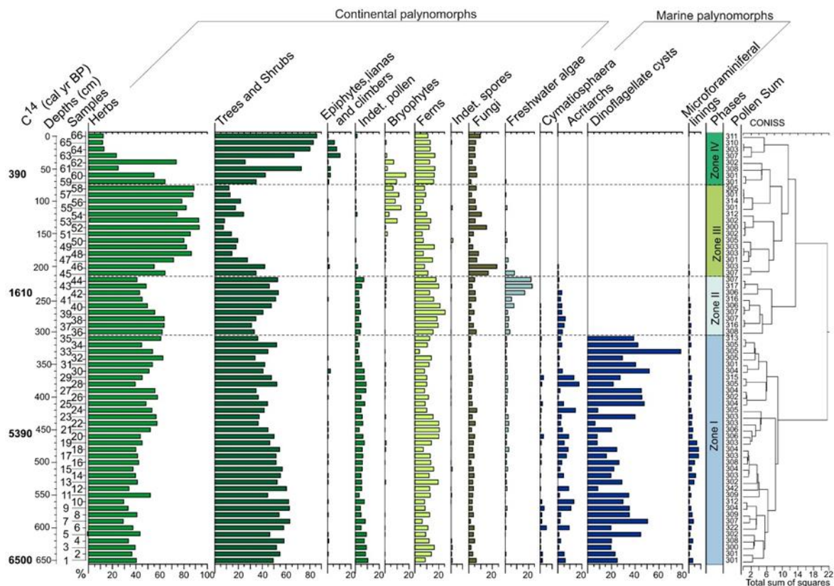
Fig. 5. Percentage diagram of the palynomorphs grouped according to their ecological affinities (habit or habitat) from the PCSC-4 core, south of Santa Catarina Island, southern Brazil, as well as the identified zones and cluster analyses.
