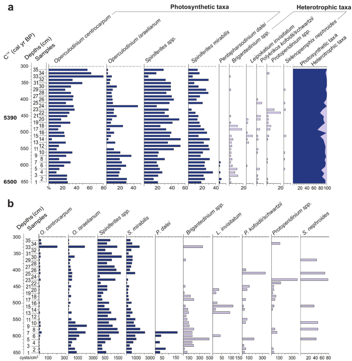
270 Fig. 8. Relative abundance diagram of the dinoflagellate cysts taxa (a) and concentration diagram of the dinoflagellate cysts taxa (b) from the PCSC-4 core, south of Santa Catarina Island, southern Brazil.
