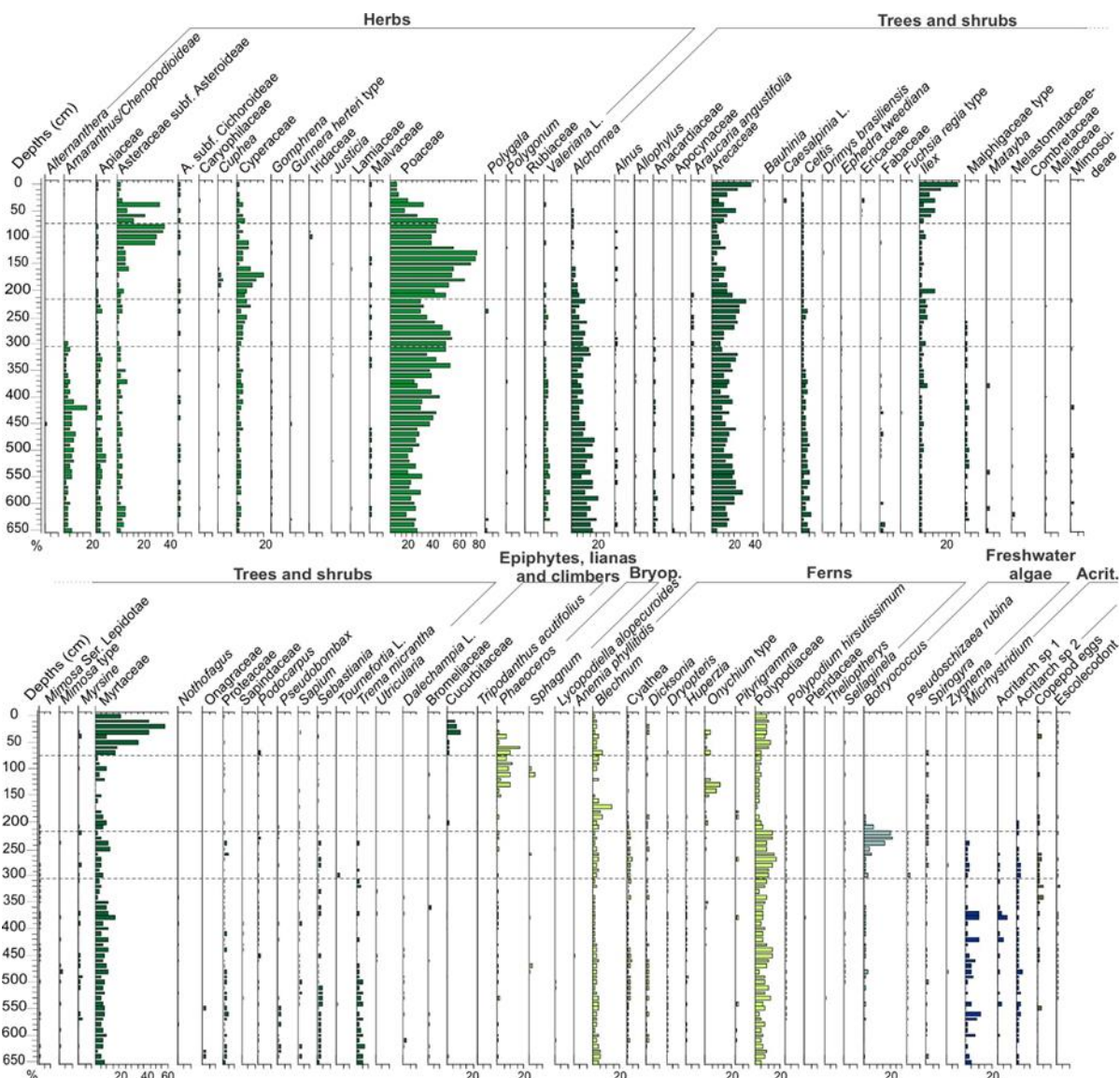
Fig. 7. Relative abundance diagram of the palynomorphs taxa according to their ecological affinities (habit or habitat) from the PCSC-4 core, south of Santa Catarina Island, southern Brazil, as well as the identified zones.
