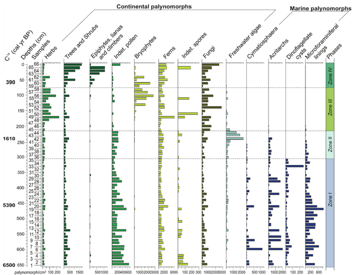
Fig. 6. Concentration diagram of the palynomorphs grouped according to their ecological affinities (habit or habitat) from the PCSC-4 core, south of Santa Catarina Island, southern Brazil, as well as the identified zones.
