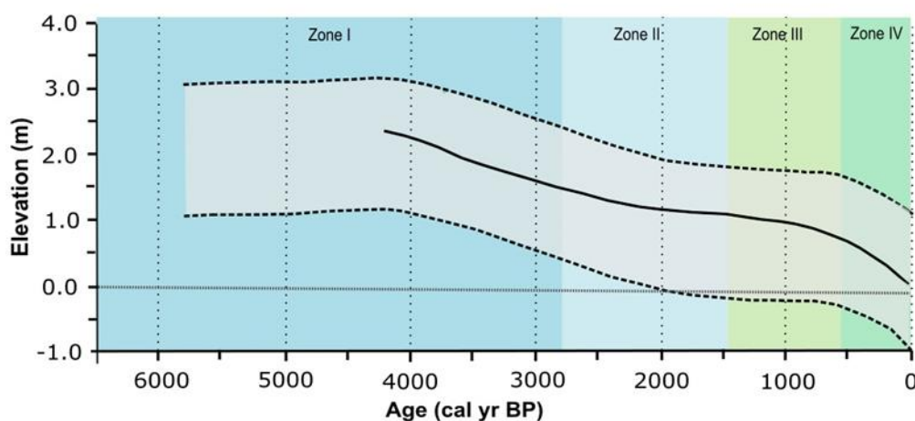
400 Fig. 11. Paleo-sea level reconstructions for the southern Brazilian coast and paleoenvironmental zones. Gray area: relative paleo-sea level envelope (Angulo et al., 2006) to the south of 28°S latitude; Solid line: sea-level model curve for Ponta do Papagaio (Angulo et al., 2022) (modified from Angulo et al., 2022).
