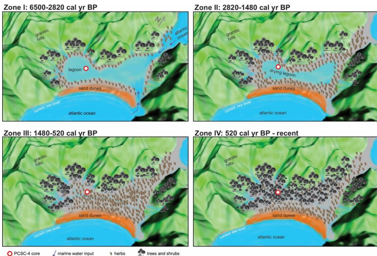
Fig. 10. Schematic model of the environmental evolution of the southernmost portion of the south of Santa Catarina Island (Pântano do Sul), southern Brazil.
