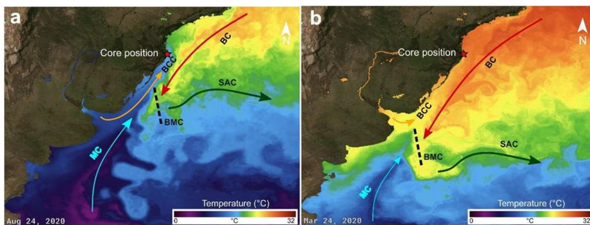
Fig. 2. Present configuration of sea surface currents and temperature in the western South Atlantic Ocean in the (a) winter and (b) summer (JPL MUR MEaSUREs Project, 2015). MC: Malvinas Current; BMC: Brazil-Malvinas Confluence; BC: Brazil Current; BCC: Brazilian Coastal Current; SAC: South Atlantic Current.
