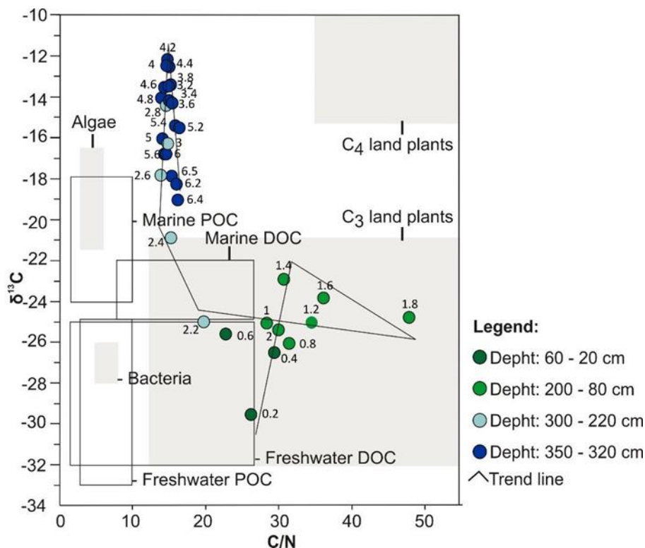
Fig. 4. Binary diagram illustrating the relationship between \delta^{13}\text{C} and C/N (according to Meyers, 1994 and Wilson et al., 2005) and the results obtained from each interval of depth of the PCSC-4 core, south of Santa Catarina Island, southern Brazil. DOC: Dissolved organic carbon; POC: Particulate organic carbon.
