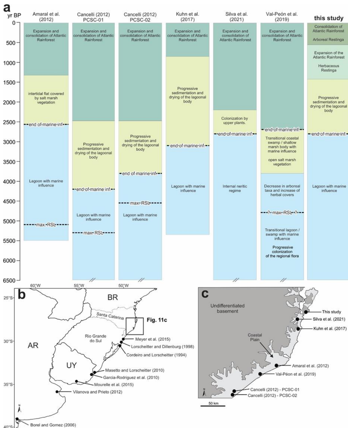
Fig. 12. Palynological studies and their location. (a) Summarized environmental changes of the palynological studies in similar settings of the Santa Catarina coastal plain. (b) Sites from the Rio Grande do Sul State, Uruguay (UY) and Argentina (AR).
