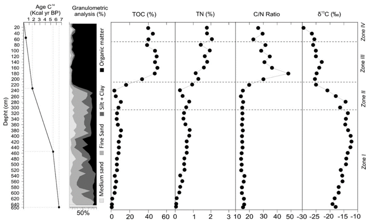
210 Fig. 3. Summarized results of the radiocarbon data, grain-size (granulometric) analyses, total organic carbon (TOC), total nitrogen (TN), C/N ratio and \delta^{13}\text{C} values obtained from the PCSC-4 core, south of Santa Catarina Island, southern Brazil.
