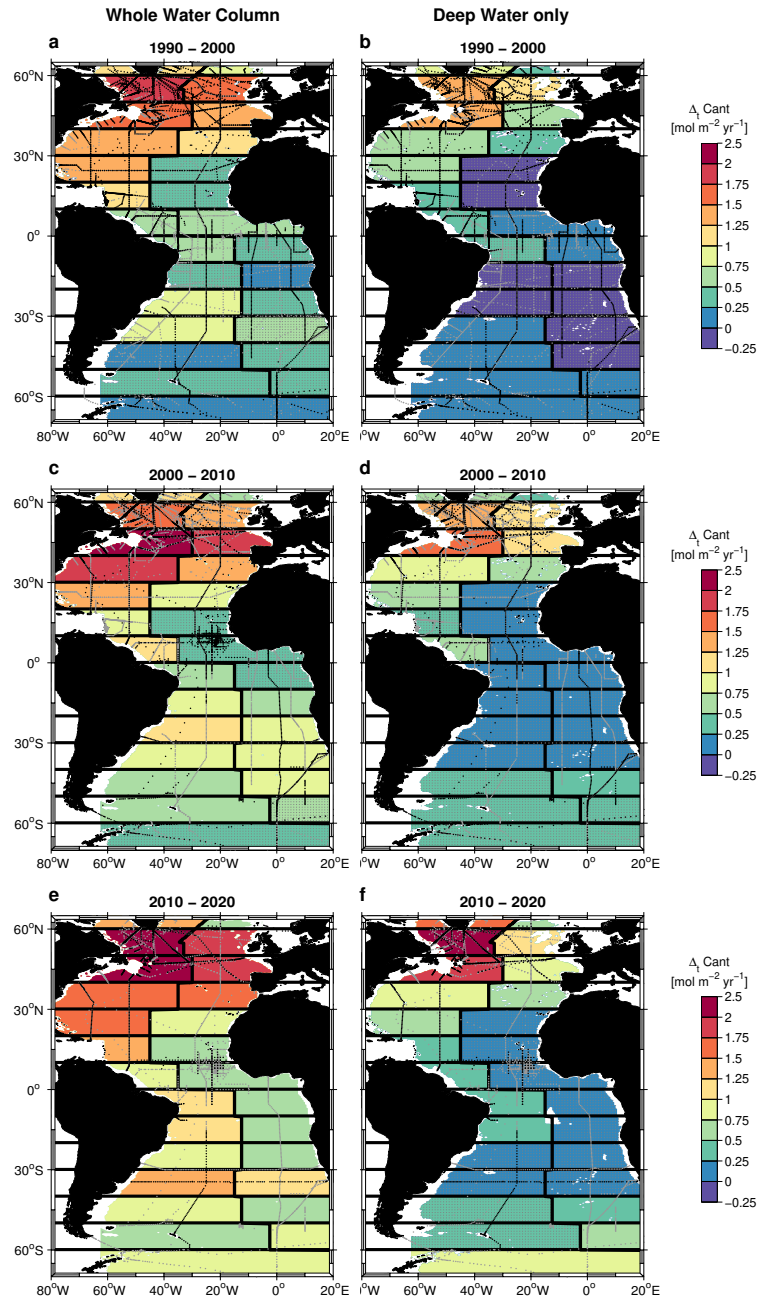
Figure 10. Mean C_{ant} storage rate ( \Delta_t C_{ant} ) for the decades between 1990 and 2020 based on decadal data. Left column: whole water column, right column: only deep and bottom water masses. Top row: 1990–2000, middle: 2000–2010, bottom: 2010–2020. Only areas with a water depth larger than 200 m are considered. Station locations for the first period (1982–1994 in a, b, 1995–2005 in c, d and 2006–2013 in e, f) are marked in light grey, those for the second period (1995–2005 in a, b, 2006–2013 in c, d, 2014–2021 in e, f) in black. Regions with differences smaller than the error range are stippled.
