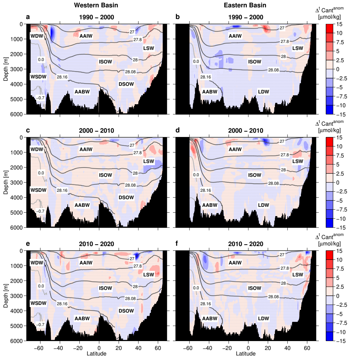
Figure 12. Zonal mean sections of \Delta^t C_{ant}^{anom} ( C_{ant} forecast based on tracer data from the first period minus C_{ant} based on tracer data from the second period). Left column: western basin, right column: eastern basin; top row: 1990–2000, middle: 2000–2010, bottom: 2010–2020. Regions with differences smaller than the error range are stippled. Contour lines are shown as in Fig. 2. Note the uneven spacing between contour intervals.
