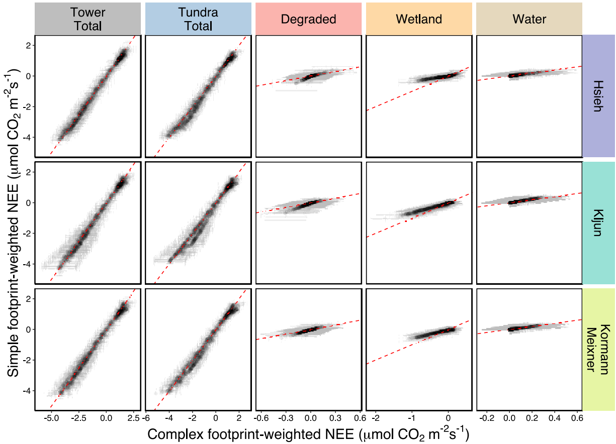
Figure S4. May 2020 median predicted net ecosystem exchange (NEE) for each landcover (simple landcover on the y-axis and complex on the x-axis) weighted by their respective footprint influence. The top row shows NEE predicted with and weighted by footprint influence from Hsieh model, the middle row uses Kljun footprint influence, and the bottom row uses footprint influence from Kormann & Meixner. The leftmost column shows tower total NEE, the linear combination of each predicted NEE weighted by its footprint influence. The next column shows tundra total NEE, the linear combination of lichen tundra, shrub tundra, sedge tundra, and tundra at the edge of degrading permafrost from the complex footprint-weighted NEE on the x-axis, compared to the simple map tundra footprint-weighted NEE on the y-axis. The columns continue with footprint-weighted NEE comparisons for fen, degraded permafrost, and surface water. The error bars show the inter-quartile range on predicted NEE. The dashed red lines indicate the 1:1 line.
