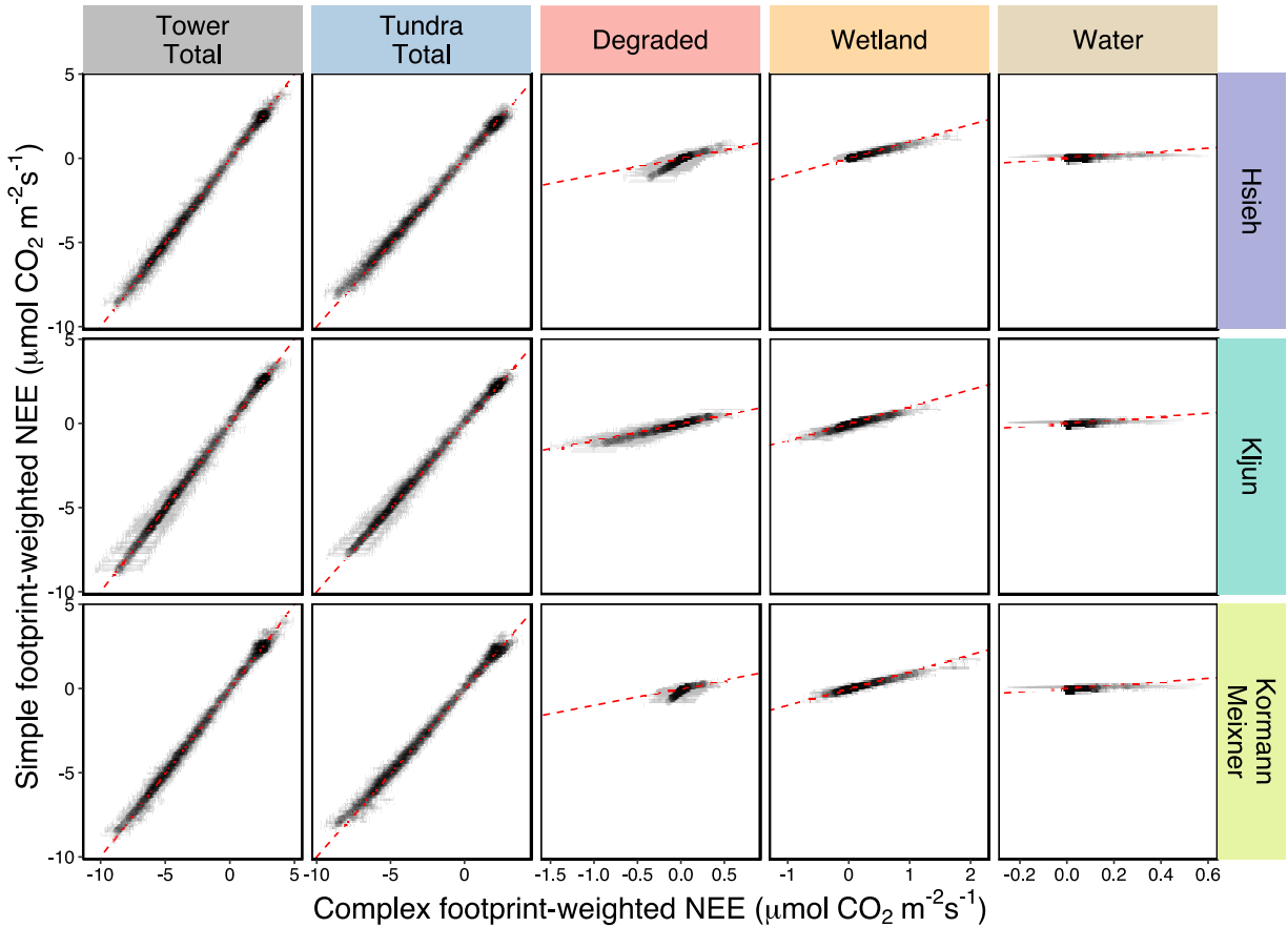
Figure S6. July 2020 median predicted net ecosystem exchange (NEE) for each landcover (simple landcover on the y-axis and complex on the x-axis) weighted by their respective footprint influence. The top row shows NEE predicted with and weighted by footprint influence from Hsieh model, the middle row uses Kljun footprint influence, and the bottom row uses footprint influence from Kormann & Meixner. The leftmost column shows tower total NEE, the linear combination of each predicted NEE weighted by its footprint influence. The next column shows tundra total NEE, the linear combination of lichen tundra, shrub tundra, sedge tundra, and tundra at the edge of degrading permafrost from the complex footprint-weighted NEE on the x-axis, compared to the simple map tundra footprint-weighted NEE on the y-axis. The columns continue with footprint-weighted NEE comparisons for fen, degraded permafrost, and surface water. The error bars show the inter-quartile range on predicted NEE. The dashed red lines indicate the 1:1 line.
