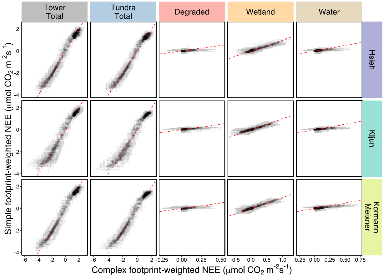
Figure S8. September 2020 median predicted net ecosystem exchange (NEE) for each landcover (simple landcover on the y-axis and complex on the x-axis) weighted by their respective footprint influence. The top row shows NEE predicted with and weighted by footprint influence from Hsieh model, the middle row uses Kljun footprint influence, and the bottom row uses footprint influence from Kormann & Meixner. The leftmost column shows tower total NEE, the linear combination of each predicted NEE weighted by its footprint influence. The next column shows tundra total NEE, the linear combination of lichen tundra, shrub tundra, sedge tundra, and tundra at the edge of degrading permafrost from the complex footprint-weighted NEE on the x-axis, compared to the simple map tundra footprint-weighted NEE on the y-axis. The columns continue with footprint-weighted NEE comparisons for fen, degraded permafrost, and surface water. The error bars show the inter-quartile range on predicted NEE. The dashed red lines indicate the 1:1 line.
