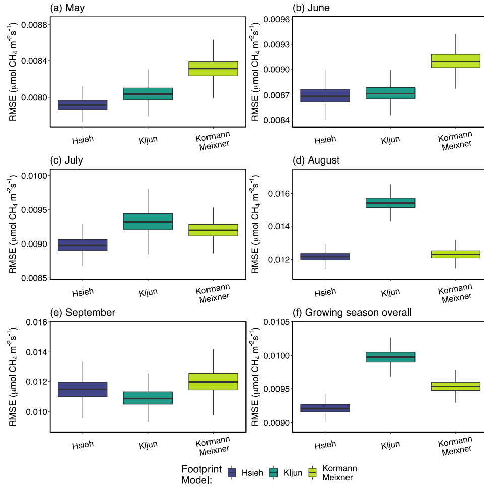
Figure S3. Monthly 2020 (a-e) and growing seasonal 2020 total (f) RMSE from artificial gap-filling CH 4 fluxes. Boxes are the median and interquartile range (IQR), whiskers are 1.5*IQR, for the Bayesian model gap-filling RMSE's.
