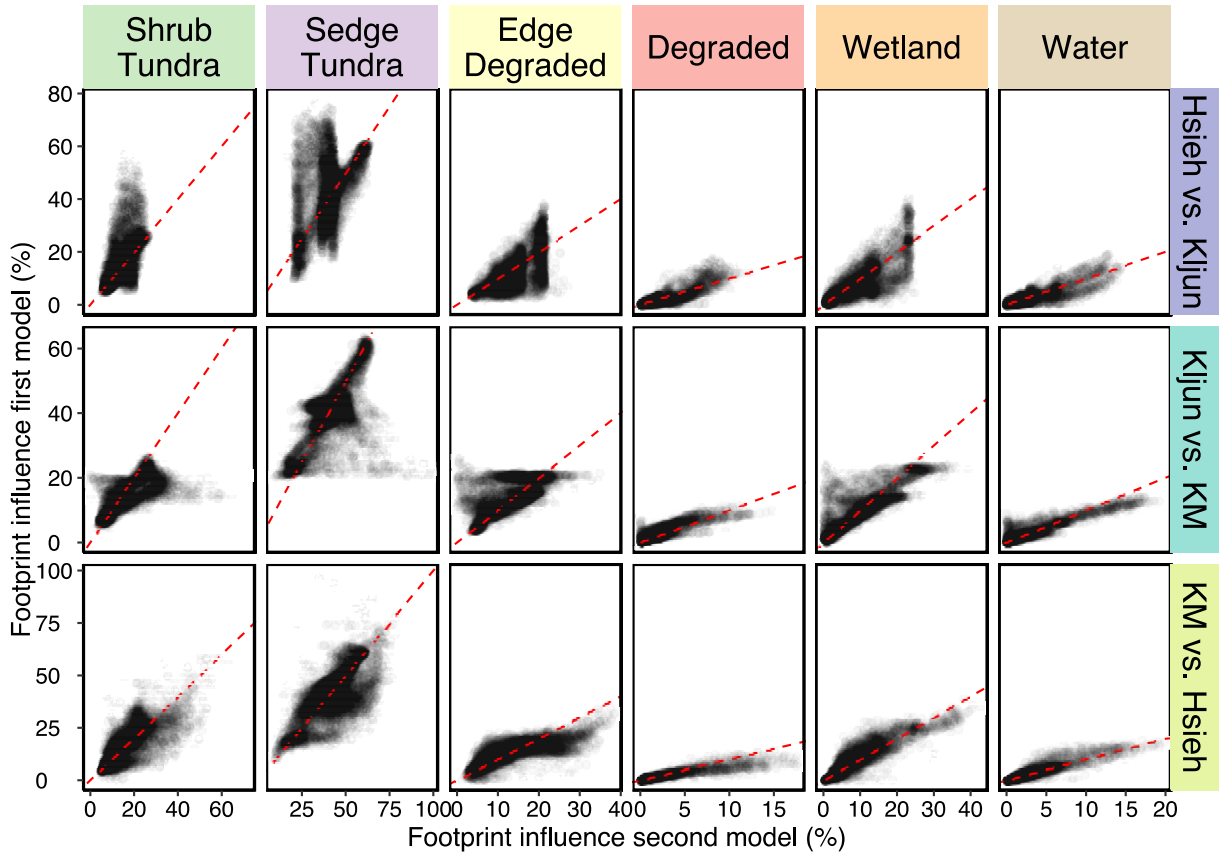
Figure S2. Footprint influences (%) summarized over landcovers for each flux observation. Top row shows Hsieh footprint influence (y-axis) against Kljun footprint influence (x-axis), middle row shows Kljun (y-axis) against Kormann & Meixner (x-axis), and bottom row shows Kormann & Meixner (y-axis) against Hsieh (x-axis). Columns show the summed footprint influence for landcovers from the complex version of the landcover map, which from left to right are; shrub tundra, sedge tundra, edge of degraded permafrost, fen, degraded permafrost, and surface water. Lichen tundra footprint influence comparisons can be found in the main text (Fig 2). The dashed red line indicates the 1:1 line.
