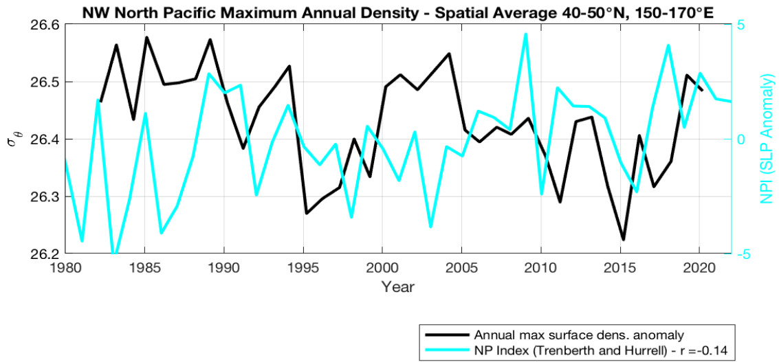
Figure A107. Annual maximum surface density anomaly in northwestern North Pacific (black; from Figure 6b) and annually averaged North Pacific Index (NPI; cyan; Trenberth and Hurrell, 1994 ) in cyan.
