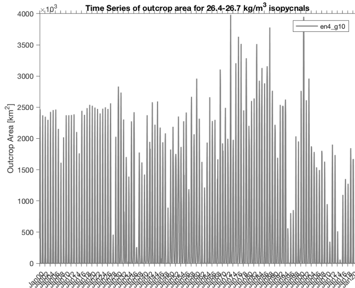
Figure A3. Time series of surface outcrop area of \sigma_{\theta}=26.4-26.7 \text{ kg m}^{-3} in the North Pacific from the 1^{\circ} smoothed EN4 dataset for the full 1900–2020 record. The data since 1982 are the same as shown for EN4 in Figure 2 (red line).
