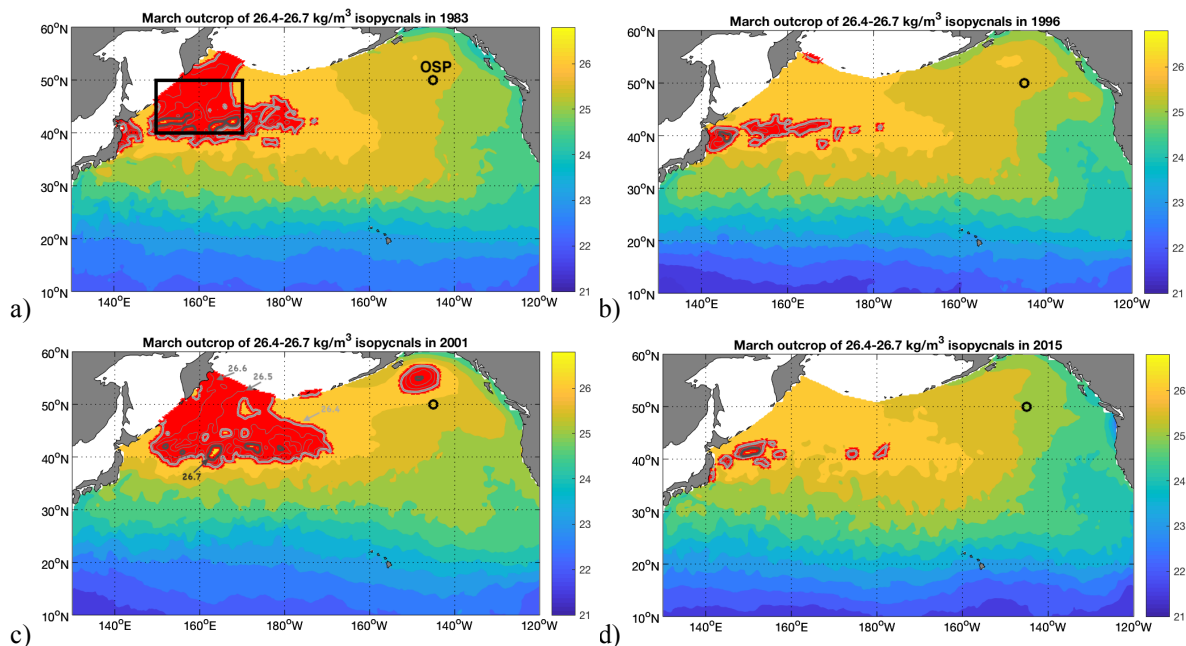
50 Figure 1. Examples of maxima (left) and minima (right) of March outcrop areas of the \sigma_{\theta}=26.4-26.7 \text{ kg m}^{-3} isopycnal range: (a) 1983, (b) 1996, (c) 2001, and (d) 2015. Dataset used is EN4-OISST: \frac{1}{4}^{\circ} degree satellite SST combined with EN4 SSS (interpolated to \frac{1}{4}^{\circ} ). Colored contours and colorbar are surface potential density anomaly, with anomalies in the \sigma_{\theta}=26.4-26.7 \text{ kg m}^{-3} range indicated with red markers (highlighting the outcrop area of those isopycnals). The contour lines, as labeled in (c), show the \sigma_{\theta}=26.4 \text{ kg m}^{-3} (light gray bold line), \sigma_{\theta}=26.5 \text{ kg m}^{-3} and 26.6 \text{ kg m}^{-3} (medium gray thin lines), and \sigma_{\theta}=26.7 \text{ kg m}^{-3} (dark gray bold line) outcrops. The location of OSP at 145°W, 50°N, as labeled in (a), is marked by an open black circle. The area used for northwestern North Pacific SST, SSS, and surface density averaging, as shown in Figures 6, A1, and A5–78–10, is outlined by a black box in (a).
