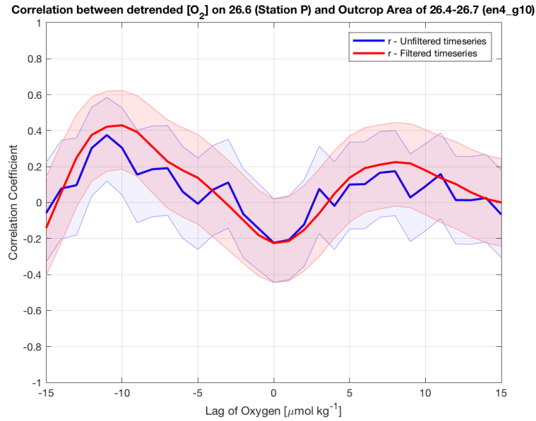
Figure A5. Lagged correlations between detrended timeseries of maximum annual outcrop area of \sigma_0=26.4-26.7 \text{ kg m}^{-3} from EN4 (using the 1941–2020 portion of the full outcrop area timeseries shown in Figure A3) and of \text{O}_2 on \sigma_0=26.6 \text{ kg m}^{-3} at OSP (1956–2020; blue/cyan lines in Figure 4), using unfiltered timeseries data (blue line) and timeseries data filtered with a 5-yr running mean (red line). Details follow Figure 5.
