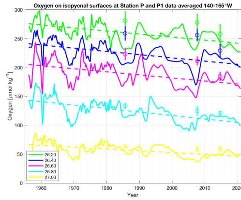
Figure A74. O_2 at OSP on isopycnals from \sigma_\theta=26.2-27.0 \text{ kg m}^{-3} (in 0.2 increments), including linear trends (dashed lines), as in Figure 3, together with averages on the same isopycnals from the WOCE (late 1980s/early 1990s), CLIVAR (2000s), and GO-SHIP (2010s) repeat hydrography cruises, indicated by circles (mean) and vertical lines (standard deviation): (a) using averages between 40-45°N for P16N cruises along 152°W in 1991, 2006, and 2015, and (b) using averages between 140-165°W for P1 cruises in 1987, 2007, and 2014. The latitudinal (P16N) and longitudinal (P1) averaging intervals are shown by the black lines in Figures A63a and A63b, respectively.
