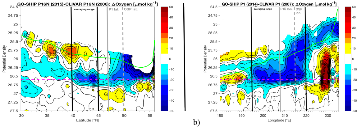
Figure A63. \text{O}_2 differences on potential density surfaces for portions of two North Pacific repeat hydrography sections collected as part of CLIVAR/GO-SHIP: (a) along 152^\circ\text{W} (P16N) – 2015 minus 2006, and (b) along 47^\circ\text{N} (P1) – 2014 minus 2007. The location of the sections relative to OSP is shown in Figure A2. Changes are calculated by objectively mapping the \text{O}_2 data from each repeat occupation to create latitude/longitude versus density grids and differencing the mapped data. The dashed magenta line in each panel marks the \sigma_0=26.6 \text{ kg m}^{-3} isopycnal. The light green lines mark the March mixed layer density along the sections, calculated from climatological data. The latitude and longitude of OSP are marked in panels (a) and (b), respectively, as dashed gray lines, and the latitude and longitude where P16N and P1 cross are marked in panels (a) and (b), respectively, as solid gray lines. The two black solid lines in each panel mark the averaging intervals used for Figure A74. Note that the averaging interval ( 40-45^\circ\text{N} ) in panel (a) ( 40-45^\circ\text{N} ) is somewhat to the south of the OSP latitude because this marks the region of largest \text{O}_2 decline on \sigma_0=26.6 \text{ kg m}^{-3} in the interior away from the mixed layer and matches the averaging interval used in previous work (Mecking et al., 2008).
