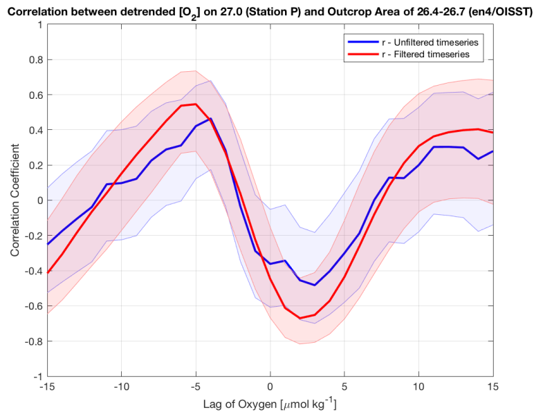
Figure A4. Lagged correlations between detrended timeseries of maximum annual outcrop area of \sigma_{\theta}=26.4-26.7 \text{ kg m}^{-3} (Figure 4) and of \text{O}_2 on \sigma_{\theta}=27.0 \text{ kg m}^{-3} at OSP (solid yellow line in Figure 3a), using unfiltered timeseries data (blue line) and timeseries data filtered with a 5-yr running mean (red line). Details follow Figure 5.
