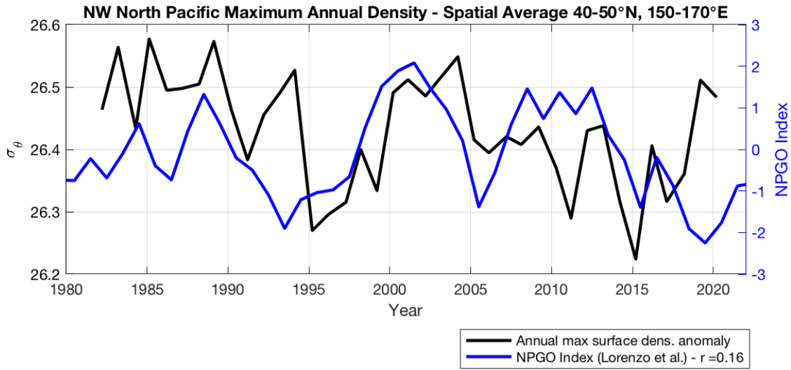
Figure A96. Annual maximum surface density anomaly in northwestern North Pacific (black; from Figure 6b) and annually averaged North Pacific Gyre Oscillation (NPGO; Di Lorenzo et al., 2008 ) index (blue).
