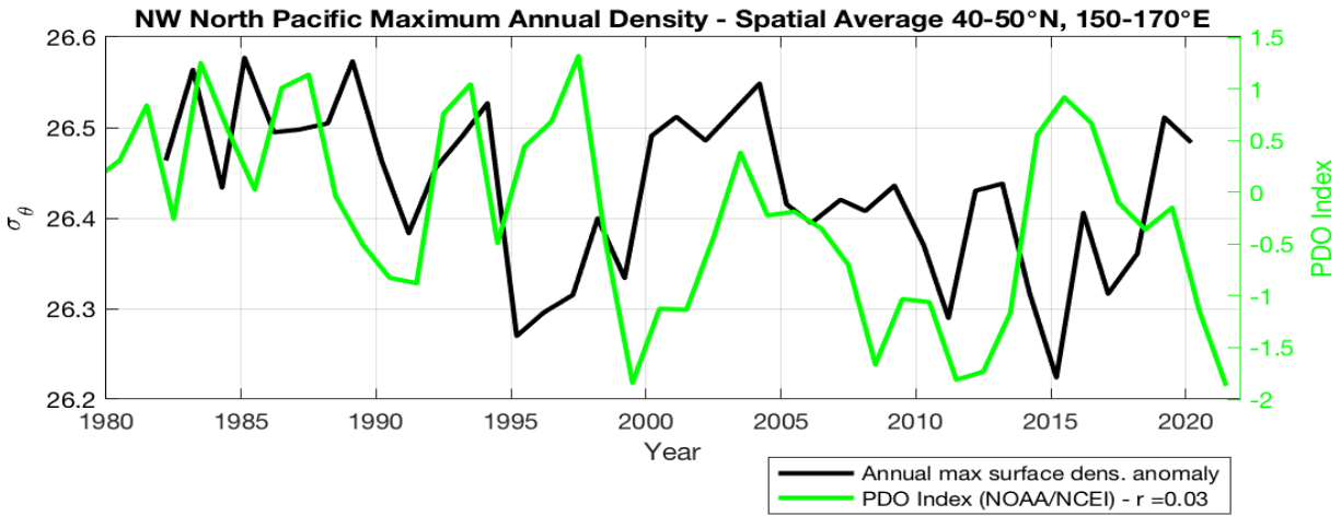
Figure A85. Annual maximum surface density anomaly in northwestern North Pacific (black; from Figure 6b) and annually averaged Pacific Decadal Oscillation (PDO; Mantua et al., 1997 ) index (light green).
