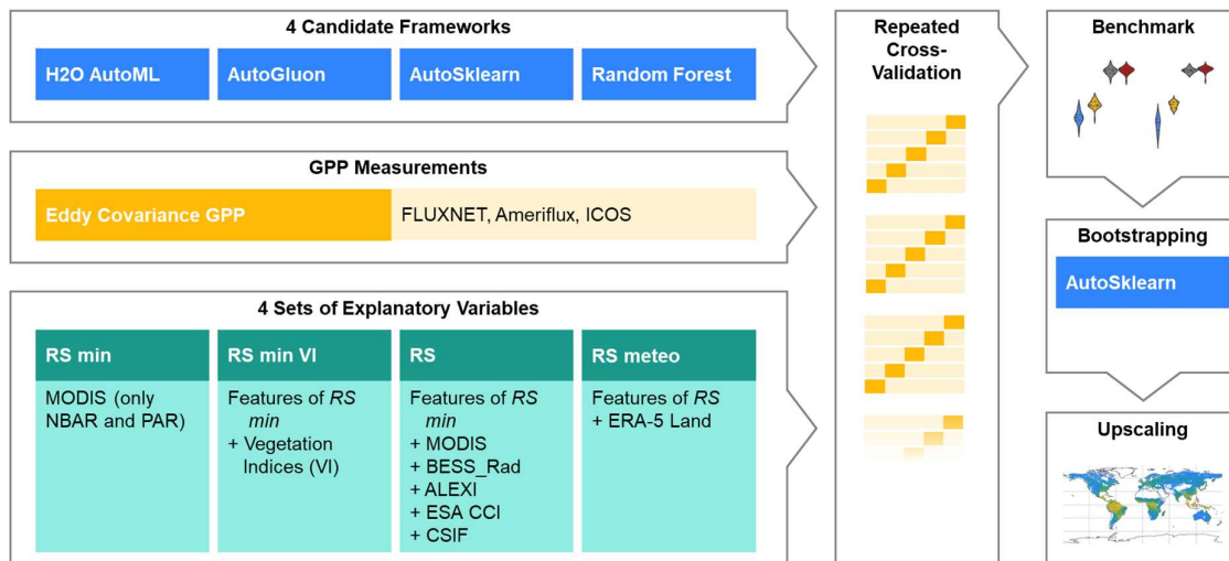
220 Figure 3 Experiment setup. We trained and evaluated AutoSklearn, H2O AutoML, AutoGluon, and Random Forest, together with four sets of explanatory variables in repeated cross-validation on GPP data from eddy covariance measurements. Then, we trained AutoSklearn in a bootstrap aggregation to produce global wall-to-wall GPP maps. The abbreviations of the explanatory variable sets translate as follows: "RS" for remotely sensed, "VI" for vegetation indices, and "meteo" for meteorological data.
