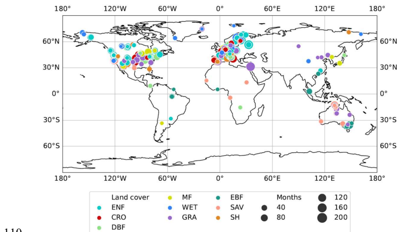
Figure 1: Locations of the measurement sites. The marker size represents the number of monthly measurements available at the respective location. The color stands for the land cover class reported at the site and comprises croplands (CRO), shrublands (SH),
