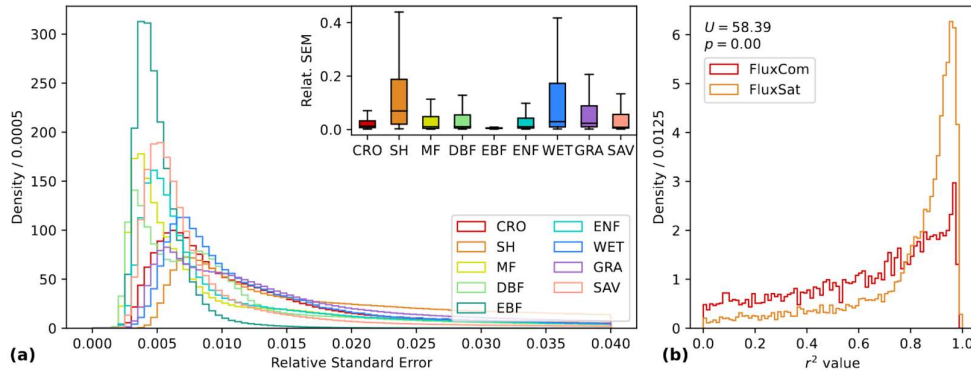
440 Figure 13 Histogram of the relative standard error of the mean (SEM) by land cover class during the entire observation period (a) and distribution of r^2 values for total GPP of the upscaled GPP AutoSklearn product with "RS" variables, compared to the FluxCom v6 and FluxSat datasets (b). For the latter, GPP is sampled at 10000 random locations and compared in a Mann-Whitney U test.
