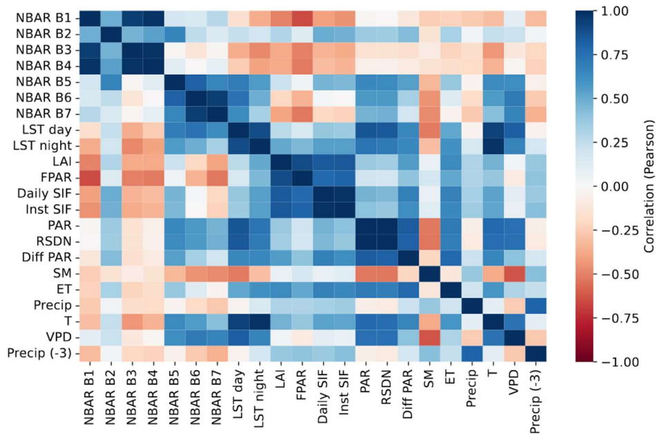
650 Figure A1 Pearson correlation matrix between the scalar explanatory variables, including the MODIS NBAR bands, land surface temperature (LST), leaf area index (LAI), photosynthetically active radiation (PAR), fraction of absorbed PAR (FPAR), diffuse PAR (Diff PAR), daily and instantaneous solar-induced fluorescence (SIF), surface downwelling shortwave flux (RSDN), soil moisture (SM), evapotranspiration (ET), precipitation (Precip), temperature at 2m height (T), vapor pressure deficit (VPD), and precipitation with 3-months lag (Precip (-3)).
