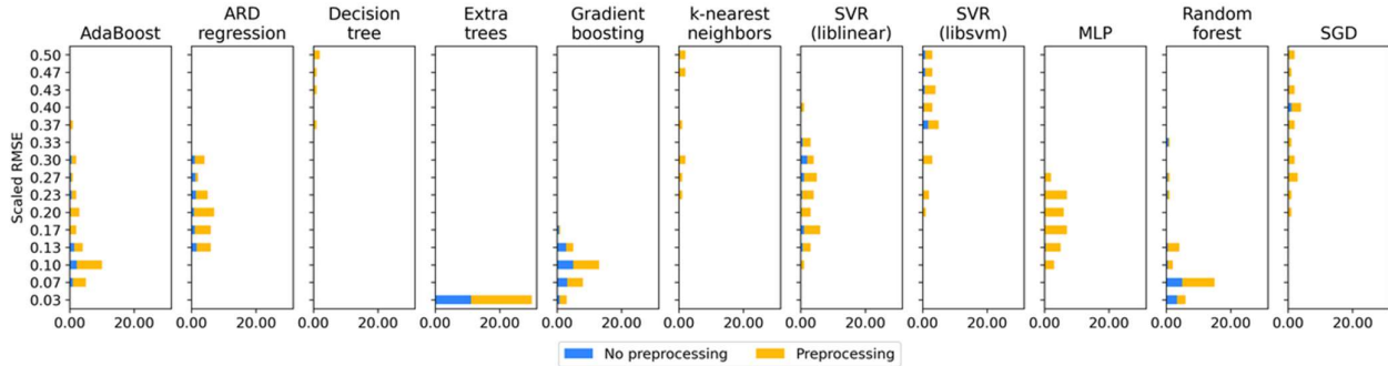
405 Figure 10 Performance of AutoSklearn base models and feature pre-processors. The chart shows the distribution of the mean RMSE for each base model type across all folds within each repetition of the cross-validation. We considered only the best-performing models for each model class within each fold. The RMSE is min-max scaled from zero to one within each cross-validation fold to account for variations in the data's predictability depending on the data's split. The use of preprocessing algorithms is shown as colors in the proportions of their usage in each bin (detailed preprocessing methods in figure A5).
