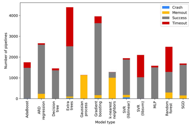
Figure A4 Run statistics of the AutoSklearn base models. The four statuses show how many base models succeeded or failed during training due to insufficient memory, training time, or other unknown reasons. Only the successful models were used for the configuration of AutoSklearn.
