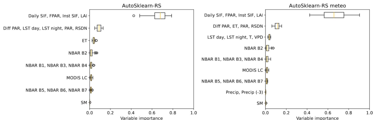
350 Figure 7 Permutation importance for different explanatory variables with the AutoSklearn framework and “RS” and “RS meteo” variable sets. The variables are grouped into clusters of colinear variables regardless of data source or ecological function. The importance is the decrease of r^2 at test time when the variables of the corresponding cluster are randomly shuffled. The variables include the MODIS NBAR bands (red, NIR, blue, green, and 3 SWIR bands), land surface temperature (LST), leaf area index (LAI), photosynthetically active radiation (PAR), fraction of absorbed PAR (FPAR), diffuse PAR (Diff PAR), daily and instantaneous solar-induced fluorescence (SIF), surface downwelling shortwave flux (RSDN), soil moisture (SM), evapotranspiration (ET), 355 precipitation (Precip), temperature at 2m height (T), vapor pressure deficit (VPD), and precipitation with 3-months lag (Precip (-3)).
