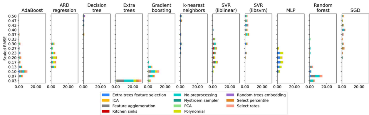
Figure A5 Detailed use of preprocessing algorithms by AutoSklearn. The chart shows the distribution of the mean RMSE for each base model type across all folds within each repetition of the cross-validation. We considered only the best-performing models for each model class within each fold. The RMSE is min-max scaled from zero to one within each cross-validation fold to account for variations in the data's predictability depending on the data's split. The use of preprocessing algorithms is shown as colors in the proportions of their usage in each bin.
