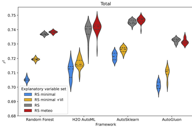
Figure 4: Overall framework performance, given in the coefficient of determination r^2 for the candidate frameworks and the four different explanatory variable sets. Each distribution results from the repeated CV and belongs to one framework and one explanatory variable set.
