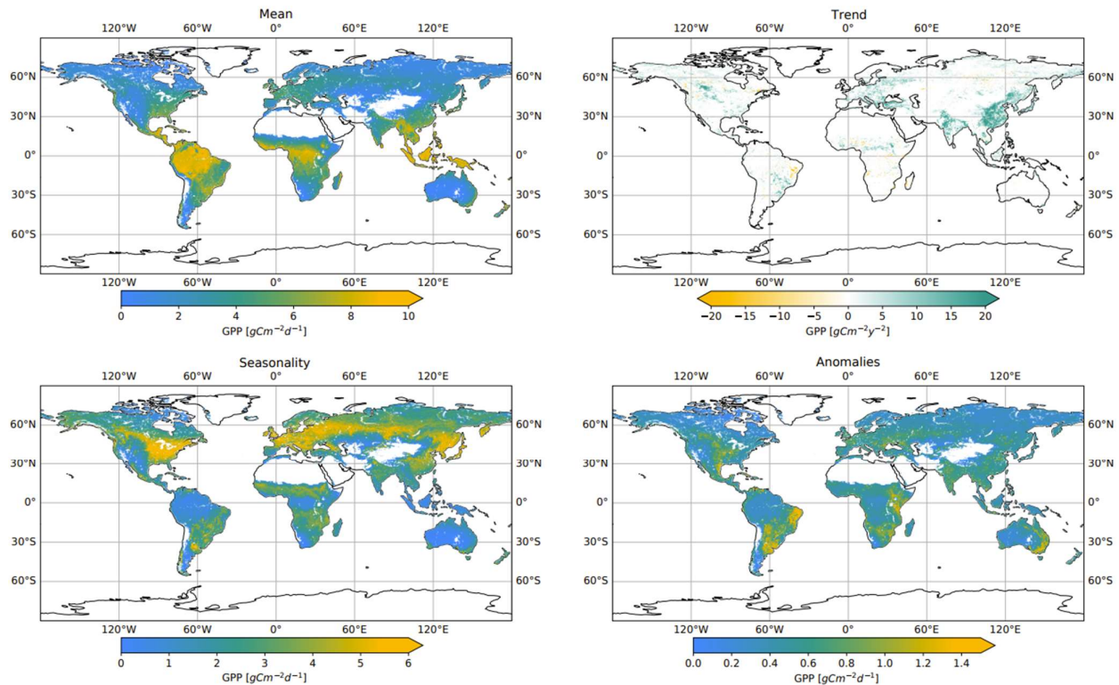
415 Figure 11 Total GPP, amplitude of seasonality, trend, and anomalies of prediction with AutoSklearn trained on remotely sensed data ("RS" dataset) in a bootstrap aggregation of 30 bootstraps. The mean was calculated at each location over all bootstrapped predictions and the entire time series. The seasonality is displayed as the amplitude of the month-wise average. Trends were calculated as the slope from an ordinary least squares linear regression over time and masked so that only significant trends were included ( p < 0.05 ). The anomalies are shown as the standard deviation of the residuals after subtracting the seasonal and trend components from the time series.
