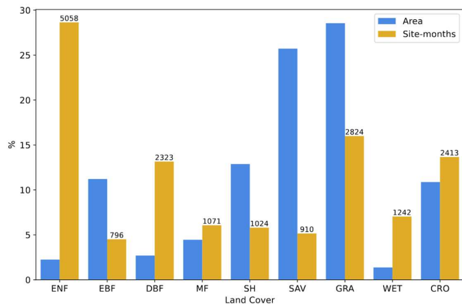
Figure 2: Standardized number of sites-months and global area of each land cover type, excluding land covers without any GPP measurements. The number of sites-months is shown above their respective columns. The land cover classes reported follow the IGBP classification (International Geosphere–Biosphere Programme, 2024) and comprise croplands (CRO), shrublands (SH), deciduous broadleaf forests (DBF), evergreen broadleaf forests (EBF), evergreen needleleaf forests (ENF), grasslands (GRA), mixed forests (MF), savannas (SAV), and permanent wetlands (WET).
