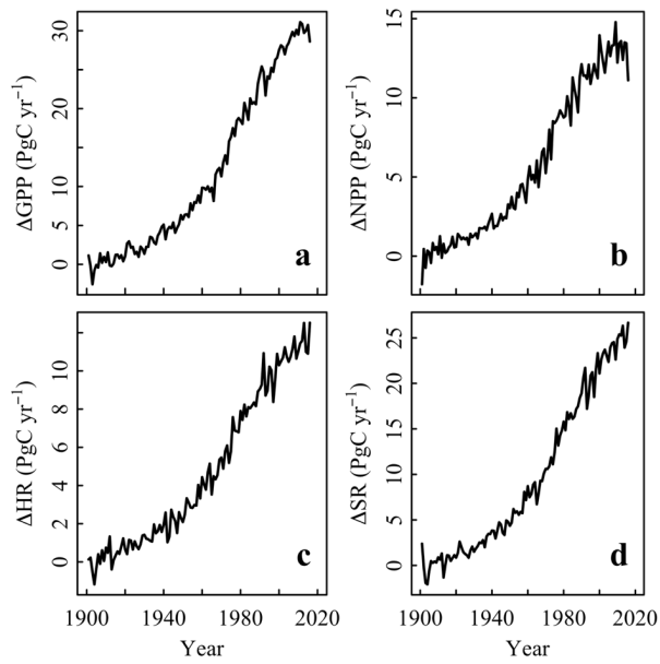
1415 Fig. 5. Evolution of annual carbon flux of area-weighted (a) GPP, (b) NPP, (c) HR, and (d) SR simulated by the CLM-Microbe model since 1901. The baseline was the ten-year average of corresponding variables during 1901-1910. GPP: gross primary productivity; NPP: net primary productivity; HR: heterotrophic respiration; SR: soil respiration.
