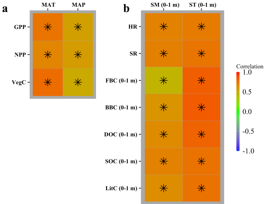
1465 Fig. 14. Heatmap showing Pearson's correlation between the CLM-Microbe model simulated (a) GPP, NPP, and VegC and 1470 MAT and MAP and (b) HR, SR, FBC in the top 1 m, BBC in the top 1 m, DOC in the top 1 m, SOC in the top 1 m, and LitC in the top 1 m and SM and ST in the top 1 m from 1901 to 2016. GPP: gross primary productivity; NPP: net primary productivity; HR: heterotrophic respiration; SR: soil respiration; DOC: dissolved organic carbon; SOC: soil organic carbon; FBC: fungal biomass carbon; BBC: bacterial biomass carbon; VegC: vegetation carbon; LitC: litter carbon; MAT: mean annual temperature; MAP: mean annual precipitation; ST: soil temperature; SM: soil moisture. Black asterisks indicate significant correlations ( P < 0.05 ).
