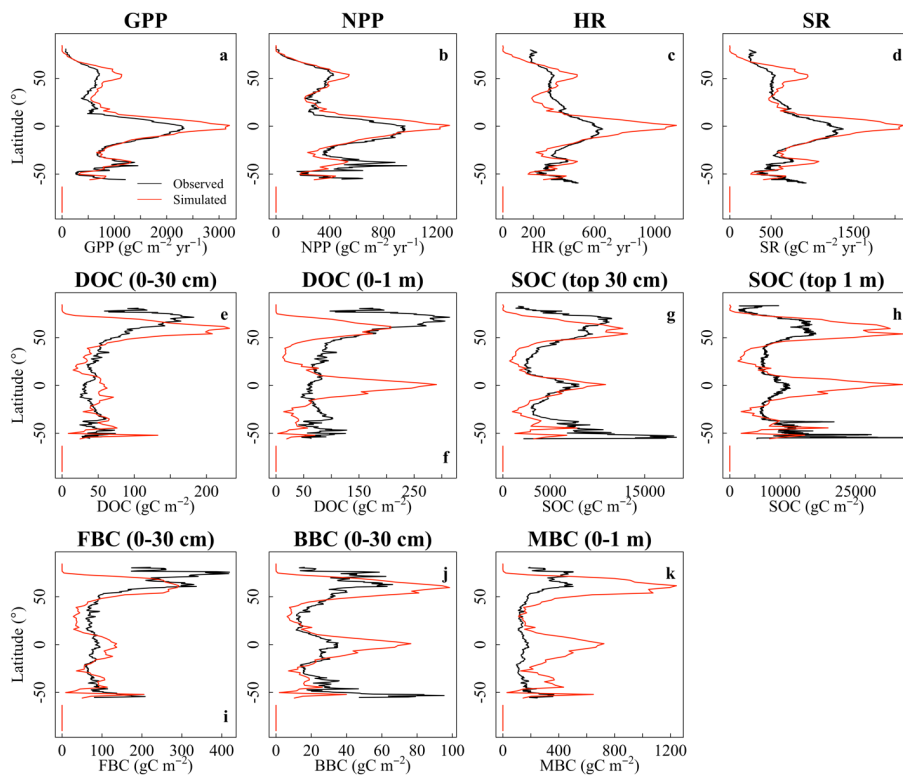
1390 Fig. 1. Latitudinal comparison between observed (black line) and the CLM-Microbe-simulated (red line) (a) GPP, (b) NPP, (c) 1395 HR, (d) SR, (e) DOC in the top 30 cm, (f) DOC in the top 1 m, (g) SOC in the top 30 cm, (h) SOC in the top 1 m, (i) FBC in the top 30 cm, (j) BBC in the top 30 cm, and (k) MBC (0-1 m). GPP: gross primary productivity; NPP: net primary productivity; HR: heterotrophic respiration; SR: soil respiration; DOC: dissolved organic carbon; SOC: soil organic carbon; FBC: fungal biomass carbon; BBC: bacterial biomass carbon; MBC: microbial biomass carbon.
