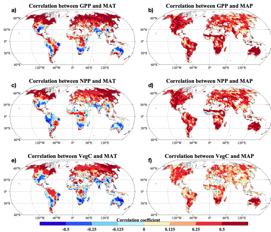
1475 Fig. 15. Pearson's correlation between the CLM-Microbe model simulated (a-b) GPP, (c-d) NPP, and (e-f) VegC and (a, c, and e) MAT and (b, d, and f) MAP from 1901 to 2016. GPP: gross primary productivity; NPP: net primary productivity; VegC: vegetation carbon; MAT: mean annual temperature; MAP: mean annual precipitation. Black dot in each grid indicates significant correlation ( P < 0.05 ).
