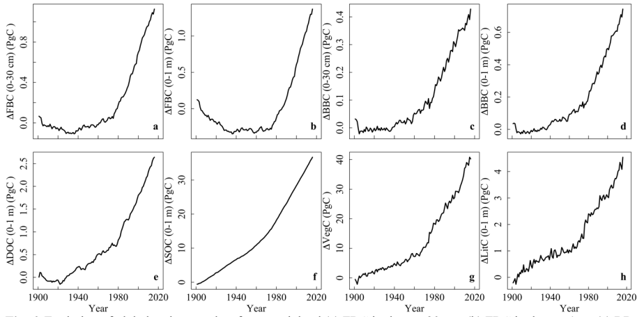
1420 Fig. 6. Evolution of global carbon stocks of area-weighted (a) FBC in the top 30 cm, (b) FBC in the top 1 m, (c) BBC in the top 30 cm, (d) BBC in the top 1 m, (e) DOC in the top 1 m, (f) SOC in the top 1 m, and (g) VegC, and (h) LitC in the top 1 m simulated by the CLM-Microbe model since 1901. The baseline was the ten-year average of corresponding variables during 1901-1910. DOC: dissolved organic carbon; SOC: soil organic carbon; FBC: fungal biomass carbon; BBC: bacterial biomass carbon; MBC: microbial biomass carbon; VegC: vegetation carbon; LitC: litter carbon.
