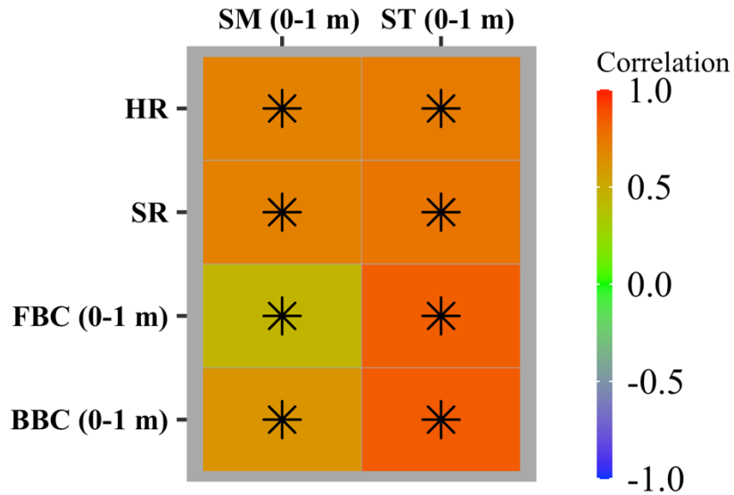
Fig. 8. Heatmap showing Pearson's correlation between the CLM-Microbe model simulated (a) GPP, NPP, and VegC and MAT and MAP and (b) HR, SR, FBC in the top 1 m, BBC in the top 1 1 m, DOC in the top 1 m, SOC in the top 1 m, and LitC in the top 1 m and SM and ST in the top 1 m from 1901 to 2016. GPP: gross primary productivity; NPP: net primary productivity; HR: heterotrophic respiration; SR: soil respiration; DOC: dissolved organic carbon; SOC: soil organic carbon; FBC: fungal biomass carbon; BBC: bacterial biomass carbon; VegC: vegetation carbon; LitC: litter carbon; MAT: mean annual temperature; MAP: mean annual precipitation; ST: soil temperature; SM: soil moisture. Black asterisks indicate significant correlations ( P < 0.05 ).
