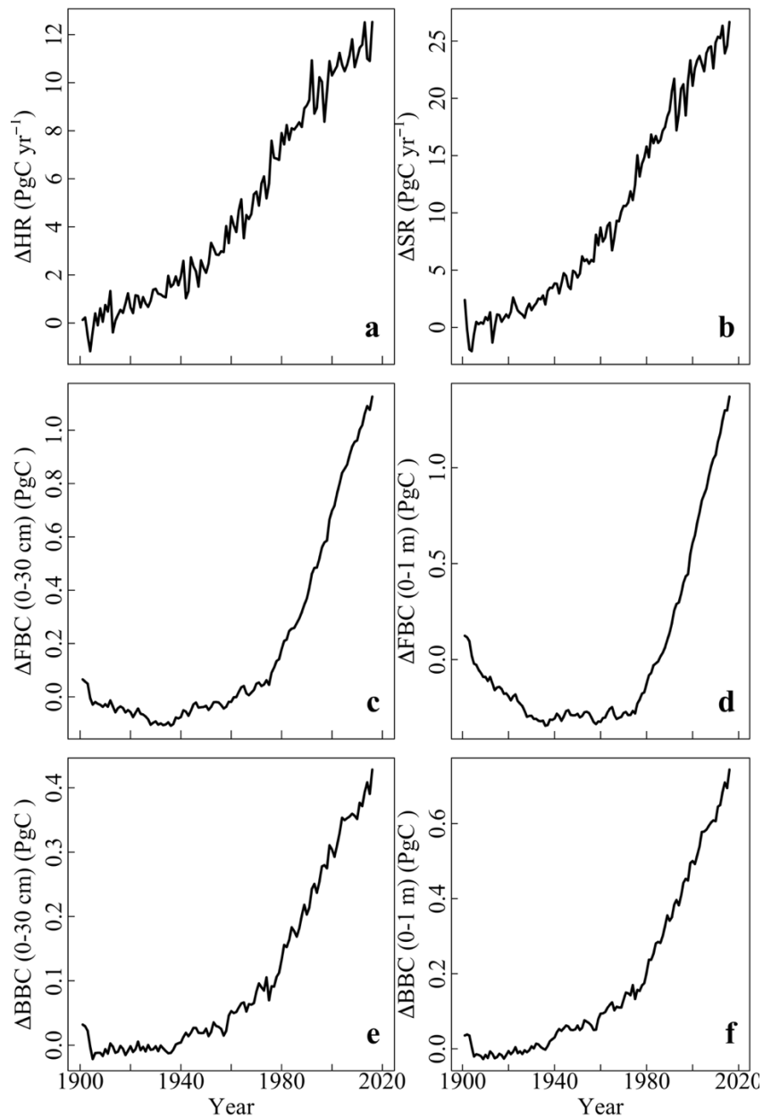
930 Fig. 3. Evolution of annual carbon flux of area-weighted (a) HR and (b) SR and carbon stock of (c) FBC in the top 30 cm, (d) FBC in the top 1 m, (e) BBC in the top 30 cm, and (f) BBC in the top 1 m simulated by the CLM-Microbe model since 1901. The baseline was the ten-year average of corresponding variables during 1901-1910. HR: heterotrophic respiration; SR: soil respiration; FBC: fungal biomass carbon; BBC: bacterial biomass carbon; MBC: microbial biomass carbon.
