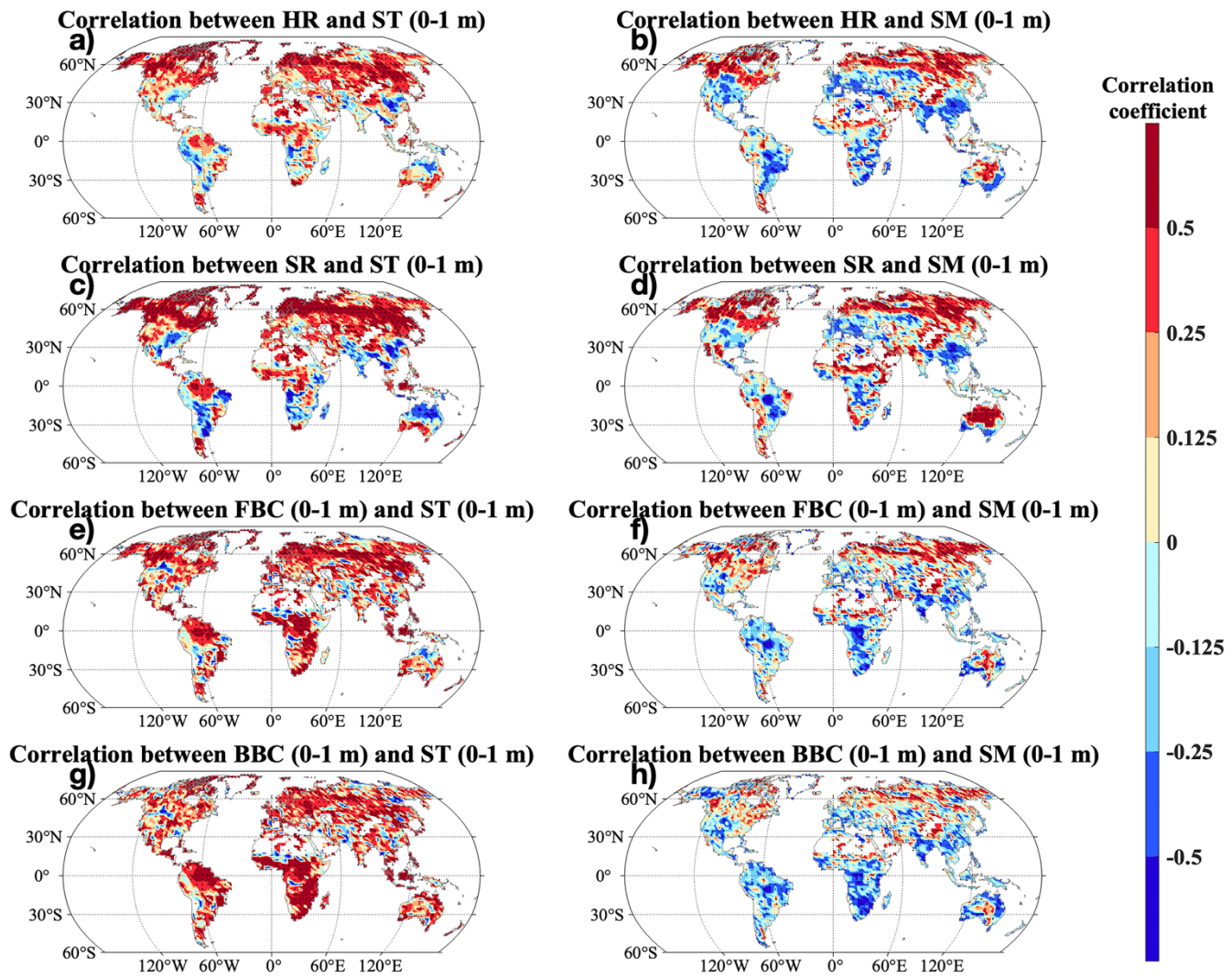
970 Fig. 9. Pearson's correlation between the CLM-Microbe model simulated (a-b) HR, (c-d) SR, (e-f) FBC in the top 1 m, and (g-h) BBC in the top 1 m (a, c, e, and g) ST and (b, d, f, and h) SM in the top 1 m from 1901 to 2016. Black dot in each grid indicates significant correlation ( P < 0.05 ). HR: heterotrophic respiration; SR: soil respiration; FBC: fungal biomass carbon; BBC: bacterial biomass carbon; ST: soil temperature; SM: soil moisture.
