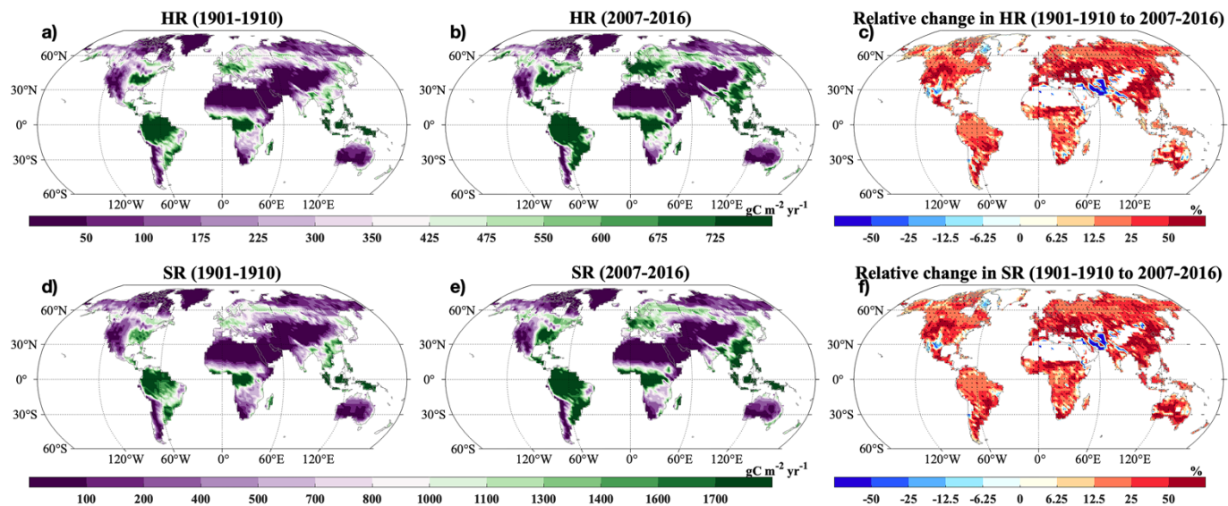
Fig. 5. Spatial distributions of decadal averages of (a-b) HR and (d-e) SR during (a and d) 1901-1910 and (b and e) 2007-2016 and relative changes in (c) HR and (f) SR by 2007-2016 relative to 1901-1910. HR: heterotrophic respiration; SR: soil respiration. Black dot in each grid indicates significant changes ( P < 0.05 ).
