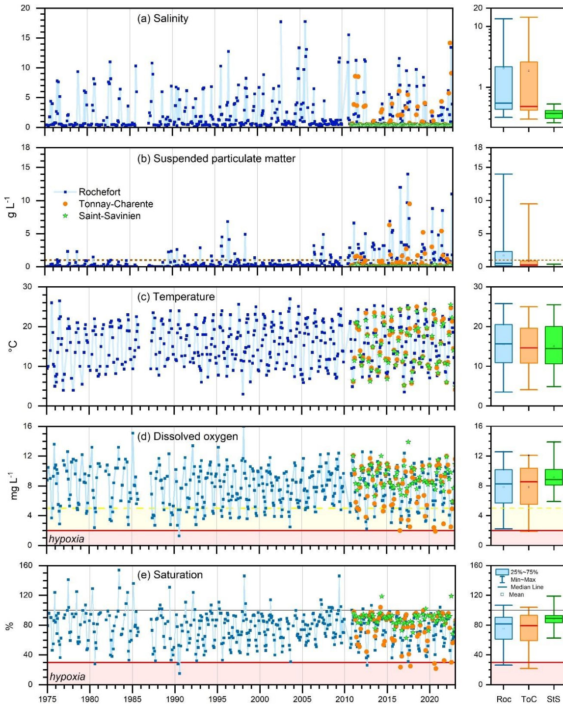
Figure 2: Low frequency records of salinity(a), suspended particulate matter (b), temperature (c) and dissolved oxygen concentration (d) and saturation (e) in surface waters (0.5 m) at Rochefort for the period 1975-2022 and at Tonny-Charente and Saint-Savinien for the period 2011-2022. The panel on the right shows the box plot (min, max, median, mean, 25%-75%) of each parameter per station (Roc: Rochefort; ToC: Tonny-Charente; StS: Saint-Savinien) for the period 2011-2022. The dashed line in Fig. 2b shows the SPM threshold of the TMZ (SPM > 1 g L -1 ). The dashed and bold lines in Fig. 2d show the DO threshold of 5 and 2 (hypoxia) mg L -1 , respectively. The thin and bold lines in Fig. 2e show the saturation threshold of 100 and 30 (hypoxia) %, respectively.
