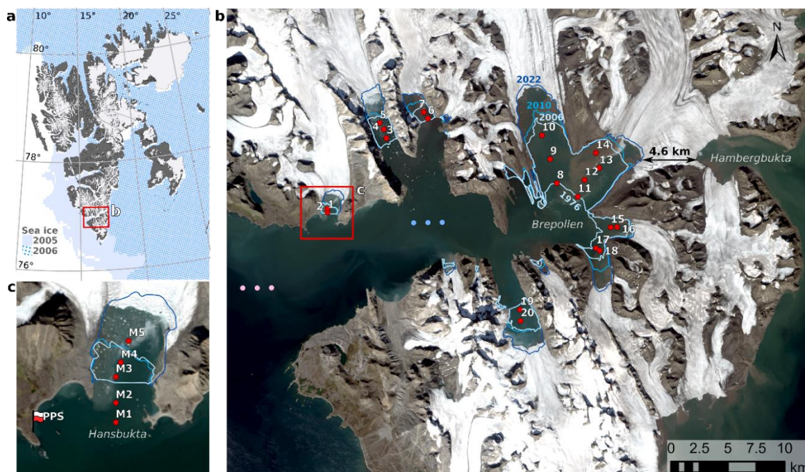
Figure 1: a) Svalbard archipelago with monthly mean sea-ice extent (SIC > 15%) in March 2005 (plain colour) and 2006 (dotted). Land and glaciers extent downloaded from https://geodata.npolar.no/ . The red frame indicates the location of Hornsund. b) Newly-ice-free areas in Hornsund which have opened since 1976 (blue lines – glaciers' front position in 1976, 2006, 2010, and 2022) with
