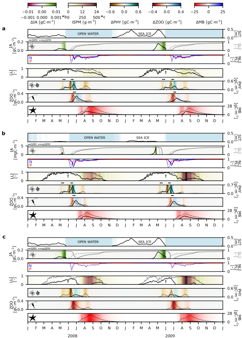
Figure 6: Changes in ecosystem dynamics due to iSPM input in 2008 and 2009 at three modelled stations: a – low iSPM influence (station 9), b – medium iSPM influence (station 2), c – high iSPM influence (station 14). Line plots show sea ice thickness (SIT, m), the biomass of ice algae (IA, \text{gC}\cdot\text{m}^{-2} or \text{mgC}\cdot\text{m}^{-2} , black), integrated silicate (grey), phosphorus (red), nitrogen (blue) and light limitation index (SLI, PLI, NLI, LLI, -), integrated biomass of phytoplankton and zooplankton (PHY and ZOO, \text{gC}\cdot\text{m}^{-3} ), and
