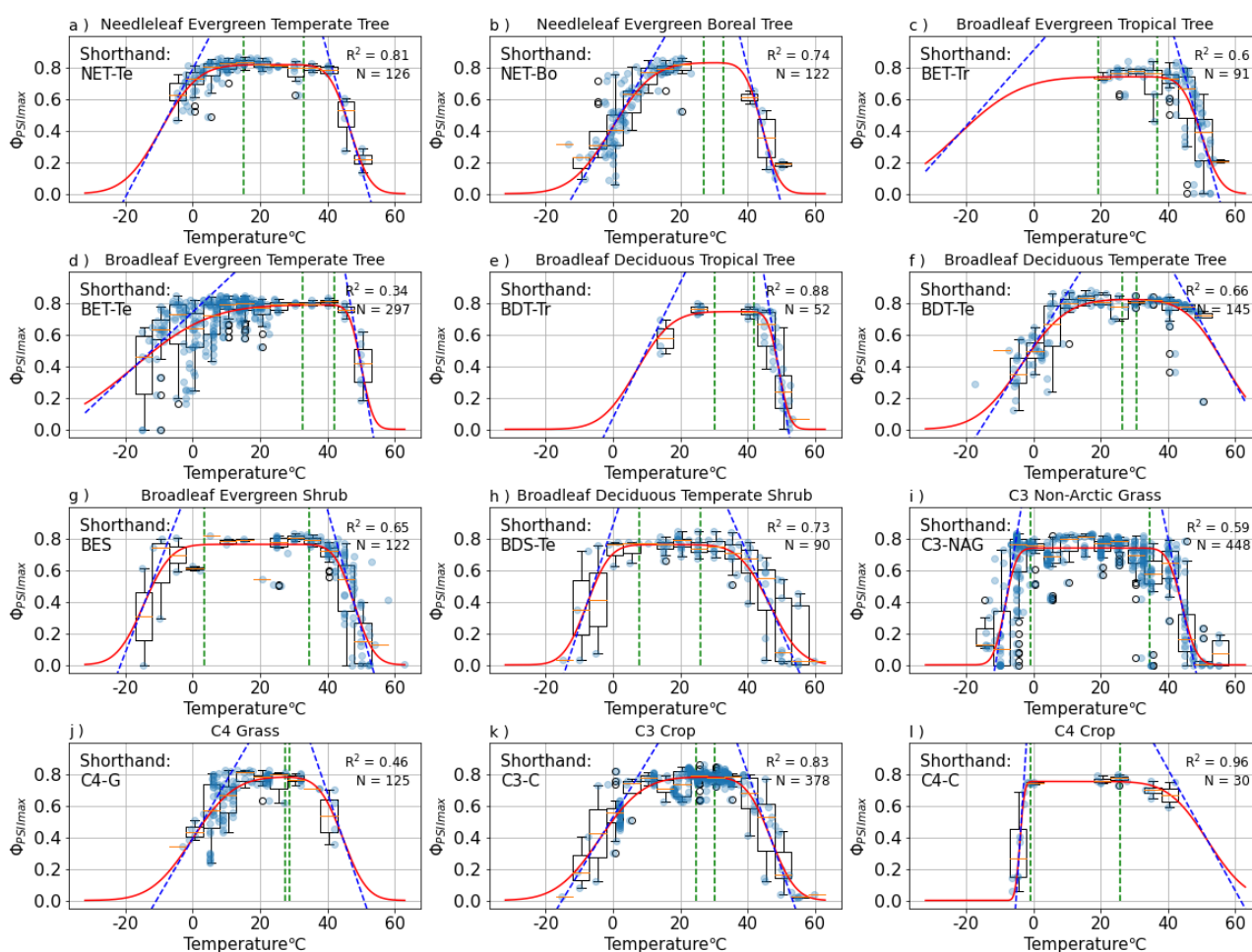
340 Figure 3. PFT-specific parameterization results for 12 plant functional types, with the abbreviations (a) NET-Te, (b) NET-Bo, (c) BET-Tr, (d) BET-Te, (e) BDT-Tr, (f) BDT-Te, (g) BES, (h) BDS-Te, (i) C3-NAG, (j) C4-G, (k) C3-C, and (l) C4-C. The red line is the resulting PFT-specific model (Eq. 1). The blue dotted lines depict the slope of the model at the temperature m_1 ( m_2 ) where \Phi_{PSII\max} declines 50% from maximum a , and its slope is the resiliency parameter s_1 ( s_2 ) for cold (hot) temperatures. The left (right) vertical green dotted lines depict the tolerance parameter T_{MC} ( T_{MH} ) for cold (hot) temperatures, and the region 345 between them is the range of temperatures at which \Phi_{PSII\max} remains constant.
