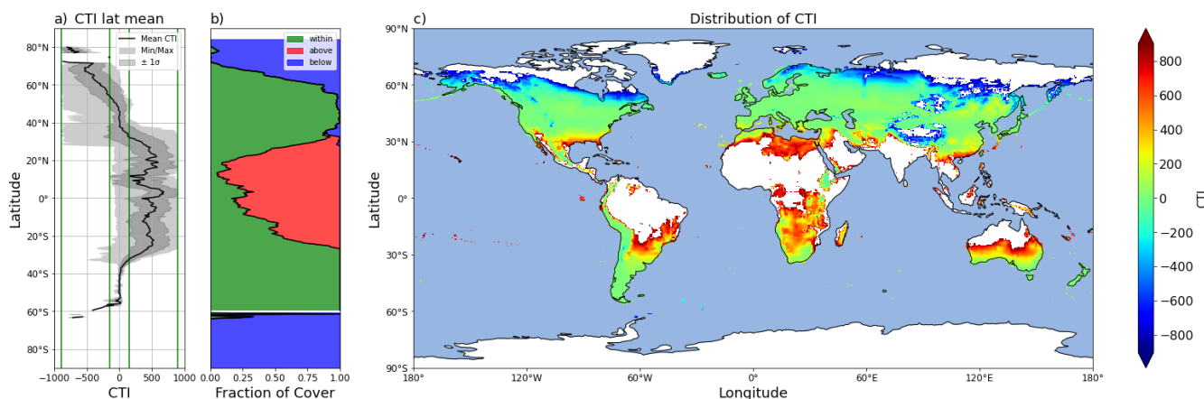
525 Figure 8. Global Distribution of CTI values and their latitudinal trends. (a) Latitude mean CTI values of all land grid cells with |CTI| not larger than 900 (black line), with both the minimum and maximum (light gray), as well as \pm the standard deviation ( \sigma ) (dark gray). Four green lines from the left to the right demonstrate the CTI bounds of -900, -150, 150, and 900, respectively. The range of 150 \leq |CTI| \leq 900 refers to the CTI range at which the temperature- \Phi_{PSII_{max}} relationship was improved by CTI- 530 informed parameterization compared with the PFT-specific parameterization. (b) The percentage of land grid cells at each latitude that were below (blue), within (green), and above (red) the range of |CTI| \leq 900 . (c) Map depicting the global distribution of grid cells at which |CTI| \leq 900 .
