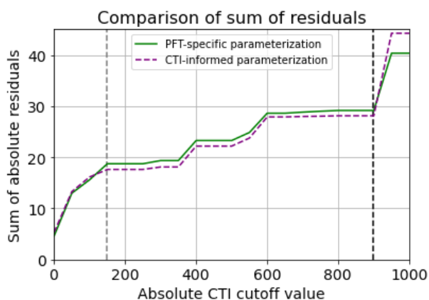
500 Figure 7. Comparing the sum of the magnitude of the prediction residuals between CTI-informed and PFT-specific parameterization of vegetative \Phi_{\text{PSII}_{\text{max}}} -temperature relationship.
