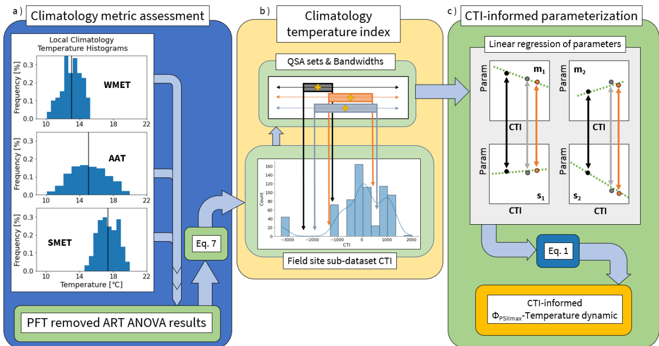
Figure 2. A pipeline of incorporating climatological temperature's effect on the modelled parameterization of temperature tolerance and resilience of vegetative \Phi_{PSII_{max}} , including (a) quantifying the histogram frequency distribution of three climatological temperature metrics (WMET, SMET, AAT) within the field site sub-dataset and their contributions to the prediction deficiency estimated by the developed PFT-specific temperature- \Phi_{PSII_{max}} functions using ART ANOVA. WMET and SMET refer to the median experienced temperature in the winter and summer, respectively, while AAT refers to the annual average temperature calculated using 0.5^\circ \times 0.5^\circ CRUNCEP v.7 hourly temperature dataset over 1985-2016. (b) calculating the Climatology Temperature Index (CTI) for all data in the field site sub-dataset using results of ART ANOVA and Eq. 7, with the resulting distribution of CTI values shown in a histogram, and the Quantile System Approach (QSA)-based data grouping and parameters ( m_1 , m_2 , s_1 , s_2 ) estimation. Here, QSA refers to using multiple bandwidths (shown as different color boxes) to group data for fitting Eq. 1, varying the range of the selected data across the whole dataset, and recording the central CTI (shown as gold cross) and resulting parameters. (c) The CTI-informed parameterization of temperature- \Phi_{PSII_{max}} dynamic, which linearly regressed each of the four parameters ( m_1 , m_2 , s_1 , s_2 ) on the corresponding central CTI values resulting in a CTI-informed parameter estimation for the temperature- \Phi_{PSII_{max}} function.
