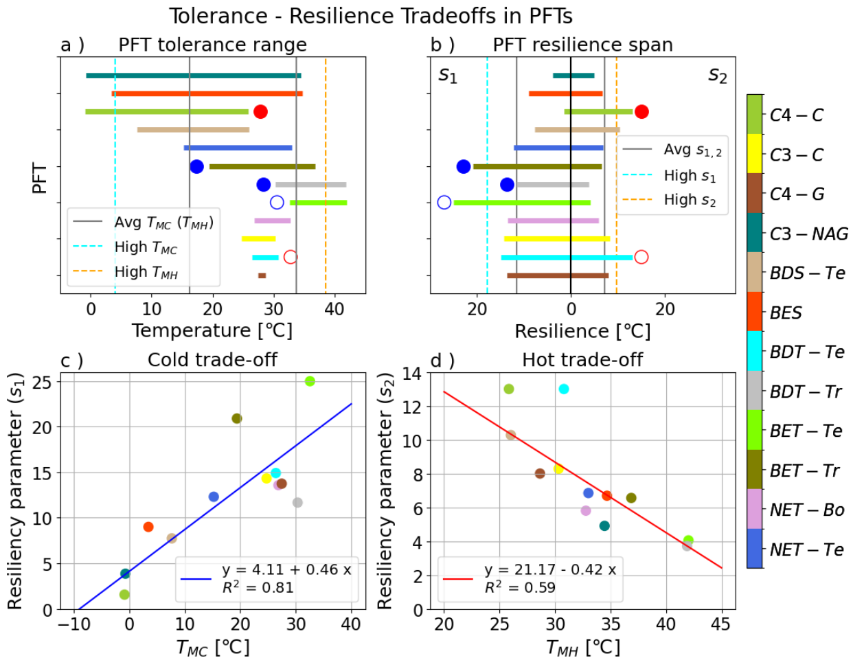
405 Figure 4. Visualization of the PFT-specific tolerance and resilience parameters, including (a) the tolerance range of temperatures across which \Phi_{PSII_{max}} remains consistently near the maximum modelled value (a) for the 12 modelled PFTs, as defined by the T_{MC} and T_{MH} values; (b) the cold ( s_1 ) and hot ( s_2 ) temperature resiliencies of the 12 modelled PFTs, labelled in the upper left and right corners respectively; (c) the trade-off between cold tolerance ( T_{MC} ) and resiliency ( s_1 ); (d) the trade- off between hot tolerance ( T_{MH} ) and resiliency ( s_2 ) for the 12 modelled PFTs. PFTs with a filled blue circle next to their parameter value in subplots (a-b) were not used in determining the respective cold temperature parameters' mean and standard deviation, and similarly PFTs with filled red circles next to their parameter values in subplots (a-b) were not used in 410 determining the respective hot temperature parameters' mean and standard deviation. Open circles of red or blue in subplots (a-b) identify a PFT with data such that the resulting cold or hot parameter results should be taken with some caution. The gray lines in subplots (a-b) are the average parameter values. The high cold and high hot tolerance classifications are based on the PFT having a T_{MC} or T_{MH} value that is 1\sigma less than or greater than the respective average tolerance value and are represented by the blue and orange dashed lines respectively. The high resiliency parameters are defined both as having s_1 or s_2 that is 1\sigma greater than the respective average value across considered PFT values.
