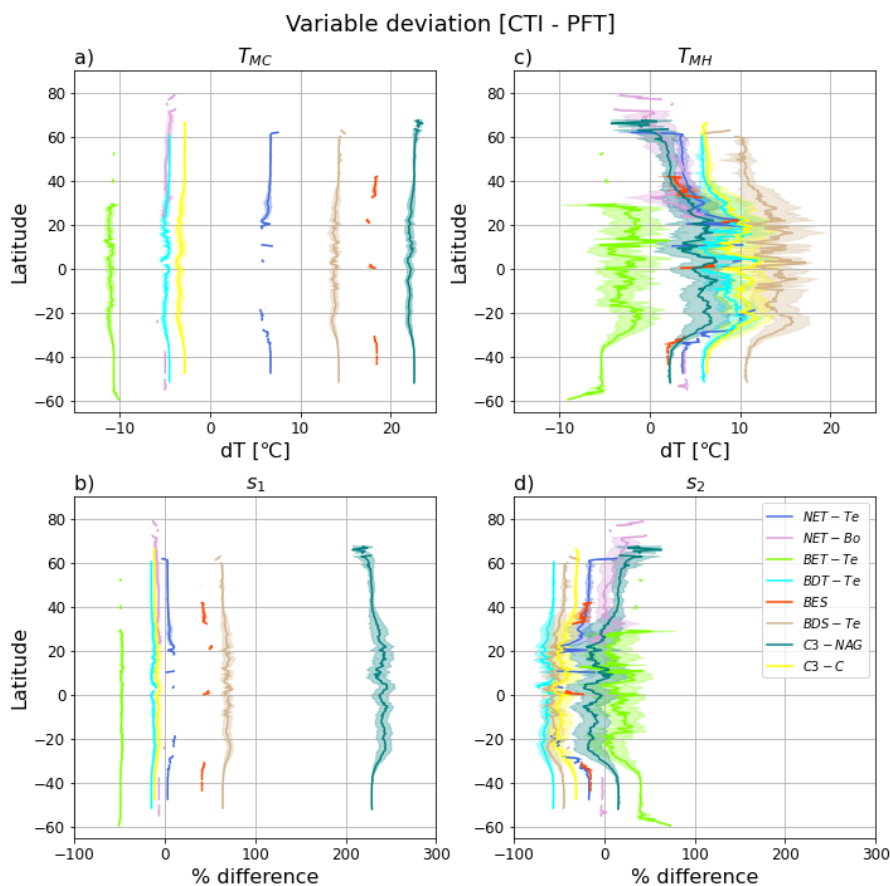
590 Figure 10. Latitudinal mean and standard deviation ( \sigma ) of the difference between CTI-informed and PFT-specific temperature tolerances metrics and resilience parameters of vegetative \Phi_{PSII_{max}} values, including (a) cold temperature tolerance ( T_{MC} ), (b) cold temperature resilience ( s_1 ), (c) hot temperature tolerance ( T_{MH} ), and (d) hot temperature resilience ( s_2 ). Here only grid cells having |CTI| \leq 900 and targeted PFT cover are included in the calculation of latitudinal mean and standard deviation. Targeted PFTs refer to PFTs which total covered area within the grid cells having |CTI| \leq 900 accounts for \geq 50\% of its global total distribution area. Each PFT-specific result is shown as separate colors, with the shaded regions of the same color are \pm 1\sigma at each latitude.
