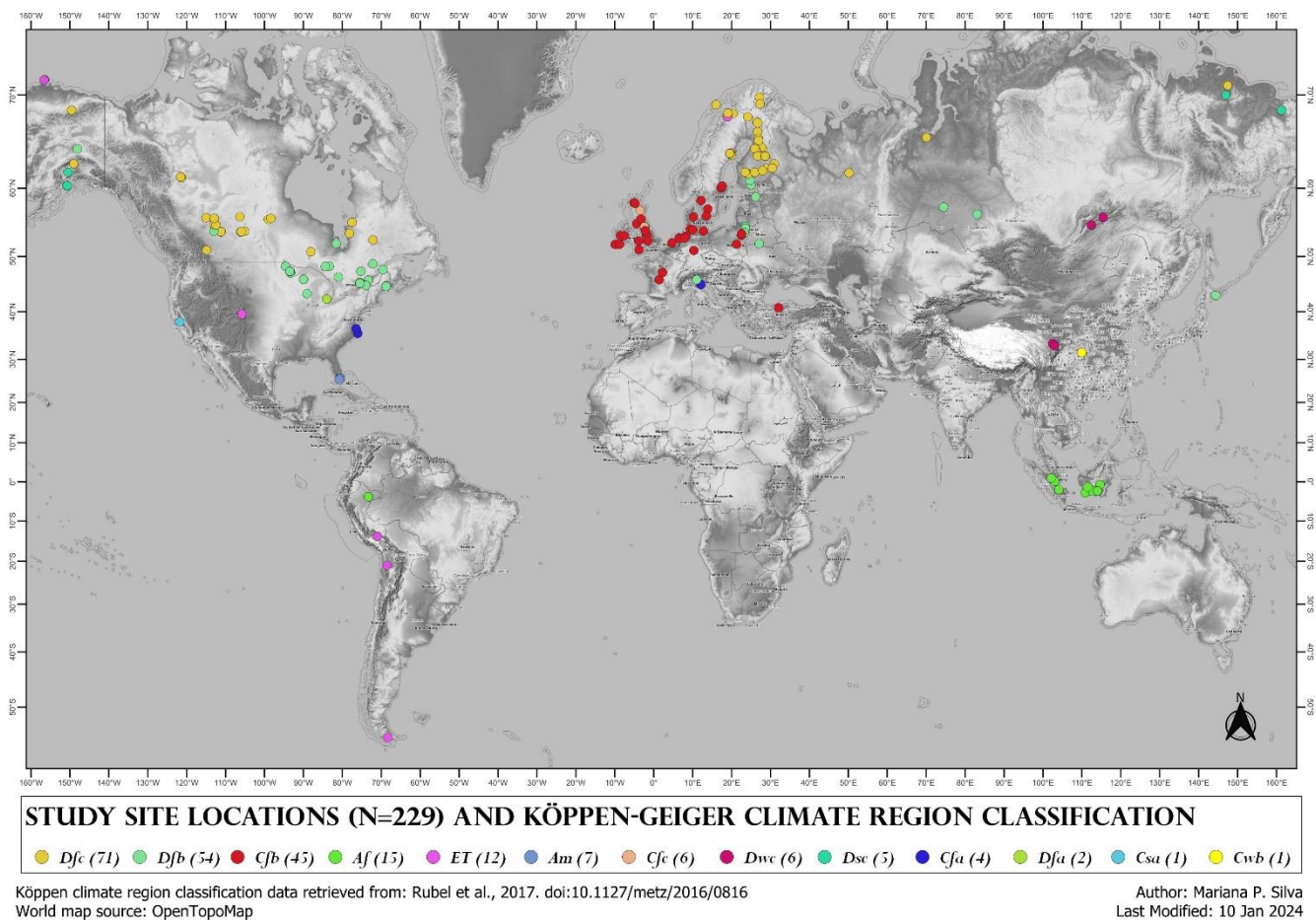
780 Figure 2: Individual site locations for the 229 sites identified in papers from this review, with their corresponding Köppen-Geiger climate region classifications. Map generated using QGIS.
