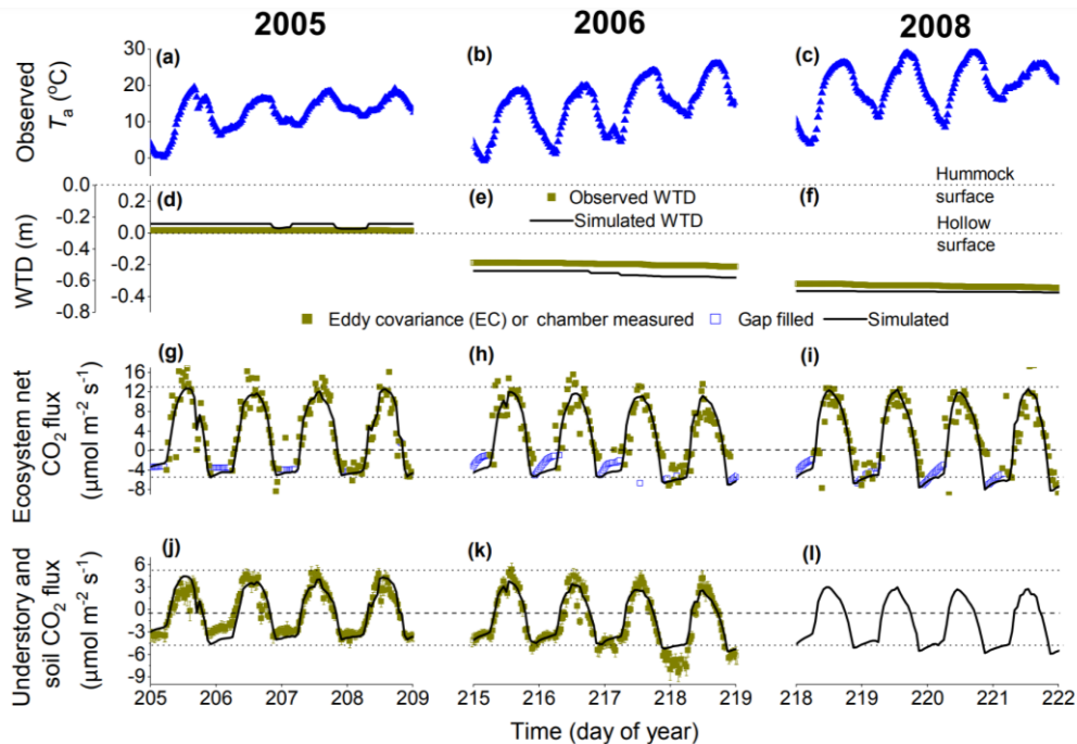
790 Figure 4: Simulated hourly WTD and CO 2 fluxes for July-August 2005, 2006, and 2008 by Mezbahuddin et al. (2017) using ecosys. Compared against half-hourly observations (a-c) air temperatures ( T_a ), (d-f) WTD, (g-i) EC-measured and gap-filled net CO 2 fluxes, and (j-l) automated chamber-measured soil CO 2 . No chamber CO 2 flux measurement was available for 2008; bars for 2005-2006 chamber measurements represent standard errors (j-k). A positive flux indicates a flux entering the system, and a positive WTD represents a depth above the surface.
