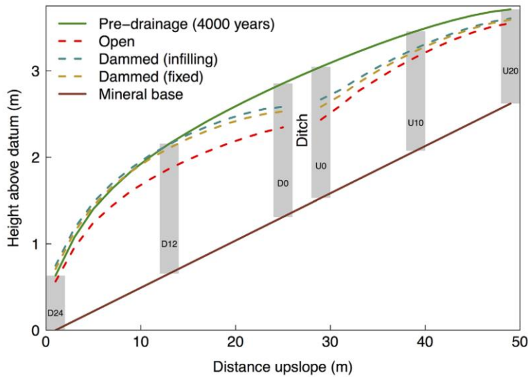
785 Figure 3: Predicted peatland surface height before and after (300 years) ditch drainage and damming imposed upon a blanket bog transect, modelled using DigiBog by Young et al. (2017). Peat accumulation is modelled here alongside hydrology for the annotated peat columns (e.g., D24, D12); columns are identified using their position upslope (U) or downslope (D) of the ditch and the distance (m) of their edges that are nearest the ditch (e.g., column U10 occurs 10 m upslope of the ditch).
