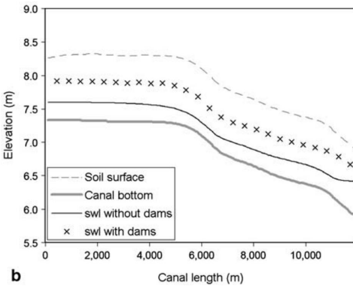
Figure 6: GIS-based predictions of water level rise for a tropical peatland using SIMGRO (Jaenicke et al., 2010). (a) Plan view of groundwater level rise after dam construction; (b) Surface water level rise (relative to soil surface elevation) in a single canal after dam construction.
