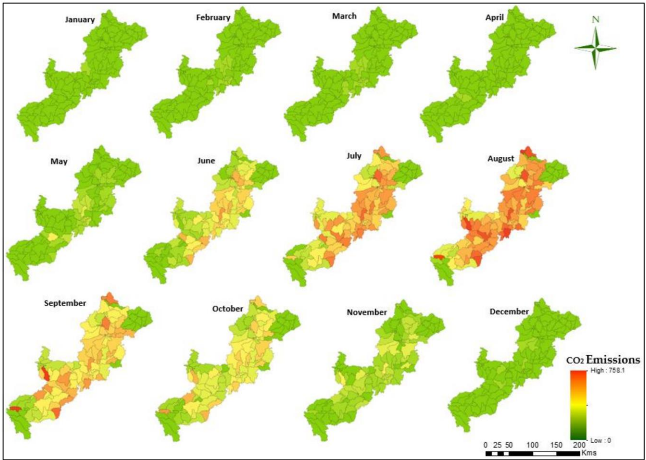
795 Figure 5: Spatiotemporal CO 2 emissions ( \mu\text{mol CO}_2\text{-C m}^{-2}\text{ day}^{-1} ) for the Athabasca River Basin as developed by Melaku et al. (2022) using SWAT. The model also produced 3-year continuous predictions for CO 2 emissions, NEE, WTD, Reco, and soil temperature, each representing an aggregate value for the whole basin.
