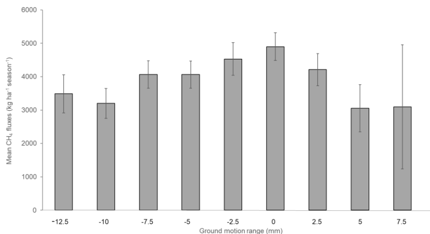
450 Figure 7. Average seasonal CH 4 emissions for different ground motion ranges (categories in 2.5 mm ranges) across the three study sites. Negative values indicate subsidence and positive values indicate uplift. Mean and SE are shown.
