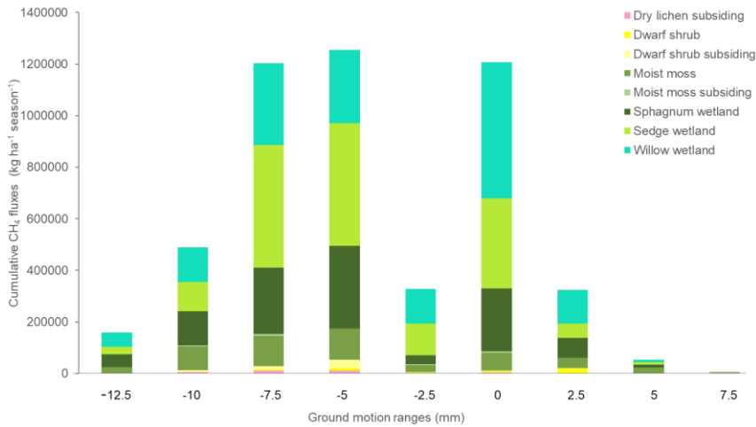
465 Figure 8. Cumulative CH 4 emission (± SE) for different ground motions across the thaw seasons of 2017 and 2020 for pixels (i.e. a sum of the CH 4 emissions from all pixel of a given ground motion (categories in 2.5 mm ranges)) of the target vegetation classes. The dry lichen vegetation types did not cover large enough areas to be evaluated on the 20×20 m pixel scale of the ground motion data and is therefore not included in this comparison. Negative values indicate subsidence and positive values indicate uplift. 470
