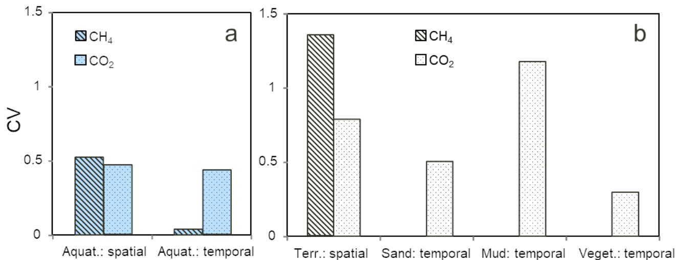
325 Figure 6: Coefficients of variation of spatial (calculated from Table 2) and temporal (calculated from Figure 5) variability of CH 4 fluxes and CO 2 fluxes of aquatic sites (a) and dry sites (b) accordingly. Temporal variability of CH 4 fluxes from terrestrial sites was not calculated.
