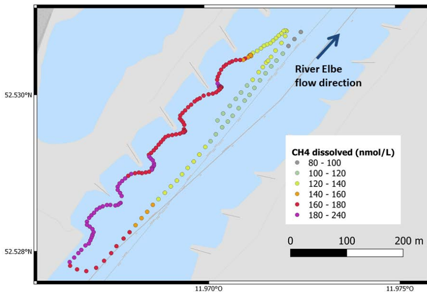
255 Figure 3: Concentrations of dissolved CH 4 in the water measured continuously with a mobile gas extraction unit connected to a GHG analyser. Measurements were carried out from an inflatable boat on 21.8.2022 between 16:18 and 16:51. CO 2 was also measured by the GHG analyzer but data were not used because gas extraction was different for CH 4 and CO 2 and the system was optimized for CH 4 .
