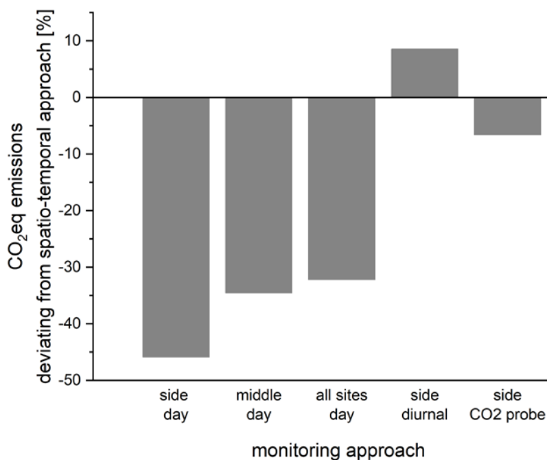
Figure 7: Deviation of total GHG emissions (CO 2 -eq) obtained by different monitoring approaches from optimal spatio-temporal approach (spatial variability of CH 4 and both spatial and temporal variability of CO 2 considered).
