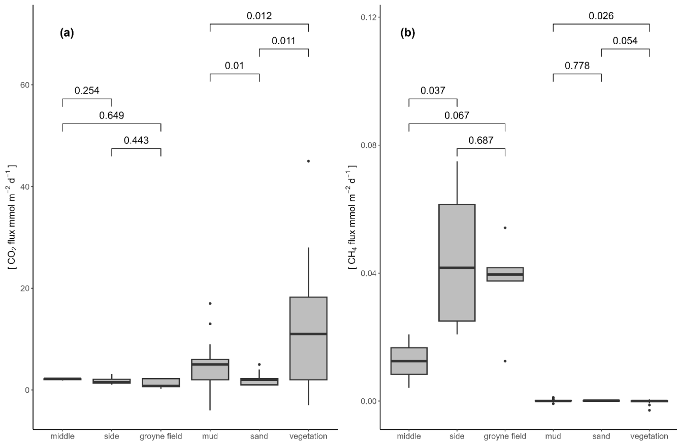
Figure 4: Boxplots comparing CO 2 flux (a) and CH 4 flux (b) in different habitat types. Numbers within the plots indicate p-values of pairwise comparisons using Wilcoxon tests (same data as in table 2).
