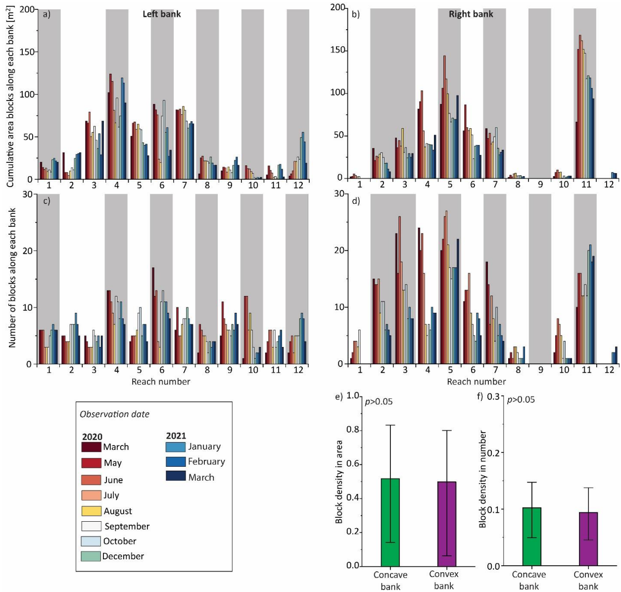
Fig. S5. The area (a, b) and number (c, d) of blocks observed within each reach along the left and right banks of Dean Creek over the course of the study (see Figure 1 for reach locations). We designated the left and right banks based on the flooding direction, so that if one were standing at the mouth then the left bank of each reach would be on the left. The gray and white backgrounds represent concave and convex banks, respectively. Plots (e-f) are comparisons of block density in terms of area and number observed per meter of shoreline within each reach along banks with contrasting shapes. The data are displayed as mean \pm standard deviation and the p-value in each panel is the result of a one-way ANOVA test.
