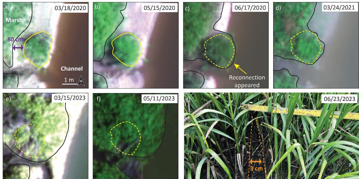
Fig. S1. The extended tracking of the reconnected block (See Figs. 2i-l). (a-d) are the same as Figs. 2i-l, showing reconnection of a slump block through 03/24/2021, with the intact marsh boundary shown as a black line and the yellow line indicating the slump block. The initial width of the gap between the block and the marsh is indicated in panel a. The dashed yellow line represents the boundaries of the location of the block on 05/2020. (e-f) are additional observations of this block in March and May 2023. (g) is a photo taken in the field at the site. The area between the orange dashed lines represents the possible area remaining from the initial gap between the block and the main marsh platform seen in panel a. Other than this, we did not observe any obvious space between vegetation patches in the surrounding areas
