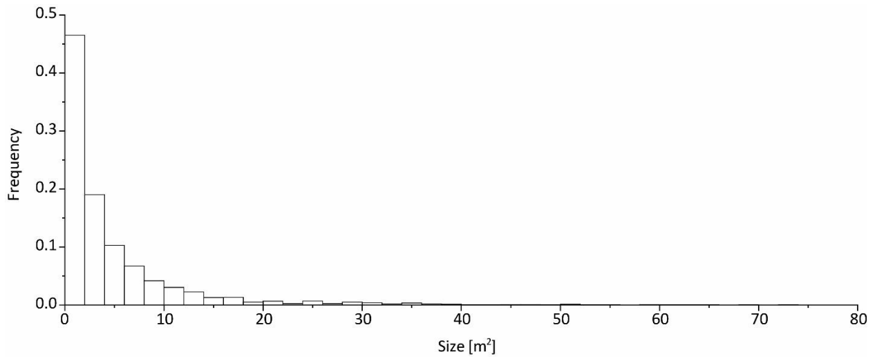
Fig. S4. The size frequency distribution of all blocks identified in the study.
