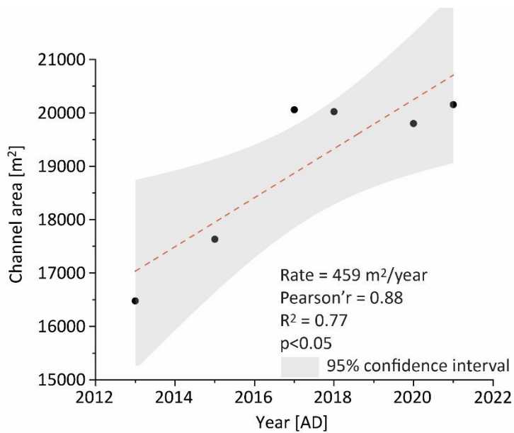
Fig. S6. Long-term change in channel area of the Dean Creek study site. Estimates of channel area between 2013 and 2018 were determined by digitization of marsh-channel boundary based on aircraft loaded aerial photo collected on 12/13/2013, 07/09/2015, 11/27/2017 and 10/31/2018, which can be found GCE-LTER archive data ( gce-lter.marisci.uga.edu ). Channel areas in 2020 and 2021 were determined by channel digitization carried out on drone images collected on 03/15/2020 and 03/24/2021 as part of this study. The rate of changes in channel area was determined by linear regression. The shaded area represents the 95% confidence interval. The p-value in the figure is the result of a one-way ANOVA test.
