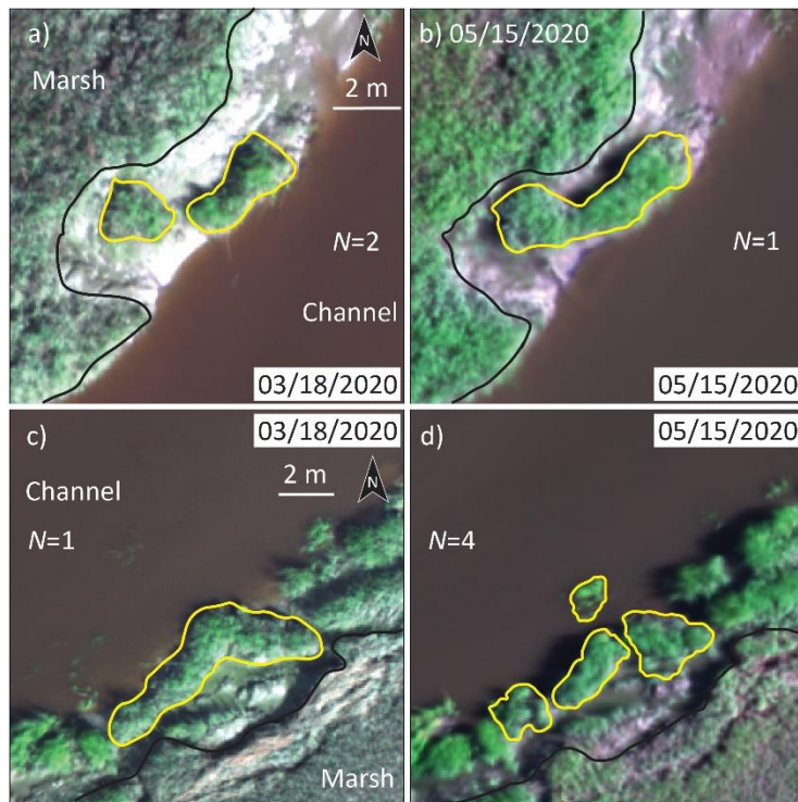
Fig. S2. Examples of block reconnection (a-b) and splitting (c-d). The number of blocks appearing in each panel is represented by N . The yellow lines in each panel represent the boundary of slump blocks, and the black line in each panel represents intact marsh boundaries. The 2 blocks in panel a are merged in panel b, whereas the block in panel c has split into 4 components in panel d.
