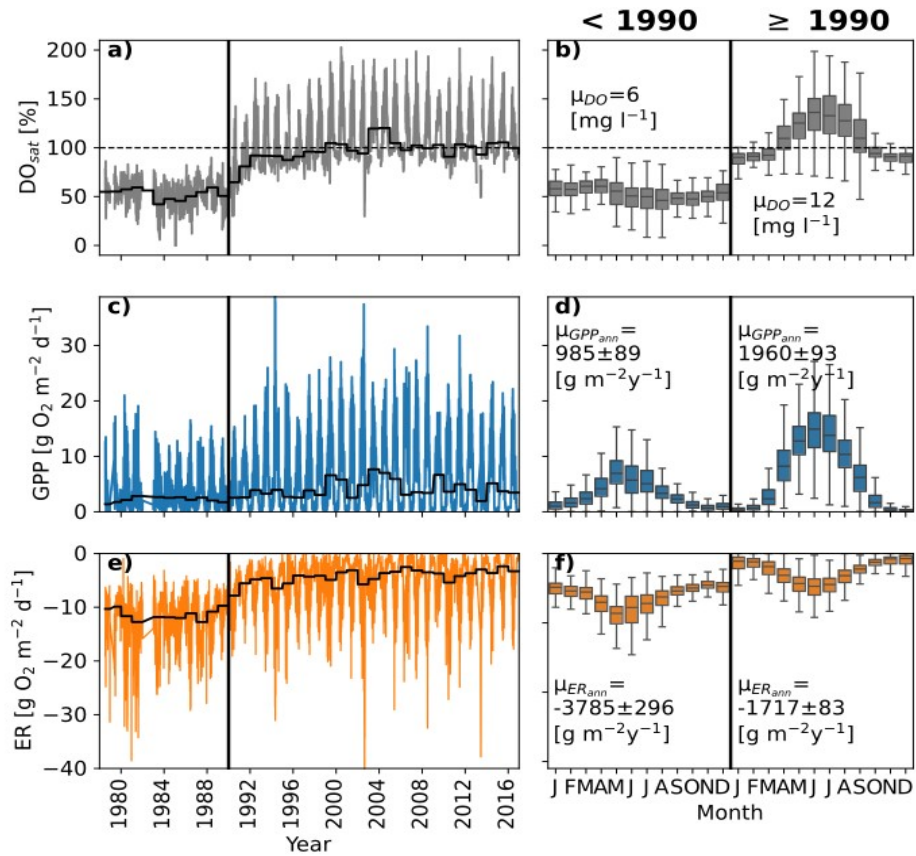
11Figure 3. Time series of daily dissolved oxygen saturation ( DO_{sat} a), daily gross primary production estimates ( GPP , c), and ecosystem respiration estimates ( ER , e). The black lines show the annual median DO , GPP and ER values. Panels b, d, and f show the mean monthly patterns for DO_{sat} , GPP , and ER , each before and after 1990. \mu_{DO} represents the mean DO concentrations, \mu_{GPP_{ann}} and \mu_{ER_{ann}} the mean annual GPP and ER rates.
