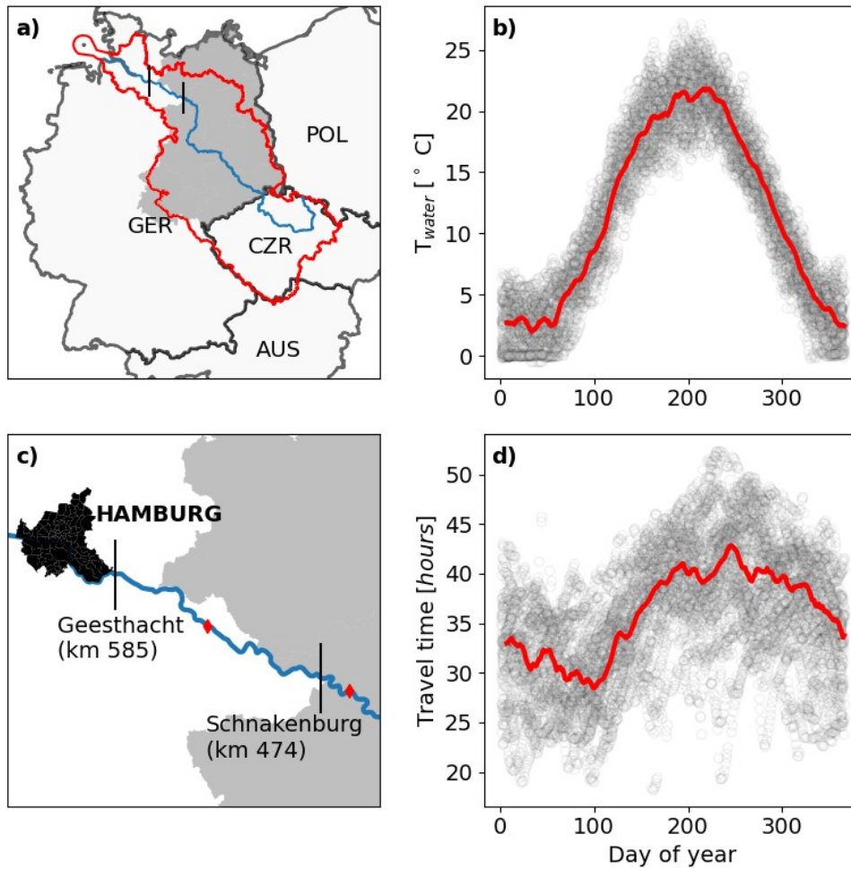
Figure 1: Location of the investigated river segment (a, c) in Europe. The blue line marks the Elbe main stream and the red outline represents the catchment. Black vertical lines mark the beginning and the end of the segment (sampling locations). Red diamonds in panel c indicate discharge gages. The former area of the German Democratic Republic (GDR) is represented by the grey shade. Intra-annual patterns of water temperature (b) and travel time (d). Circles show raw data, and red lines multi-year 7 day running means for each day of the year.
