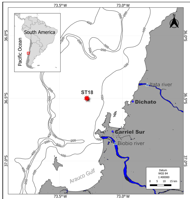
Figure 1. Time series location map (ST18) over the central Chile upwelling platform. The Itata and Biobio rivers, Carriel sur meteorological station and Dichato town are indicated.
