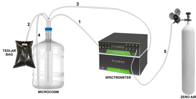
Figure 2. Assembly of the microcosm for long-term experiments (10 L). Capillary 1 is connected directly to the spectrometer. Capillary 2 is connected to a TEDLAR bag filled with N 2 (3L). Capillary 3 is removable and connected to the outlet of the spectrometer. Capillary 4 is connected to a loose hose for water sampling and hose 5 is connected to zero air.
