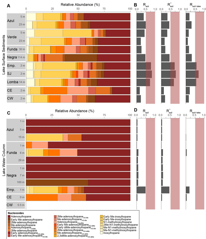
410 Figure 7: (A) Relative abundance of nucleosides identified in the surface sediment samples for all Azorean lakes (where Emp = Empadadas; SJ = São Jorge, CE = Cubres East; CW = Cubres West) with the (B) R_{soil} (see equation 1), R'_{soil} , and R_{soil-lake} calculated for each sample. (C) The distribution of nucleosides in water column samples and their respective (D) R_{soil} , R'_{soil} , and R_{soil-lake} values are also shown. The red bars indicate the terrestrial end-member values. Note: nucleosides were not detected in the water column SPM of Cubres West.
