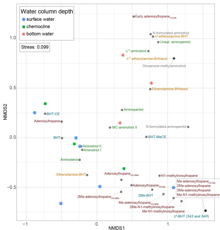
Figure 5: NMDS visualization of BHP distributions between different water column samples from lakes Azul, Empadadas, Funda, and Negra, as well as Cubres East and West. Note: f or Empadadas, Cubres East, and Cubres West we only have surface water column samples since the sampling locations were less than 3.5 m deep.
