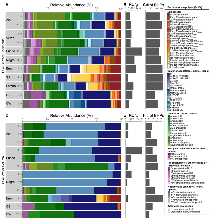
260 Figure 2: (A) Relative abundance of all BHPs found in surface sediment samples labelled with the lake depth (meters) at which they were collected where Emp. = Empadadas, SJ = São Jorge, CE = Cubres East, and CW = Cubres West (all raw data is available in the supplementary material). (B) The response units (RU) of BHPs in the sediment samples normalized to g of dry sediment and (C) the number of BHPs identified in each sample. (D) Relative abundance of BHPs identified in water column samples from the different lakes and lagoons (E) with the total response units/L of water filtered and (F) number of BHPs shown.
