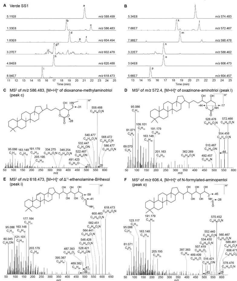
Figure 3: (A) Partial mass chromatograms of ethenolamine-BHT (peak a), \Delta^6 -ethenolamine-BHT (peak b), dioxanone-methylaminotriol (peak c), ethenolamine-BHPentol (peak d), isomers of methylcarbamate aminotriol (peaks e and f), a potential peak for unsaturated ethenolamine-BHPentol (peak g), ethenolamine-BHhexol (peak h), and \Delta^{11} -ethenolamine-BHhexol (peak i). (B) Partial mass chromatograms of N-formylated-aminotriol (peak j), \Delta^6 -N-formylated-aminotriol (peak k), oxazinone-aminotriol (peak l), N-formylated-aminotetrol (peak m), \Delta^{11} -N-formylated-aminotetrol (peak n), N-formylated-aminopentol (peak o), and \Delta^{11} -N-formylated-aminopentol (peak p). MS 2 spectrum of (C) the dioxanone-methylaminotriol in m/z 586.483 (peak c) and (D) the oxazinone-aminotriol composite (peak l) with tentative structures shown. MS 2 spectrum of (E) [M+H] + \Delta^{11} -ethenolamine-BHhexol and (F) [M+H] + N-formylated-aminopentol with tentative structures shown. The chromatograms are from a surface sediment sample from Lake Verde.
