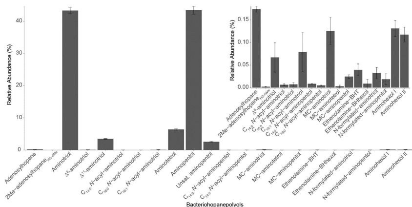
455 Figure 8: BHP profile of Methylobacter-Methylotenera co-culture (n=3). Note: the BHPs present in low abundance are shown in the inset figure.
