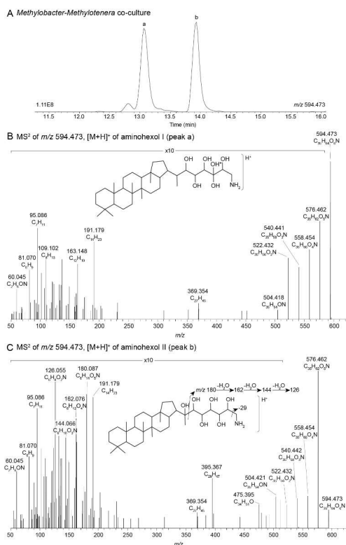
480 Figure 9: (A) Partial mass chromatograms of aminohexol I (peak a) and II (peak b) BHPs from the Methylobacter-Methylotenera co-culture with. MS 2 spectra for (B) aminohexol I and (C) aminohexol II and the proposed-tentative structures shown . The asterisk (*) indicates arbitrary placement of the hydroxyl group on the side chain.
