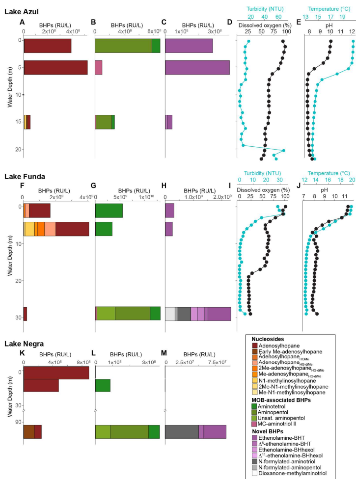
395 Figure 6: Water column profiles for Lakes Azul (A-E), Funda (F-J), and Negra (K-M). Plots A, F, and K show the relative units/liter (RU/L) of nucleoside BHPs identified in the water column. Plots B, G, and L show the relative response units/liter (RU/L) of BHPs associated with methane-oxidizing bacteria found in the water column. Plots C, H, and M display the response relative units/liter (RU/L) of ethenolamine-BHPs and recently identified composite BHPs (i.e., N-formylated-aminoBHPs and dioxanone-methylaminotriol) identified in the water column. D and I show the turbidity (blue) and dissolved oxygen (pink/black) from the water column at the time of sampling in June 2018. Similarly, E and J display the temperature (blue) and pH (pink/black) profiles of the water column at the time of sampling for both Lakes Azul and Funda.
