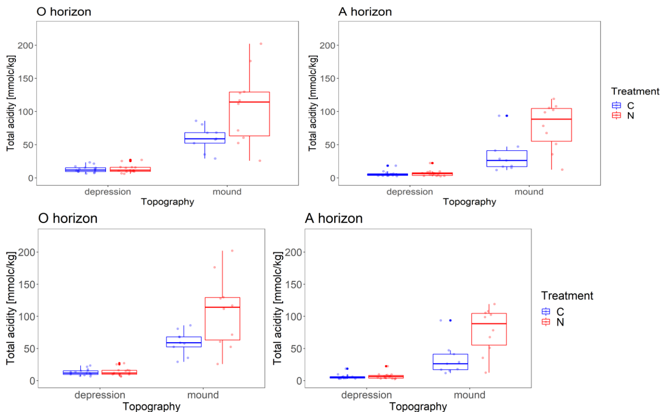
Figure 4: Observed total soil acidity values from all years for O and A horizon for both topographical features (mounds and depressions).
