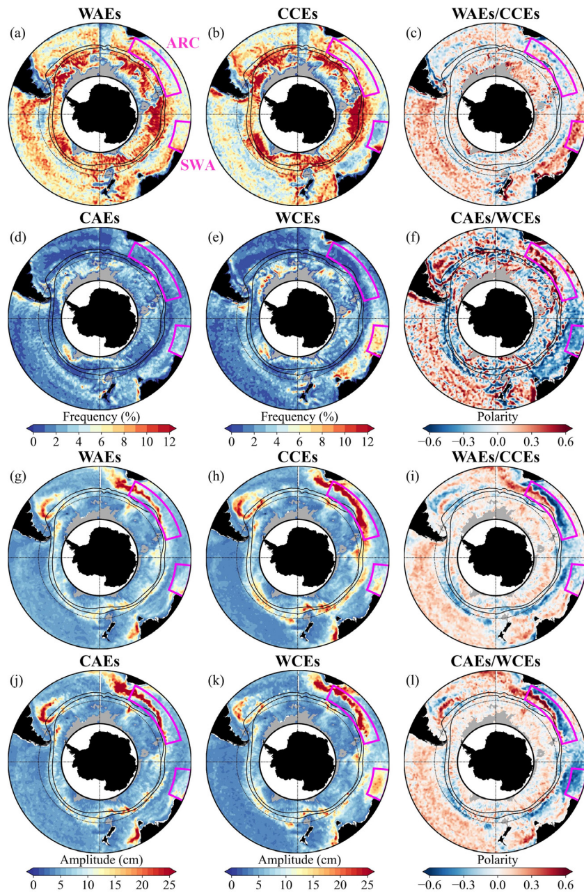
Figure 2. Spatial distribution of (a, b, d, and e) eddy frequency, (g, h, j, and k) eddy amplitude, and eddy polarity dominance in the SO from 1996 to 2015. (c, f) Ratio of the area occupied by WAEs/CAEs over the area covered by CCEs/WCEs). (i, l) Ratio of amplitude for WAEs/CAEs over CCEs/WCEs). For (c, f, i, l) eddy polarity, values >0 in red and <0 in blue mark the dominance of AEs and CE, respectively. Black solid lines show the mean northern ( SAF ) and southern ( PF ) positions of the ACC major fronts ( Sallée et al., 2008 ). The black dotted circle is 50^\circ S. The magenta boxes represent ARC and SWA regions.
