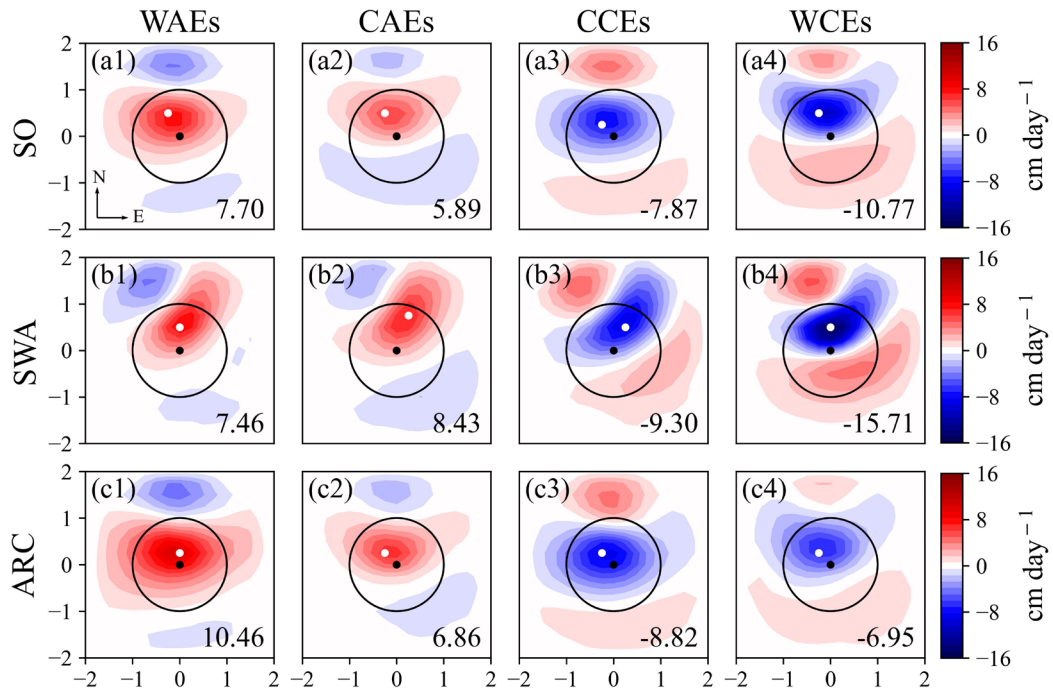
795 Figure 8. Eddy-centric composite averages for eddy-induced Ekman pumping in the SO, SWA, and ARC. On each map, a black dot denotes the eddy center, and a white dot denotes the center location of variables (defined by the location of the extremum value). Contour intervals are 1.067 \text{ cm day}^{-1} . The numbers in the lower right corner are the extremum value.
