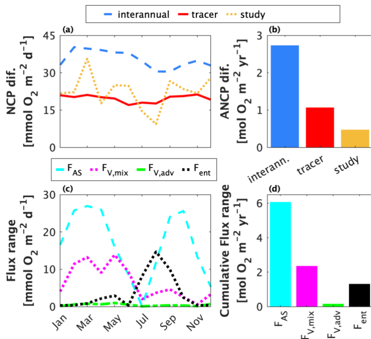
835 Figure 9. Contributions to differences between float-based net community production (NCP) and annually integrated NCP estimates at Ocean Station Papa (OSP). Panels (a) and (b) show estimates of the contributions of different factors to differences in published mixed layer-integrated NCP and ANCP estimates from OSP. The blue line/bar represent differences due to real, interannual NCP and ANCP variability; the red line/bar shows differences resulting from the choice of tracer; and the yellow line/bar represents differences between approach occurring between studies within the same year. Panels (c) and (d) represent estimates of the range of dissolved oxygen ( \text{O}_2 ) flux parameterizations across studies (Table 1). For each flux, values were calculated as the absolute range of estimates after applying the different parameterizations for each term (Table 2). F_{AS} = air-sea flux via diffusion and bubbles; F_{vmix} = vertical transport flux via diapycnal mixing; F_{vadv} = vertical transport flux via advection; F_{ent} = vertical transport flux via entrainment. Panel (d) shows the cumulative flux range over one year. 840
