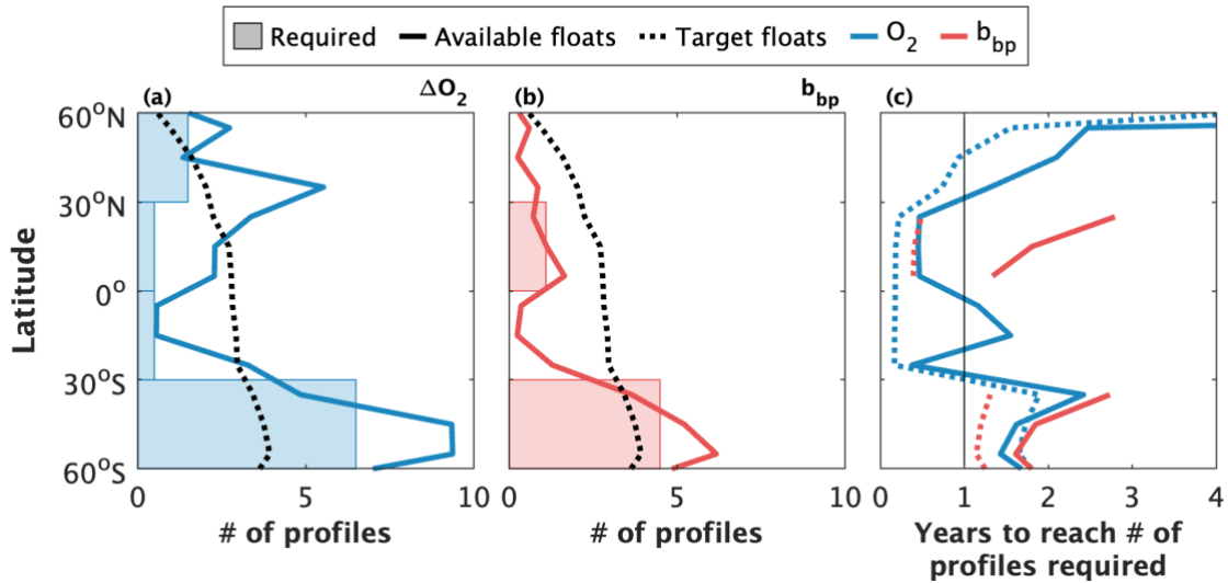
740 Figure 8. Estimates of the number of profiles and time required to derive statistically consistent gross oxygen production (GOP) and gross carbon production (GCP) estimates at different latitude bands. The shaded regions in (a) and (b) represent the estimated number of profiles required for dissolved oxygen ( O_2 ) and particle backscattering ( b_{bp} ), respectively. The minimum number of profiles required was calculated from a bootstrap analysis with a signal-to-noise threshold of 0.5. The solid lines represent the current number of profiles available for gross primary production calculations since 2010. The dashed lines represent estimates of the number of profiles obtained, per year, by a target biogeochemical-Argo array of 1000 floats deployed ocean-wide proportionally with ocean surface area, and profiling at 10.2-day intervals. Panel (c) shows an estimate of the time required to attain the minimum number of required profiles if the current active (Jan. 2023; solid lines) and target (dashed lines) biogeochemical-Argo array profiles at 10.2-day intervals. The time required was calculated as \frac{(\text{profiles required}) \times (10.2 \text{ days per profile})}{(\text{current or target \# of floats in region}) \times (365 \text{ days per year})} .
