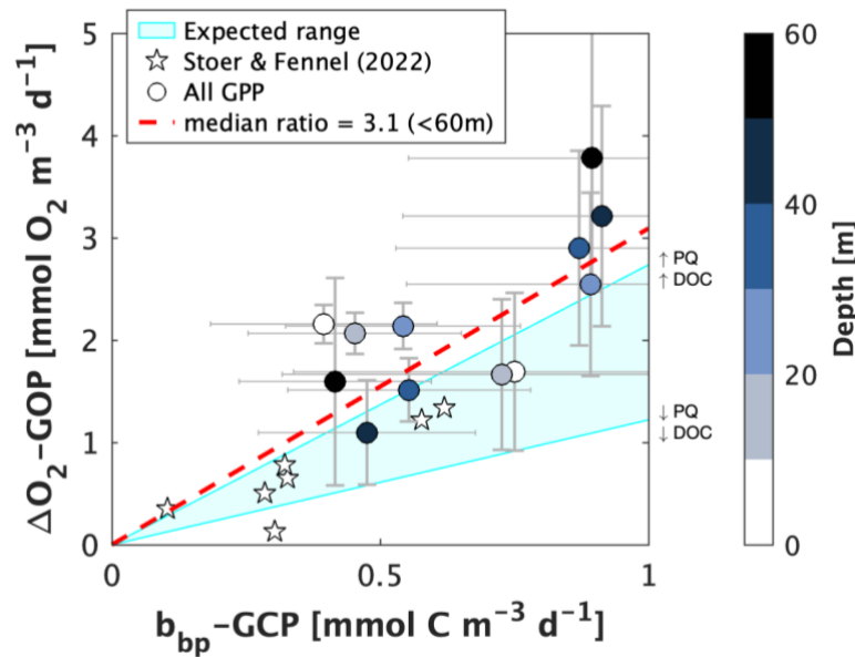
Figure 7. A comparison of depth-resolved oxygen-based estimates of gross oxygen production ( \Delta O_2\text{-GOP} ) and particle backscattering-based estimates of gross carbon production ( b_{bp}\text{-GCP} ) in waters shallower than 60 m. Data points represent values derived from co-located profiles in latitude bands or Longhurst Provinces with enough profile measurements to obtain statistically consistent GPP estimates (sect. 4.1.1). Error bars represent one standard error. Star markers represent GPP estimates from Stoer and Fennel (2023) which were obtained from co-located O_2 and b_{bp} profile measurements below the euphotic depth in the latitude range 30-60°S. GCP estimates were not converted to O_2 equivalents, nor were they adjusted for potential PER. The light blue shading represents the expected range for the relationship between GOP and GCP, given a percent extracellular release (PER) range of 18-47% (Moran et al., 2022) and photosynthetic quotient (PQ) range of 1-1.45 (Laws, 1991). The dashed line shows the median GOP:GCP ratio below 60 m.
