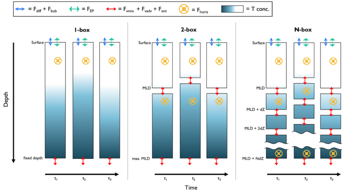
Figure 4 Schematic of box model setups for float-based NCP approaches. The columns represent a profile of tracer concentration at discrete time intervals ( t_n , where n is the n -th point in time) and the rows are divided into vertical layers ( dZ ). T conc = tracer concentration; MLD = mixed layer depth; F_{diff} = air-sea flux via diffusion; F_{bub} = air-sea flux via bubbles; F_{EP} = evaporation or precipitation flux; F_{vmix} = vertical transport flux via diapycnal mixing; F_{vadv} = vertical transport flux via advection; F_{ent} = vertical transport flux via entrainment; and F_{horiz} = horizontal transport flux.
