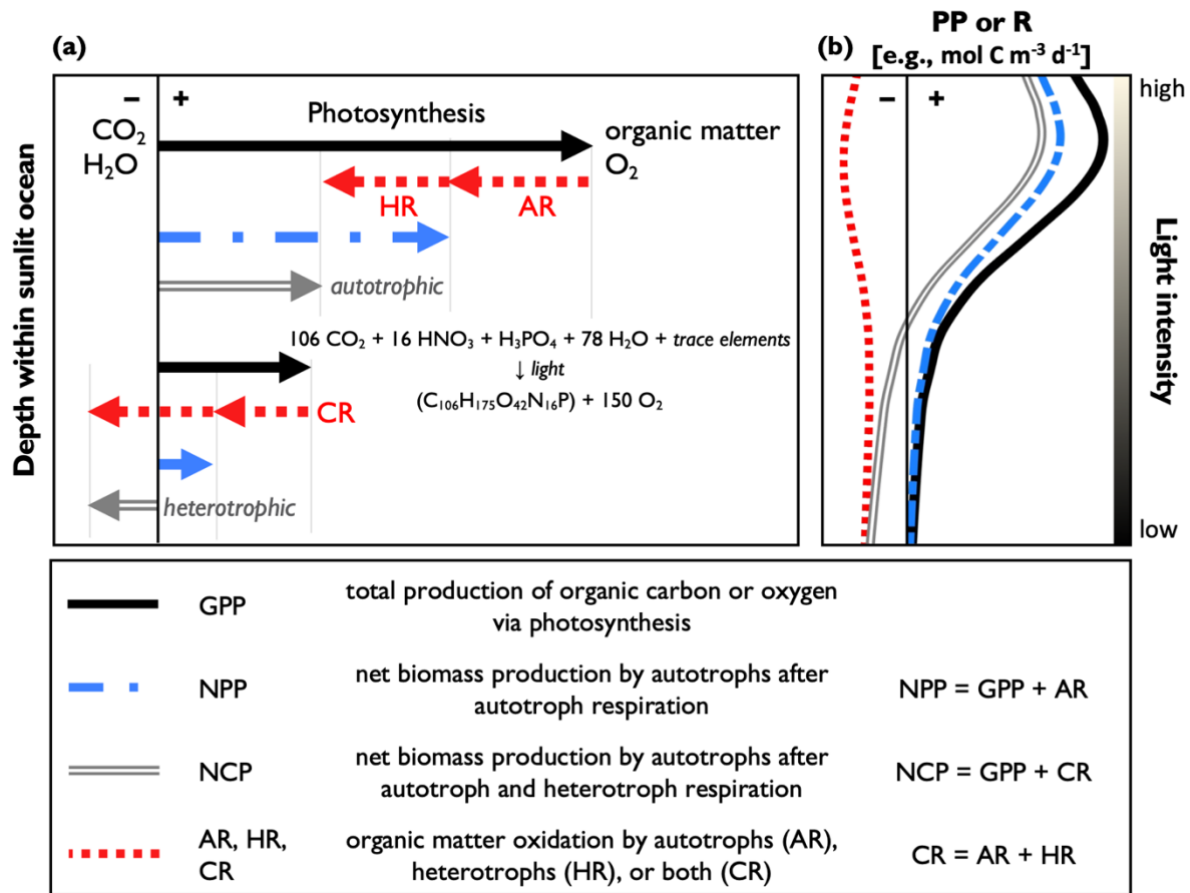
80 Figure 1. A conceptual schematic and definitions of the common primary productivity (PP) and respiration (R) metrics: gross primary production (GPP), net primary production (NPP), net community production (NCP), and autotrophic, heterotrophic and community respiration (AR, HR, CR, respectively). Panel (a) shows simplified reaction equations of organic matter production and R. The upper part of the figure represents a region of net autotrophic conditions (NCP > 0), while the lower part represents a region of net heterotrophic conditions (NCP < 0). Panel (b) represents idealized PP and CR profiles, where PP declines with depth due to the light dependency of photosynthesis with a subsurface maximum resulting from photoinhibition. The vertical axis represents water column depth, and the thin black line divides positive and negative rates. The equation represents average oceanic aerobic photosynthesis, following Redfield nutrient stoichiometry. The reverse reaction represents respiration. 85
