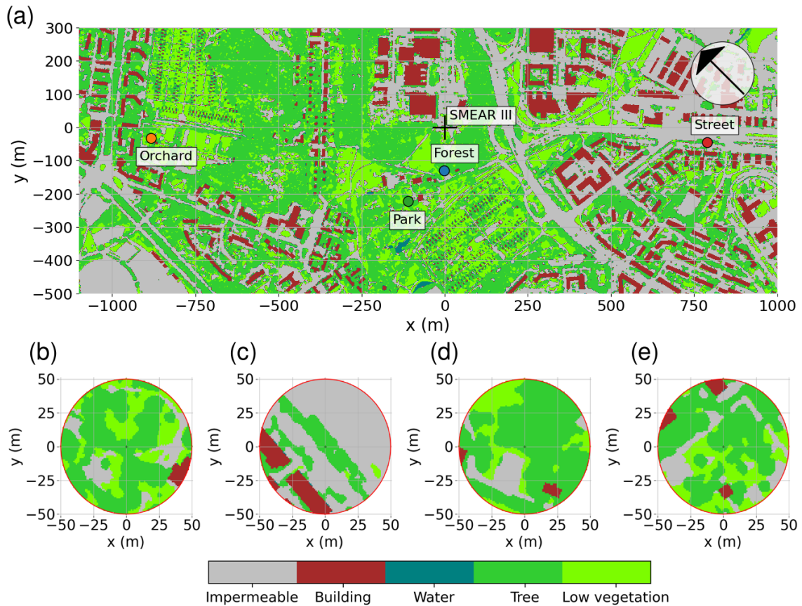
Figure 1. (a) Surface cover of the study area in Helsinki (StromJan, 2020) with the location of the monitoring sites, and surface covers at the (b) Park, (c) Street, (d) Forest, and (e) Orchard measurement sites.
