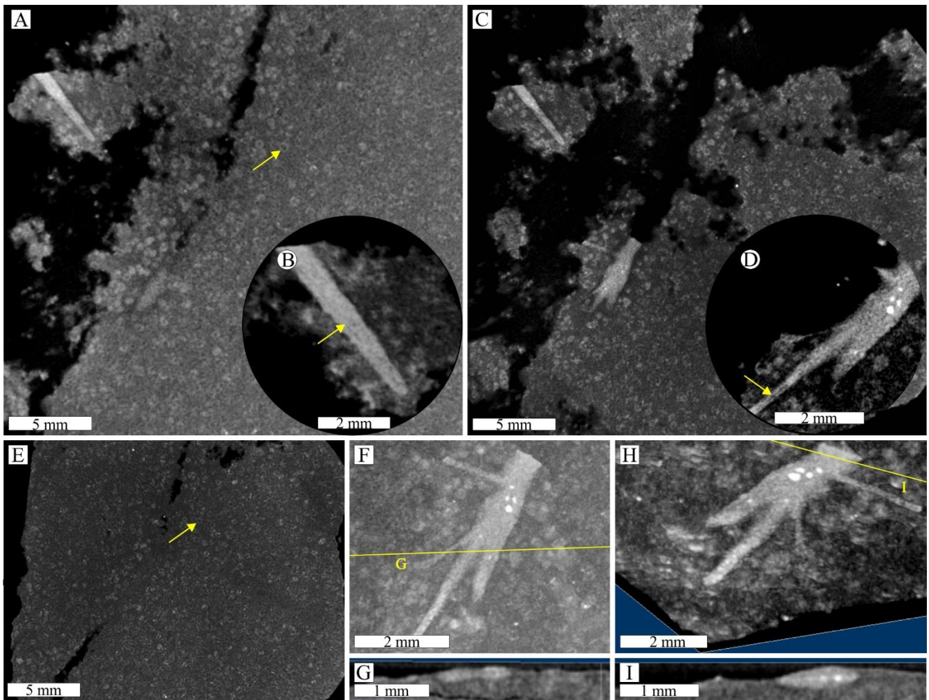
Figure 6: Micro-CT results, needle (lighter gray structure), matrix (darker gray), and matrix spheres (gray circles): A) General view of a non-ramified needle, yellow arrow point to matrix sphere; B) close view showing the internal structure (slight density differences inside the tube, yellow arrow); C) View of ramified structure; D) Close view of the ramified tubule, middle tubule less dense (yellow arrow). E) Matrix view with multiple matrix spheres (one pointed by the yellow arrow). F-H) Cross-section demonstrating the true ramification and insertion in the matrix. Fig. 6A-E, 2D micro-CT slices. Fig. 6F-I 3D volume viewer composition, F and G horizontal and G and I vertical.
