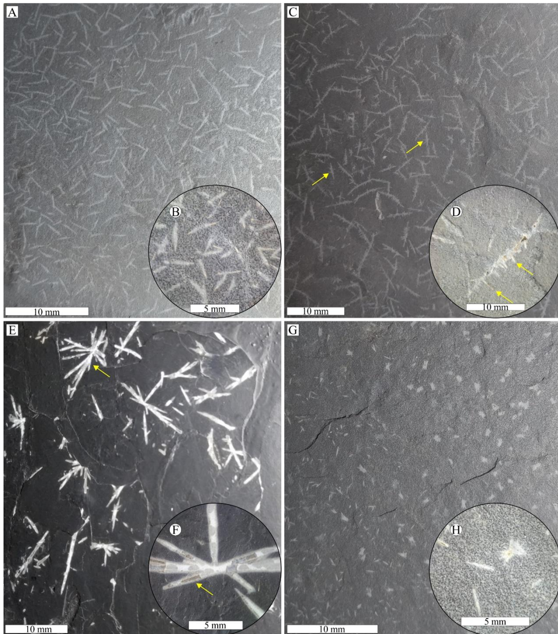
Figure 4: Informal classes of dubiofossil forms related to the matrix: A) General view of class A, loose packed unramified acicula; B) closed-up view of class A yellowish-white needles with tapered tips and fainter regions; C) General view of class B, laterally ramified needles; D) example of class B ramified acicula, branches depart from and crossing the main axis; E) General view of class C, radially ramified dubiofossil; F) Detail of class C radially ramified structures, with tapered tips, external fainter layer, and internal dark layer; G) General view of class D, small needles and dots, each dominating one side of the slab; H) Closed up view of class D non ramified needles and “dots”, small radially ramified forms. Example of branches indicated by yellow arrows.
