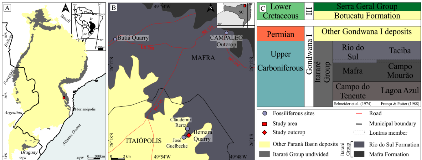
Figure 2: Location and geologic context of the collection area. A) coverage area of the Itararé Group in the Paraná Basin in south-central Brazil and neighbouring countries, study area; modified from Vesely and Assine (2006). B) Location of the collection area, Bemara Quarry, municipality of Itaiópolis and other paleontological sites in the region, including similar to Bemara Claudemir Rertz and José Guelbecke locations, geological units of study, Mafra Fm., Rio do Sul Fm. (Itararé Group) and other sequences of the Paraná Basin; CAMPALEO Outcrop is the fossil site with multiple sponge bodies, see Mouro and Saldanha (2022); modified from Silva (2020) C) Temporal distribution of the studied units, Itararé divisions based on Schneider et al. (1974) and França and Potter (1988). Based on Weinschütz and Castro (2006) and Valdez Buso et al. (2019).
