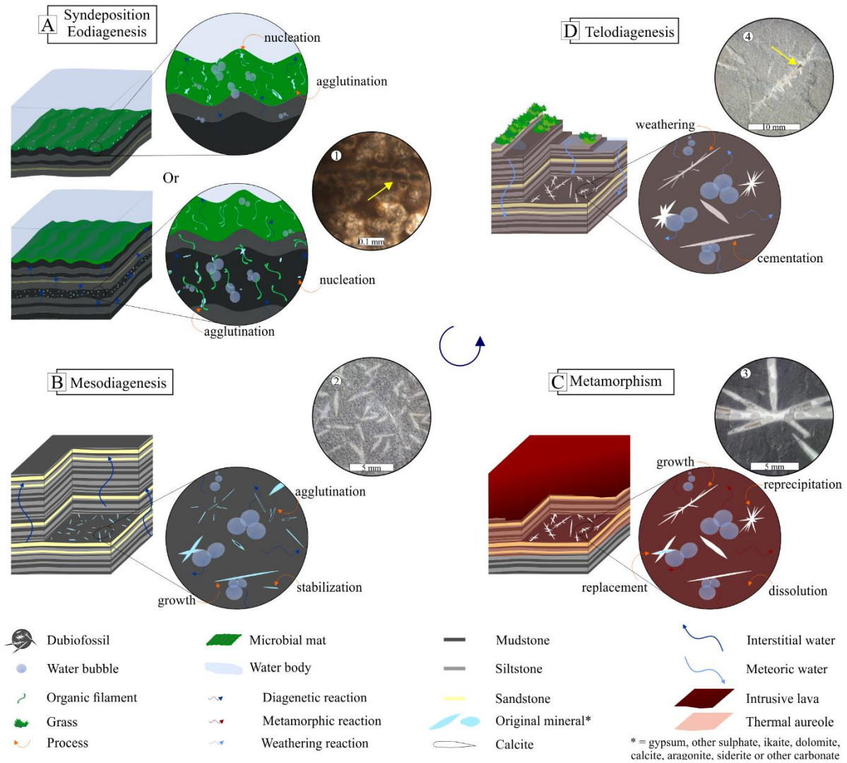
Figure 11: History of the formation of dubiofossils. A) Syndeositional or eodiagenesis associated with microbial mats, upper model deposition on the mat in life, lower, authigenesis in eodiagenesis by mat degradation; B) Mesodiagenesis and mineralization modifications; C) thermal effect, dissolution, modification, and replacement of the initial minerals by calcite and precipitation; D) telodiagenesis process of oxidation and cementation by hematite in recent exposure. 1-4) examples of the result of interpreted processes, yellow arrows points to crystals alignment on “filament” in 1 and cemented interior in 4. In each phase processes like nucleation, agglutination, stabilization, growth, dissolution, reprecipitation, replacement, cementation and weathering have acted to produce and modified the dubiofossils.
