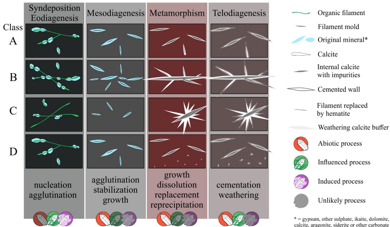
Figure 12: model of differences between morphological classes (A to D) generated by variations in matrix properties in each of the stages of the complex history of mineralization. Associated matrix: Class A - light gray siltstone; Class B - black to dark gray siltstone; Class C - black mudstone; Class D - dark to light gray siltstone. Different intensities of the processes occurred determining the morphologies and increasing the final morphological complexity. At each stage, the most likely process is indicated: biotic or abiotic, without being able to rule out the other hypotheses.
