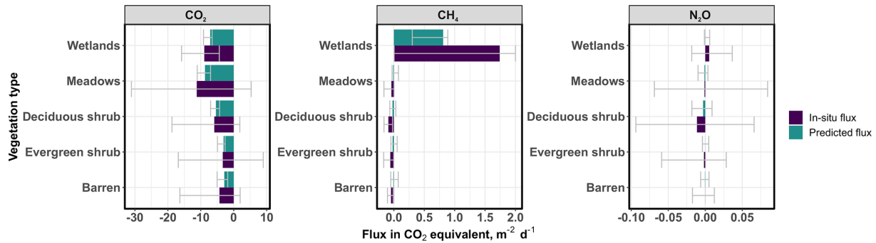
Figure 8. Growing season mean and percentile (0.025 and 0.975) GHG fluxes in \text{CO}_2 equivalents based on in situ data and upscaled flux predictions, averaged across the entire study period (only daytime variability between 08:00 and 20:00 considered) and across vegetation types. Note that the scale for the x axis is different for each gas species, and that the uncertainties in in situ versus predicted mean fluxes cannot be directly compared with each other. The uncertainty in in situ wetland \text{CH}_4 continues up to 6.7 but was cropped for visualization purposes. The same graph using the sustained GWP approach can be found in the Supplement Fig. 6 and demonstrates the potentially larger role of \text{CH}_4 fluxes over a 100-year horizon in this landscape.
