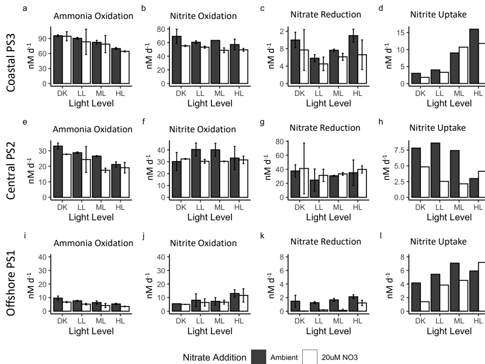
320 Figure 2. Rate measurements ( \text{nM d}^{-1} ) from experimental manipulation of light and nitrate using source water collected at coastal station PS3 (top row), central ODZ station PS2 (middle row) and offshore station PS1 (bottom row). Ammonia oxidation (a, e, i), nitrite oxidation (b, f, j), nitrate reduction (c, g, k) and nitrite uptake (d, h, l) are shown at each station with ambient nitrate concentration (solid bars) and 20 \mu\text{M} nitrate treatment (open bars) for each light condition (dark=DK, low light=LL, medium light=ML and high light=HL). Error bars depict standard error of replicate incubations where available.
