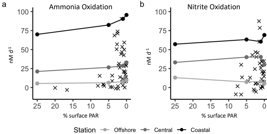
Figure 7. Experimental rates from light experiments (circles) plotted on top of ambient measurements (crosses) from the ETNP region. The % surface irradiances are from light level in experimental incubations tanks, or % surface irradiances from collection depth for ambient rates. Measurements from the same source water are connected with a line across the experimental light levels tested.
