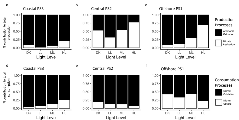
425 Figure 4. Relative contribution of production processes (top row) and consumption processes (bottom row) across light treatments at coastal PS3 (a,d), central PS2 (b,e) and offshore PS1 (c,f). Nitritification processes are black and phytoplankton processes are white. Ambient nitrate treatments only, does not include 20 \mu\text{M NO}_3^- treatments.
