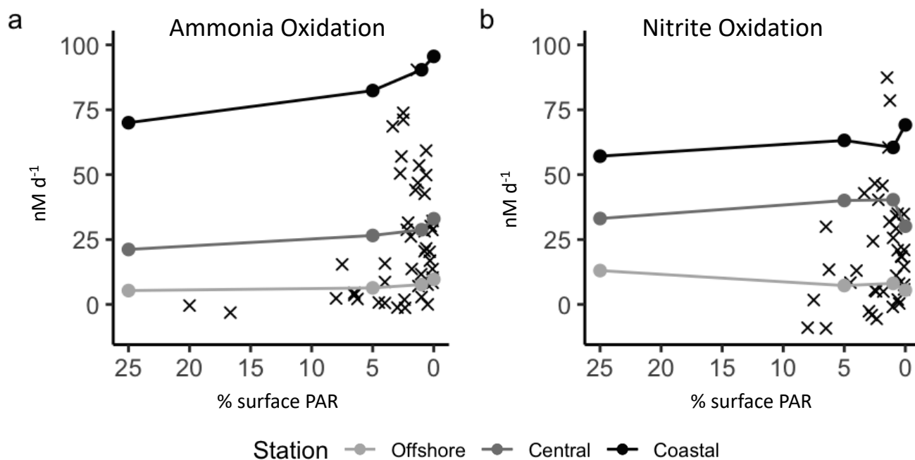
Figure 7. Experimental rates from light experiments (circles) plotted on top of ambient measurements (exes) from the ETNP region. The % surface irradiances are from light level in experimental incubations tanks, or % surface irradiances from collection depth for ambient rates. Measurements from the same source water are connected with a line across the experimental light levels tested.
