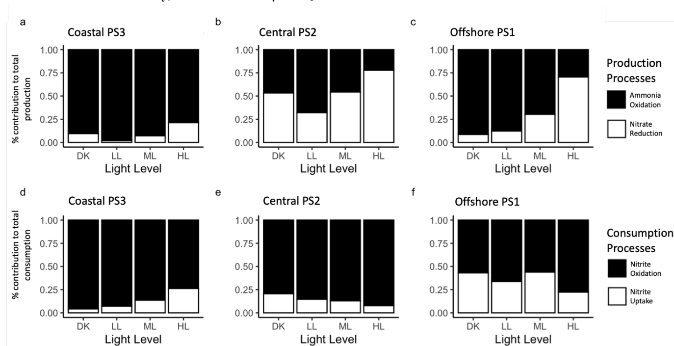
Figure 4. Relative contribution of production processes (top row) and consumption processes (bottom row) across light treatments at coastal PS3 (a,d), central PS2 (b,e) and offshore PS1 (c,f). Nitrification processes are black and phytoplankton processes are white. Ambient nitrate treatments only, does not include 20 \mu\text{M NO}_3^- treatments.
