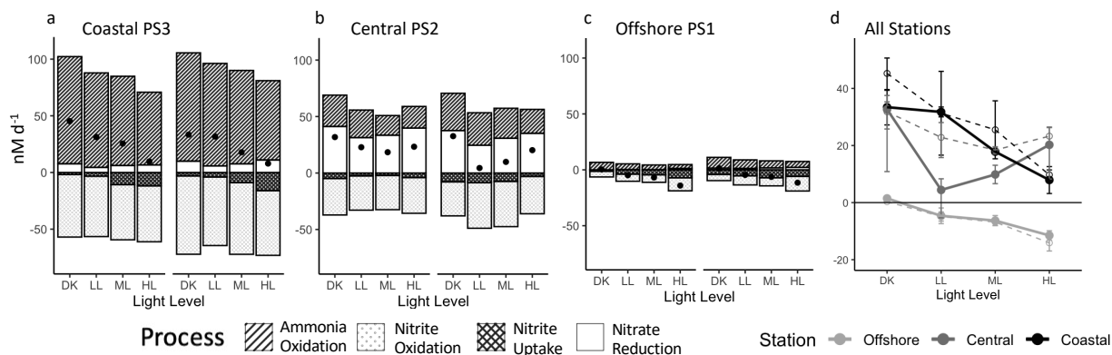
470 Figure 6. Component processes of net nitrite production (NetNO 2 ) at each station: coastal PS3 (a) central PS2 (b) and offshore PS1 (c). Positive values represent production of nitrite and negative values represent consumption of nitrite. The net nitrite production rates at each station are presented together in panel d, and overlaid as black dots on individual station panels a,b,c. The 20 μM NO 3 - treatments are on the left in panels a,b,c, and as dashed lines in panel d. Error bars are omitted, but presented in Figure 2 for individual rates. Pooled error is calculated for NetNO 2 (d).
