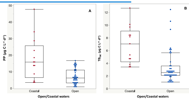
325 Figure 2: (A) Primary Production (PP) and (B) Total dark bacteria DIC fixation ( TB_{DIC} ) measured in open and coastal waters. Boxplots indicate the 95 % confidence intervals with \pm 1 SD deviation. The central line in the box represents the median for each group of samples.
