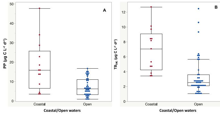
Figure 2: (A) Primary Production (PP) and (B) Total dark bacteria DIC fixation ( TB_{DIC} ) measured in coastal and open waters. Boxplots indicate the 95 % confidence intervals with \pm 1 SD deviation. The central line in the box represents the median for each group of samples.
