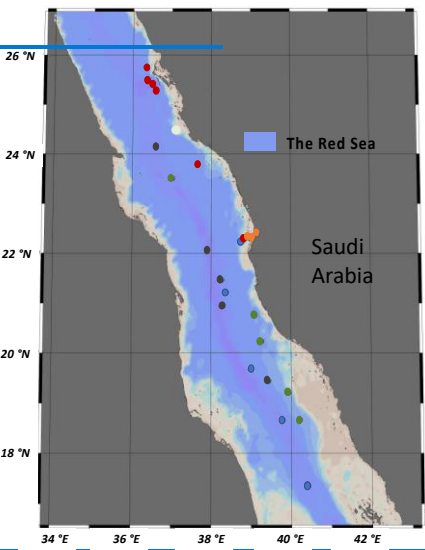
Figure 1: Stations sampled during the four oceanographic cruises [CCF (blue-blue dots), DC (green dots), DCS (red dots), RSDE (black-gray dots)] time series and coastal stations (orange dots) along the Eastern Red Sea conducted between 2017 and 2022.
