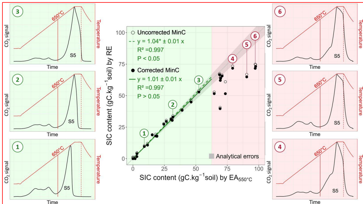
385 Figure 5: Plot of the SIC content estimated by the uncorrected (hollow-point) and the corrected (full-point) MinC parameter on one aliquot vs the SIC content estimated by EA_{550^{\circ}C} -after decarbonation on one aliquot for the 30 soils of the first panel. The coloured areas in green and red refer to SIC contents estimated by EA_{550^{\circ}C} lower ( n = 19 ) and higher ( n = 11 ) than 62.50 \text{ gC.kg}^{-1}\text{soil} , respectively. The equations of the linear regressions corrected MinC vs EA_{550^{\circ}C} (green bold line) and MinC vs EA_{550^{\circ}C} (green dashed line) correspond only to SIC contents < 62.50 \text{ gC.kg}^{-1}\text{soil} are provided with their coefficient of determination and their p-value. For both regressions, the slopes were significantly different from 0 ( P < 0.001 ) but not the intercepts ( P > 0.01 ). *The slope of the regression was significantly different from 1 ( P < 0.05 ). The oxidation thermograms presented on both sides of the plot are examples of the S4CO 2 and S5 curves obtained for six soils of the first panel: three with SIC contents < 62.50 \text{ gC.kg}^{-1}\text{soil} (N° 1-3) and three with SIC contents > 62.50 \text{ gC.kg}^{-1}\text{soil} (N° 4-6). The grey area, centred on the grey line y = x , represents the analytical measurement error of the two methods. On both sides of the plot, the S4CO 2 and S5 peaks were obtained during the oxidation phase of RE analyses of six soils (as examples). 390 395
