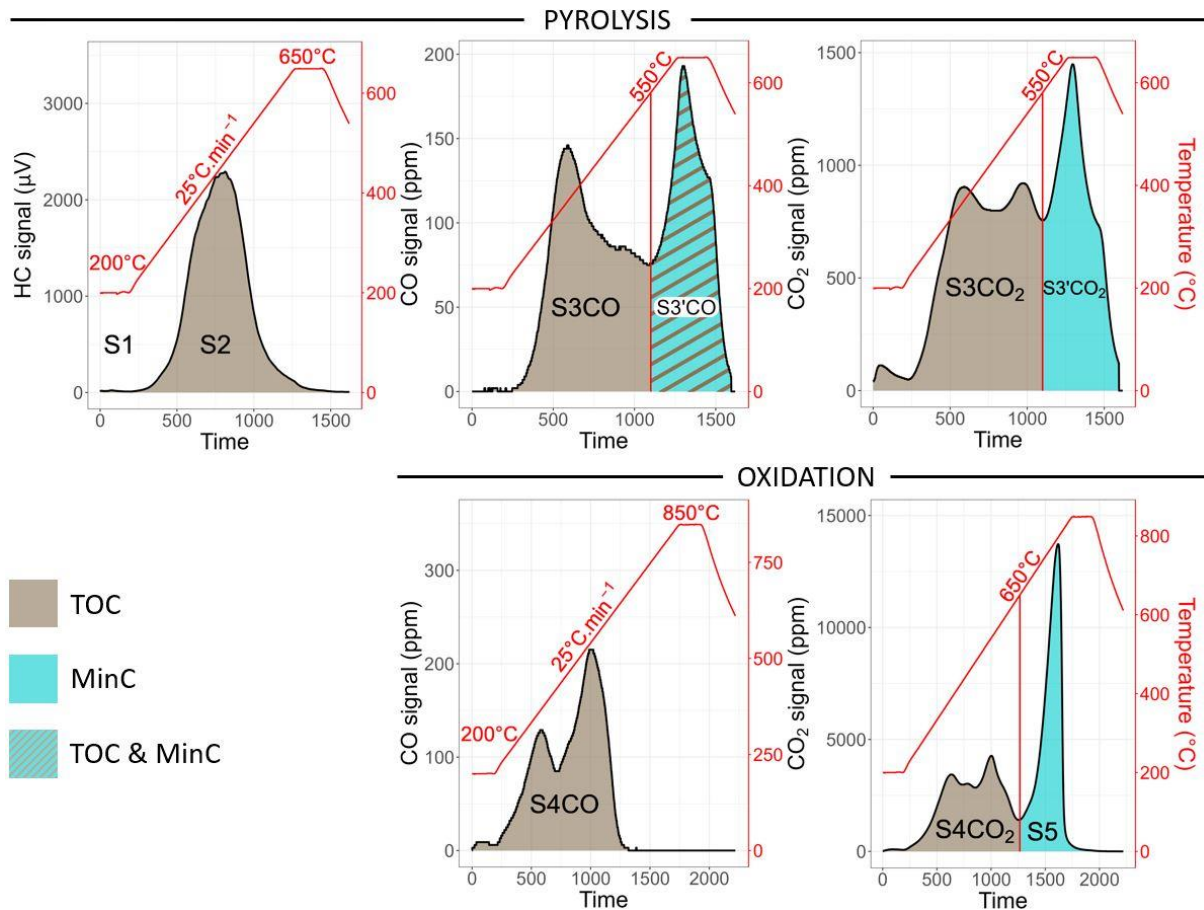
180 Figure 1: Principle of the Rock-Eval® analysis. The thermograms were obtained during the analysis of a soil with a SOC content of 15.7 gC.kg -1 soil and a SIC content of 11.6 gC.kg -1 soil with the Rock-Eval 6 standard device at the University of Lausanne. Example of the 5 thermograms and 9 curves (S1, S2, S3CO, S3'CO, S3CO 2 , S3'CO 2 , S4CO, S4CO 2 and S5) obtained during the Rock-Eval® analysis of a calcareous agricultural topsoil with a SOC content of 15.68 gC.kg -1 soil and a SIC content of 11.61 gC.kg -1 soil. The brown areas correspond to the curves formed by the pyrolytic cracking and the oxidative combustion of SOC and are integrated in the TOC parameter calculation. The blue areas correspond to the curves formed by the SIC thermal breakdown and are integrated in the MinC parameter calculation. The blue area with brown stripes corresponds to the curve formed by the SOC pyrolytic cracking and the SIC thermal breakdown and is integrated in both TOC and MinC parameters calculation. FID: Flame Ionization Detector; IR: InfraRed. 185
