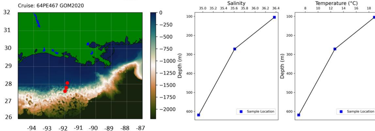
Figure 1: Left: sampling location in the Gulf of Mexico (GEMCO, 2022). Right: salinity and temperature data from CTD at bottom sample.
