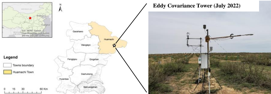
120 Figure 1. Overview of the study area. The red area in the map (from OpenStreetMap) is Yanchi County located in China. The white star denotes the field station located in Yangzhaizi village in Yanchi County, Ningxia Province.
