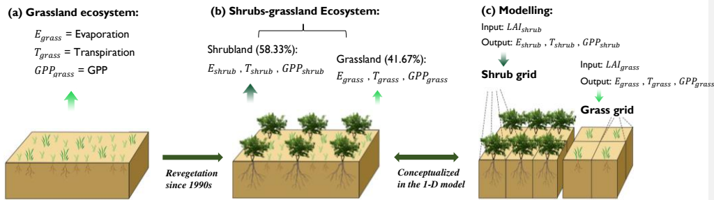
Figure 3. Conceptual diagram of (a) native grassland scenario before revegetation (hereafter is denoted as grassland ecosystem), (b) realistic scenario with mixed shrubs and grasses (hereafter is denoted as shrubs-grassland ecosystem) and (c) conceptualization in the model. The bare soil evaporation is implicitly included in E_{shrub} and E_{grass} , where E is the evaporation.
