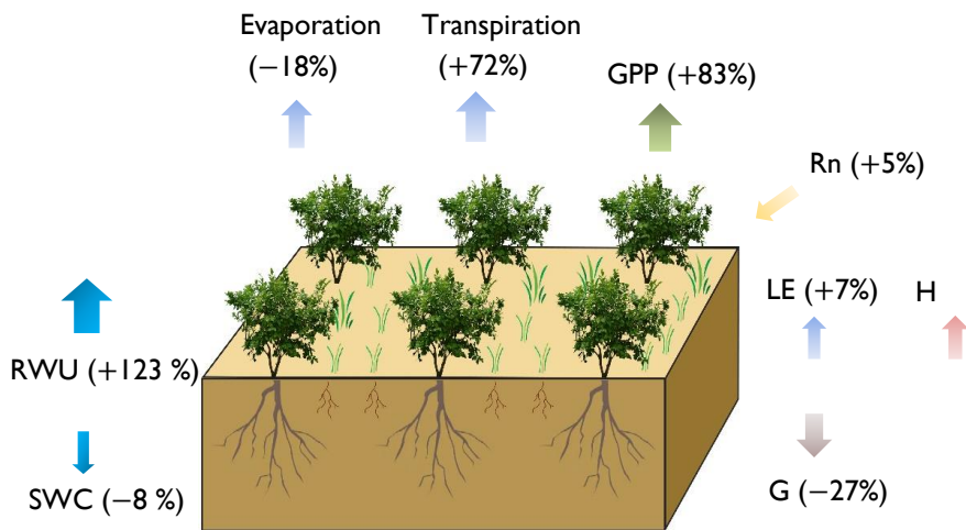
Figure 10. The changes in the energy, water and carbon fluxes caused by the revegetation, illustrated by the difference in averaged fluxes between shrubs-grassland ecosystem and grassland ecosystem. The arrows indicate the direction of the fluxes and the symbol ‘-’ represents a decrease while the ‘+’ represents an increase based on the grassland scenario.
