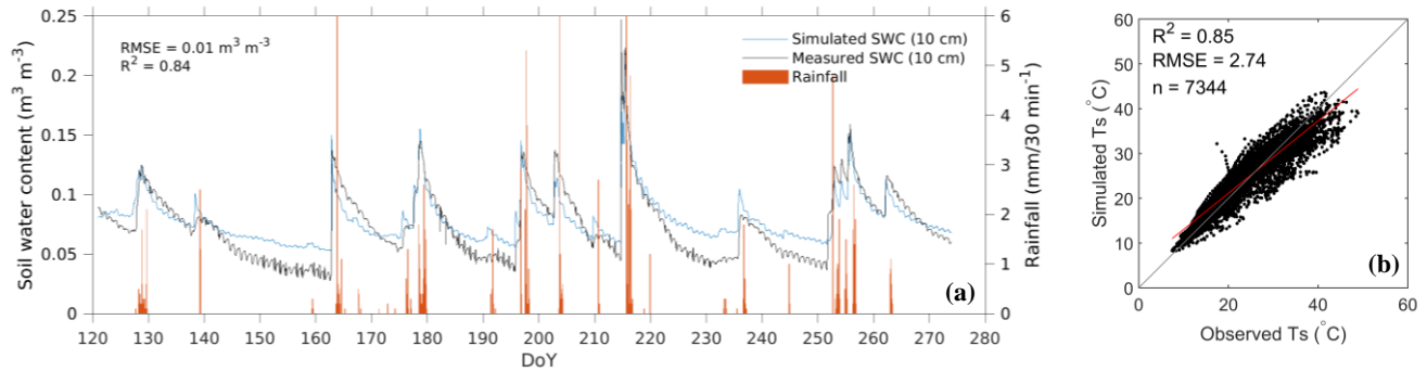
230 Figure 5. Model simulated and measured half-hourly soil water content (SWC) and (b) soil temperature (Ts) during May-September in 2019; (a) Temporal dynamics of SWC; (b) Scatter plots between the simulated and the observed Ts.
