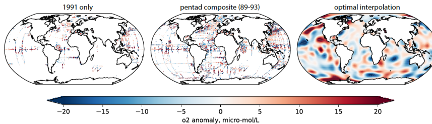
Figure 1. Maps of (left) single year observation for the O 2 anomaly in Year 1991 at 200m depth, (middle) the pentadal composite O 2 anomaly centered at Year 1991 covering from 1989 to 1993 at 200m depth, and (right) the optimally interpolated pentadal O 2 anomaly based on the data in the middle figure.
