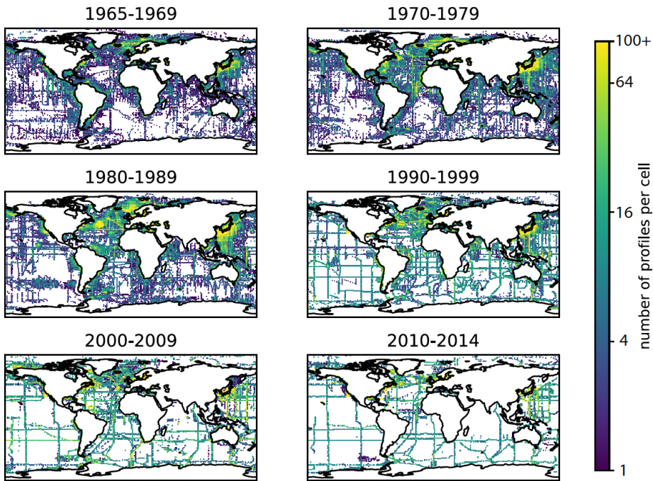
Figure 2. Number of OSD and CTD oxygen profiles aggregated into 1^{\circ}\times 1^{\circ} longitude-latitude grid cells for four decades from 1965 to 2014. The color scale indicates the number of measurements in log scale.
