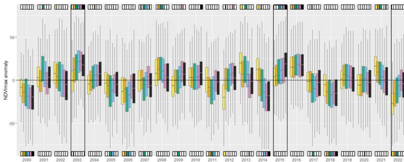
605 Figure 2: Anomalies of NDVImax for the six clusters. Time series of NDVImax were detrended using a monotonic function and the anomalies show the residual around the trend. Upper (lower) color chips indicate whether the collective, i.e. per cluster, anomaly was significantly above (or below) 0, based on a counting of signs test for random samples of 10% of the pixels per cluster. To ease reading, colored chips only indicate the most significant tests ( P < 0.001 ). The three rectangles point to the three major heat waves that have occurred in the Alps during the last two decades. Color legends of clusters are in Figure 1.
