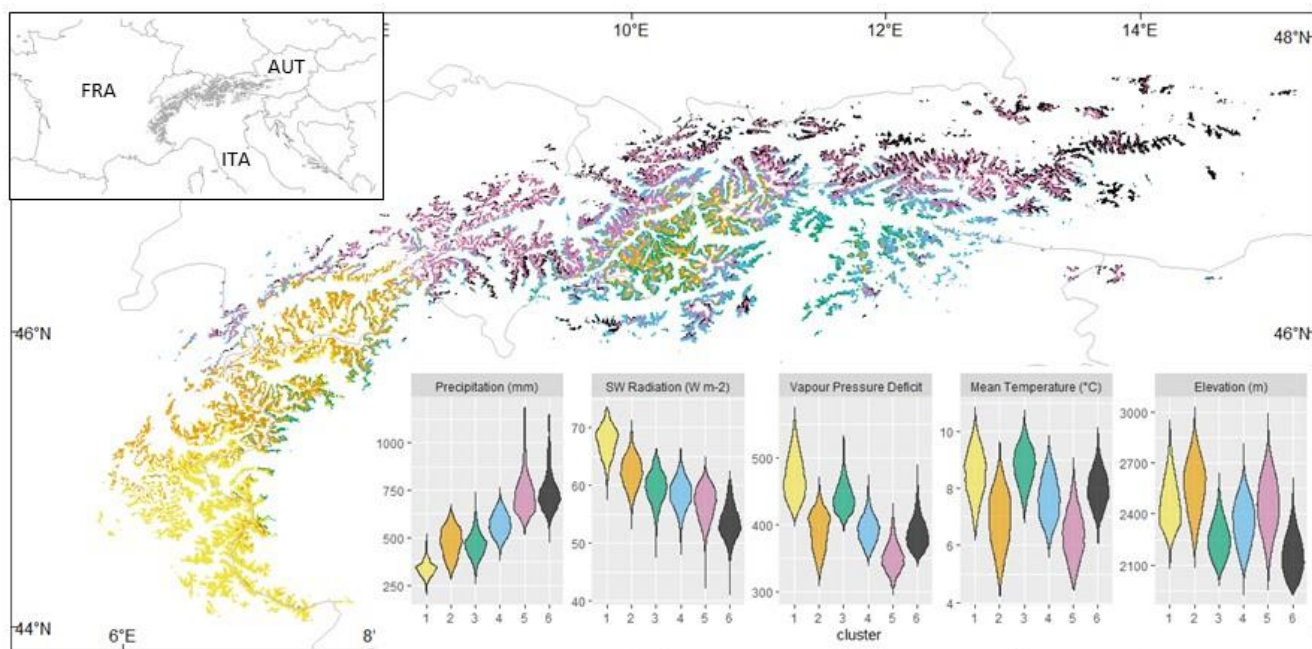
600 Figure 1: Geographical distribution of above-treeline ecosystems in the European Alps and delineation of the six subregions based on a clustering of summer climate averages for the reference period 1981-2010. The upper left panel shows the location of the study area. Violin plots in the lower right panels quantify the distribution of bioclimate values between clusters. Climate data were obtained from the high-resolution climatology CHELSA v2.1.
