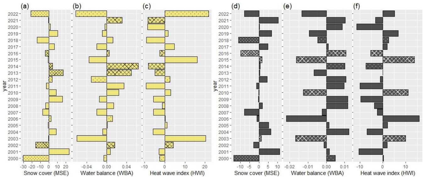
Figure 3: Anomalies of snow cover duration (MSE) and early summer meteorological variables (WBA, HWI) for cluster 1 (a, b, c) and cluster 6 (d, e, f). Crosshatched (dotted) bars indicate significant positive (negative) NDVImax anomalies. Similar figures for the other clusters are given in Supplement Figure 2.
