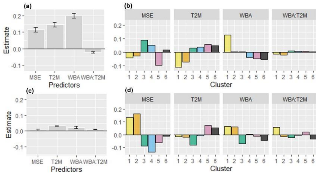
Figure 4: Estimates of the fixed effects (gray bars) and of the cluster random effects (colored bars) for the predictors of NDVImax variability. Panels a, b show results for the full period (2000-2022), and panels c, d show the differences between the second and the first 13-year long period. Data correspond to the best linear mixed effect model outlined in Table 1. See Material and methods for details.
