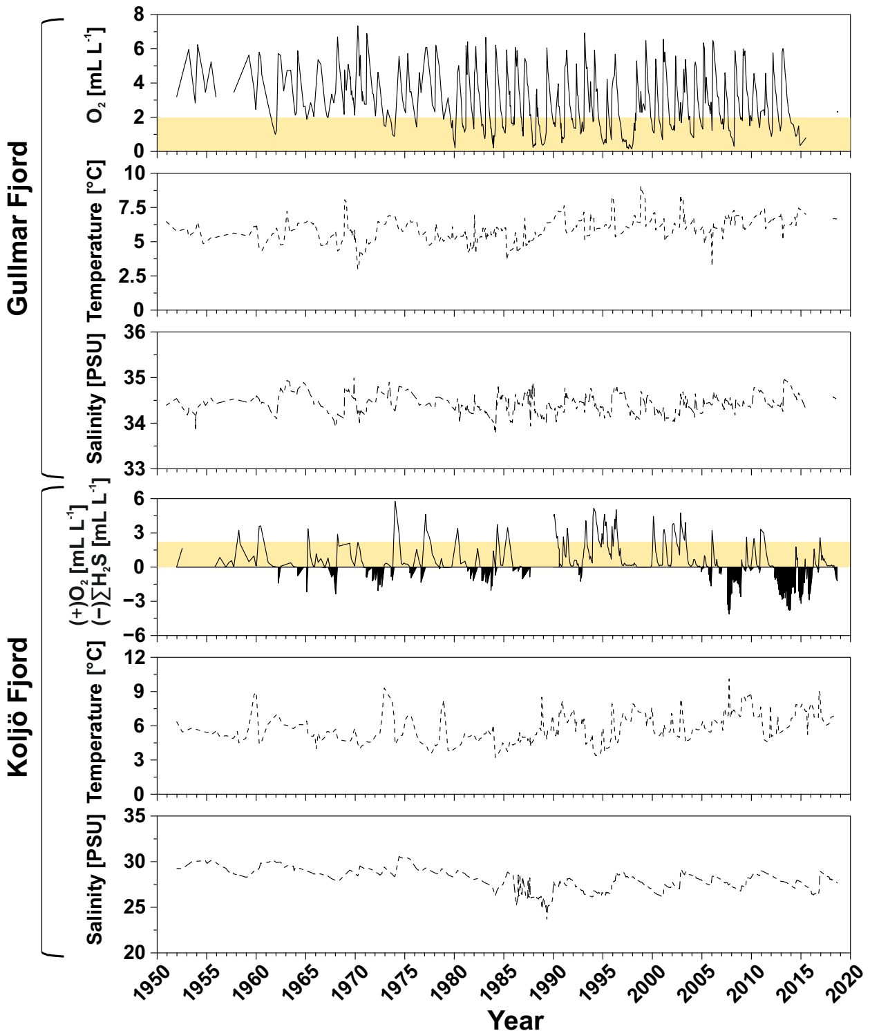
Figure 2. Bottom water monitoring data for Gullmar Fjord (upper three panels: O 2 , temperature, and salinity) and Koljö Fjord (lower three panels: O 2 – positive values, ΣH 2 S – expressed as negative O 2 , temperature, and salinity), recorded between 1950 and 2018 (SMHI, 2022). The yellow bars in the two O 2 panels indicate the dysoxic minimum and maximum boundary (0.2–2 mL L -1 ).
