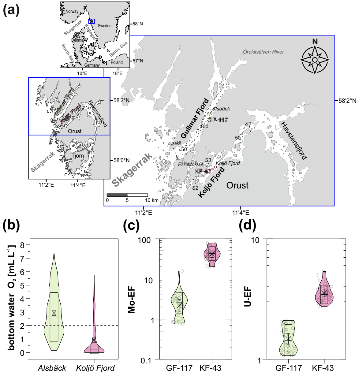
105 Figure 1. (a) Bathymetric map of the study area with the sites in Gullmar Fjord (GF-117, 58° 19.689'N, 11° 33.135'E, 115 m water depth) and Koljö Fjord (KF-43, 58° 13.624'N, 11° 34.265'E, 41.5 m water depth). Monitoring sites near both study sites “Alsbäck” (Alsbäck Deep, Gullmar Fjord, ~120 m water depth) and “Koljö Fjord” (Koljö Fjord, ~43 m water depth) are indicated by an empty circle next to the sampling locations. Map adapted from Brinkmann et al. (2023a). (b) Ranges in bottom water O 2 at the two monitoring sites from 1951–2018 (obtained from the publicly available Svenskt HavsARKiv (SHARK) database, https://sharkweb.smhi.se/hamta-data/ , provided by the Swedish Meteorological and Hydrological Institute, SMHI, 2022, last accessed: 03 September 2022), displayed as violin plots. The mean is indicated by a cross, and the 0.99 confidence interval (CI) of the mean by an error bar. The box within each violin plot represents the median absolute deviation (MAD) and horizontal line in each box shows the median. The dashed horizontal line marks the upper dysoxic threshold at 2 mL L -1 (Algeo and Li, 2020). The colors of the violin plots correspond to the color scheme used in Paul et al. (2023), illustrating the two “redox bins” 4 (ir/regularly dysoxic, light green) and 2 (ir/regularly euxinic, pink). (c) Molybdenum (Mo) enrichment factor (EF) and (d) Uranium (U) EF at both study locations from the September 2018 sampling campaign (original data and description of EF calculations are outlined in Paul et al., 2023). Color coding, and statistical features as in (b). Individual observations are shown (empty circles within each violin plot). 110 115
