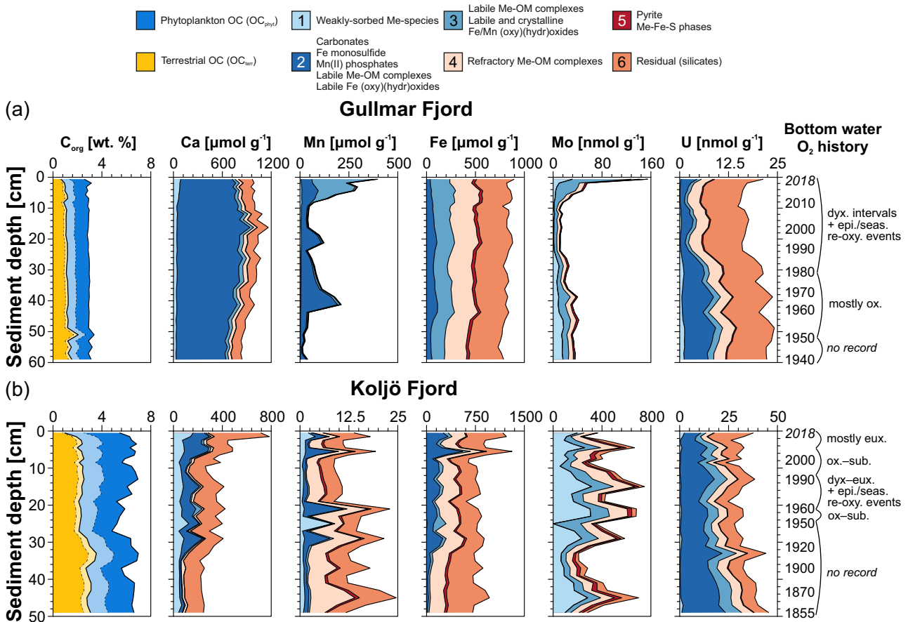
Figure 4. (a) Gullmar- and (b) Koljö Fjord downcore solid-phase distribution of C_{\text{org}} – divided into riverine-estuarine-phytoplankton-derived (blue) and terrestrial-plant-derived (yellow), and elemental Ca, Mn, Fe, Mo, and U contents – divided into six different fractions (F1–F6) based on the sequential extraction scheme (Table 1). In each C_{\text{org}} plot, the light-shaded area (light yellow, light blue) denotes the absolute range in OC_{\text{phyt}} and OC_{\text{terr}} fractions based on the maximum (N/C)_{\text{terr}} and (N/C)_{\text{phyt}} endmembers (dashed line), and minimum (N/C)_{\text{terr}} and (N/C)_{\text{phyt}} endmembers (dashed-dotted line), as reported in Goñi et al. (2003). The solid line denotes the OC_{\text{terr}}:OC_{\text{phyt}} contributions calculated when using the (N/C)_{\text{terr}} = 0.04 and (N/C)_{\text{phyt}} = 0.13 endmembers, as per Jilbert et al. (2018). A summary of bottom water O_2 history at both fjords is provided on the right. The bottom water redox conditions were derived from the fjord's monitoring data (Fig. 2, SMHI, 2022) and correlated to selected depth intervals in the sediment cores using the estimated age-depth models (section 3, Fig. S2a+b). The abbreviations used to describe the average bottom water (BW) redox condition are defined as follows (in order of appearance top to bottom): dyx = dysoxic, ox = oxic, epi. = episodic, seas. = seasonal, re-oxy. = re-oxygenation, eux = euxinic, and sub = suboxic.
