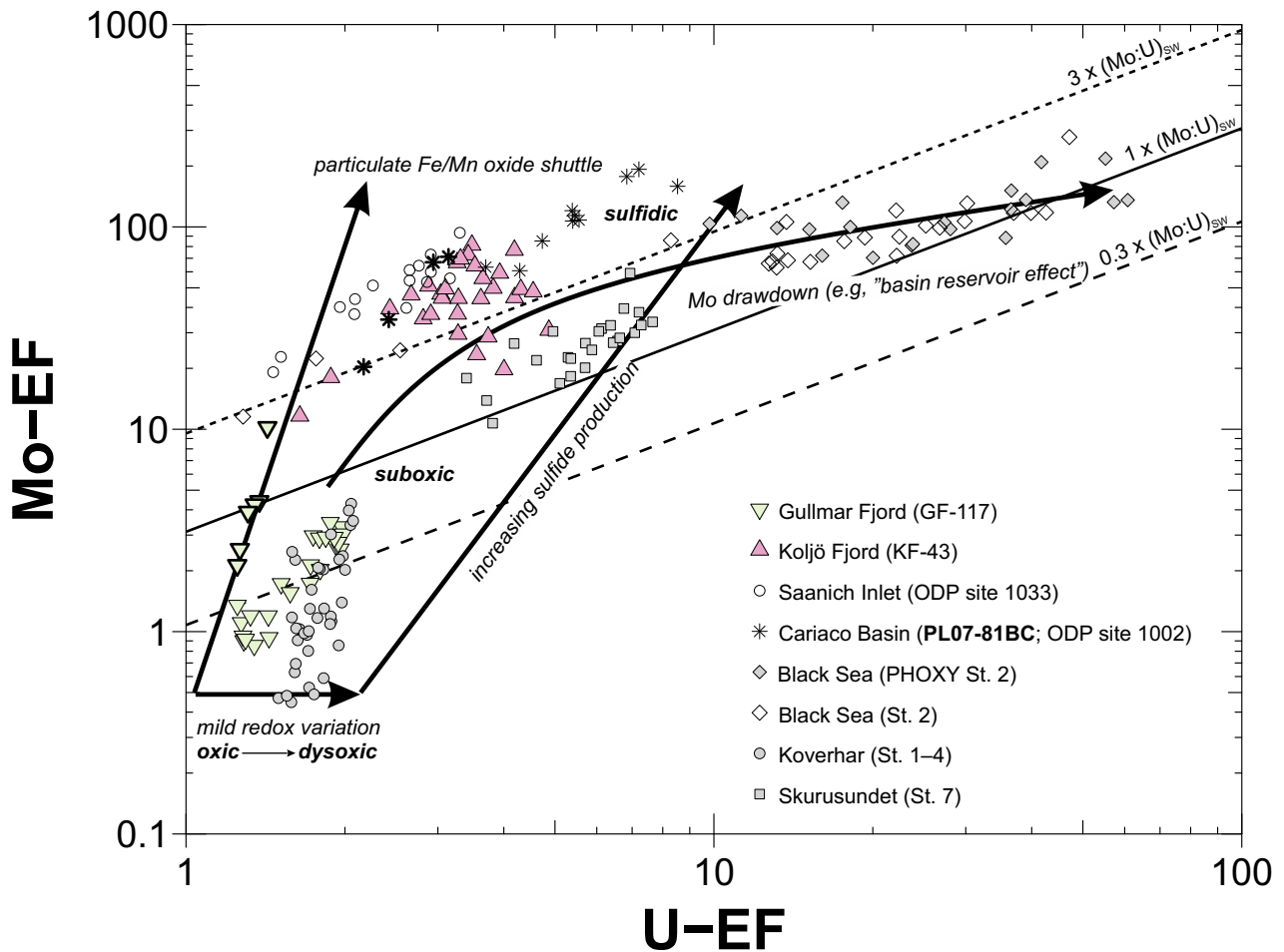
820 Figure 6. Sedimentary Mo-EF and U-EF covariation patterns at Gullmar Fjord (light green-filled reversed triangles) and Koljö Fjord (pink-filled triangles), relative to other coastal marine environments worldwide (unfilled symbols). Grey filled symbols depict data from a parallel study, Koverhar (St.1–4, circles), Skurusundet (St. 7, squares) and Black Sea (PHOXY St. 2, diamonds) (Paul et al., 2023). The four black arrows and letters denote key enrichment controls as described in Algeo and Tribovillard (2009) and the three diagonal lines denote multiples (0.3, 1, and 3) of the present-day seawater (SW) Mo:U ratio converted to an average weight ratio of 3.1 for the purpose of comparison with sediment Mo:U weight ratios (Tribovillard et al., 2012). Additional literature data are from Yano et al. (2020) – Saanich Inlet (ODP site 1033, unfilled circles), Cariaco Basin (ODP site 1002, plain stars), and Black Sea (St. 2, unfilled diamonds) – and Calvert et al. (2015) – Cariaco Basin (PL07-81BC, four samples, bold stars). Gullmar Fjord data is divided into two sub-patterns, the upper sediment section (0–7 cm) with the steepest Mo-/U-EF ratios, and the remaining sediment core (7–59 cm) with less steep Mo-/U-EF ratios (see text). 825 830
