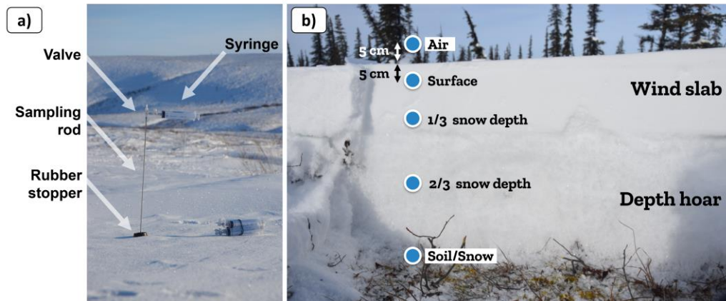
215 Figure 2: (a) Gas sampling equipment for the CO 2 concentration gradient measurement. (b) Typical snow depth profile of an Arctic snowpack (picture from Trail Valley Creek close to a tree patch).
