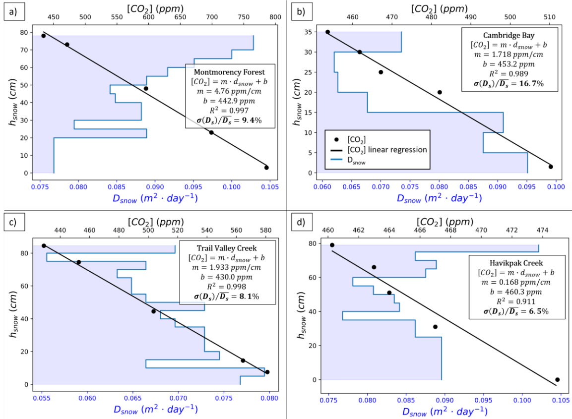
1015 Figure A3: Examples of snow diffusion coefficient ( D_{snow} = D_{air} \cdot \phi \cdot \tau ) vertical stratification and CO_2 concentration ( [CO_2] ) gradient measurements in function of snow height ( h_{snow} ) from the ground level. The coefficient of determination ( R^2 ), [CO_2] gradient ( m ) and y-axis intercept ( b ) for the linear regressions on the [CO_2] gradient measurements are provided. The ratio between D_{snow} standard deviation ( \sigma(D_s) ) and average ( \bar{D}_s ) is provided in percent. The data comes from (a) Montmorency Forest balsam fir closed-crown coniferous boreal forest on 2021-02-26, (b) Cambridge Bay prostrate-shrub tundra (hydic tundra: hydic sedge fen) on 2022-04-15, (c) Trail Valley Creek erect-shrub tundra (lichen) on 2022-03-26, and (d) Havikpak Creek black spruce open-crown coniferous boreal forest on 2022-03-16. 1020
