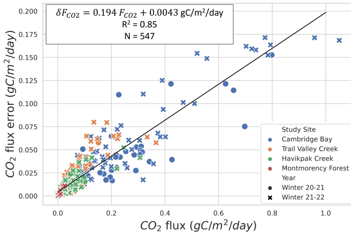
Figure 3: CO 2 flux ( F_{CO_2} ) uncertainty relationship to F_{CO_2} for four study sites and two winters 2020-2021 and 2021-2022. Specifications of the linear fit can be found in the upper left. The data dots color indicates the study site and its symbol (i.e., circle or x-shaped) indicates the winter during which it was collected.
