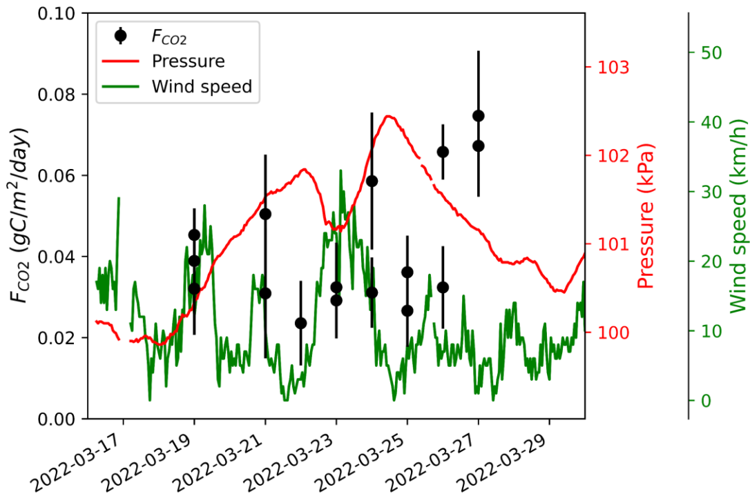
1005 Figure A1: CO_2 fluxes ( F_{CO_2} ) at a sampling location in the Trail Valley Creek erect-shrub tundra (lichen) between March 19 th and March 27 th , 2022. Atmospheric pressure and wind speed were obtained from Environment and Climate Change Canada's Meteorological Service of Canada meteorological station at Trail Valley Creek ( https://climate.weather.gc.ca/historical_data/search_historic_data_e.html ).
