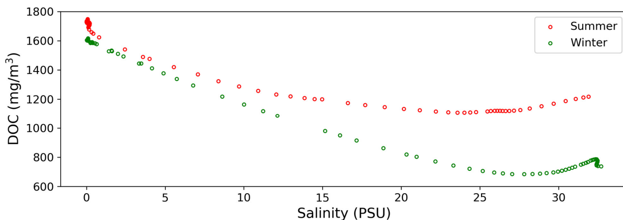
Figure 10. The surface average DOC varies along the profile (Fig. 2) as it mixes with the salinity gradient in summer and winter in the model. 4.4 Limitations and future research needs
