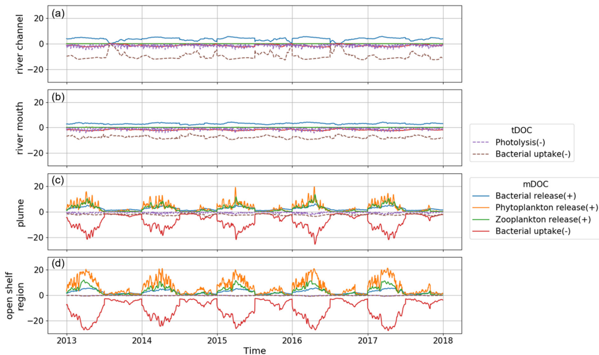
255 Figure 7. Daily vertical average rate (Units: \text{mg m}^{-3} \text{d}^{-1} ) of production (source) and consumption (sink) of tDOC (dashed lines) and mDOC (solid lines) in the four sub-regions. Positive values indicate sources, while negative values indicate sinks.
