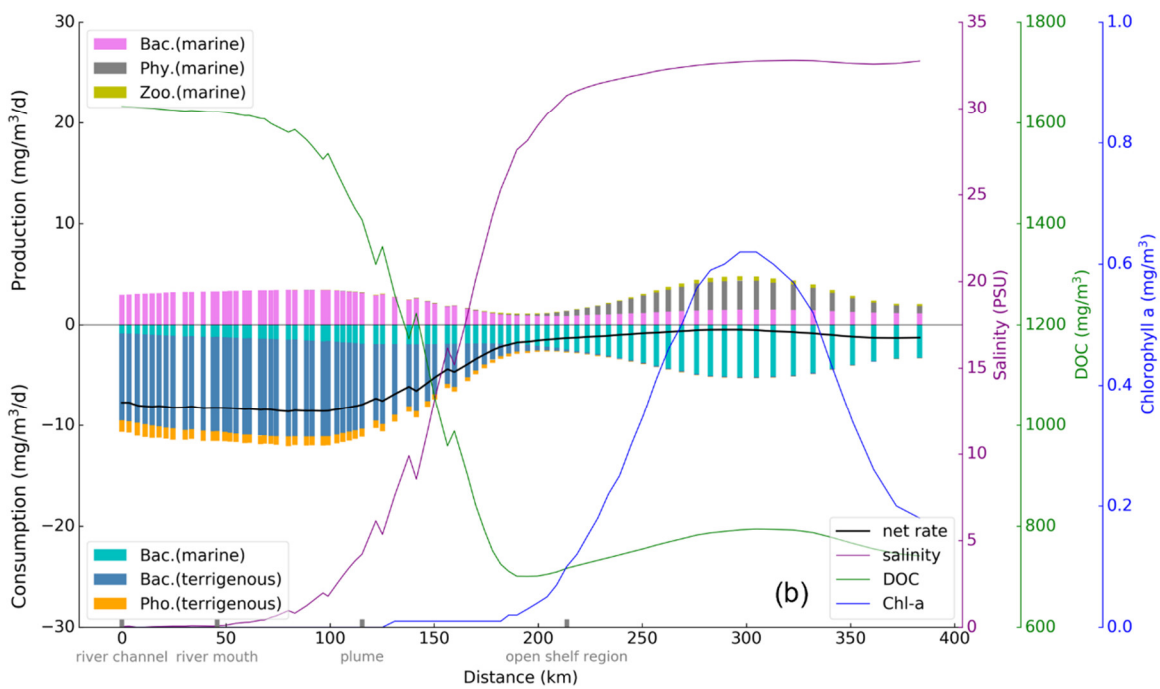
290 Figure 9. Vertical average production and consumption rates of DOC along the transect from the river channel to the shelf in summer (a) and winter (b).
