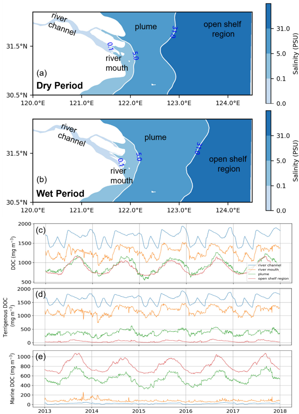
Figure 6. The partition of the model study area into four sub-regions based on the vertical average of salinity (a, b). The region with salinity less than 0.1 PSU is classified as the river channel, 0.1-5 PSU is the river mouth, 5-31 PSU is the plume, and the remainder region with salinity greater than 31 PSU is defined as an open shelf region. Time series of the concentration of total DOC (c) and its components tDOC (d) and mDOC (e) in the four sub-regions. Blue, orange, green, and red lines represent regions of river, river mouth, plume, and open shelf region, respectively, and all concentrations are regional vertical averages.
