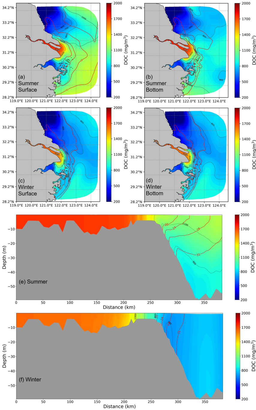
Figure 4. DOC spatial distribution from model is based on a five-year average for both surface and bottom layers (a-d) and vertical distribution (e, f) in summer and winter along the selected transect from river to shelf. The red contour lines represent salinity, while the black contour lines indicate DOC concentration.
