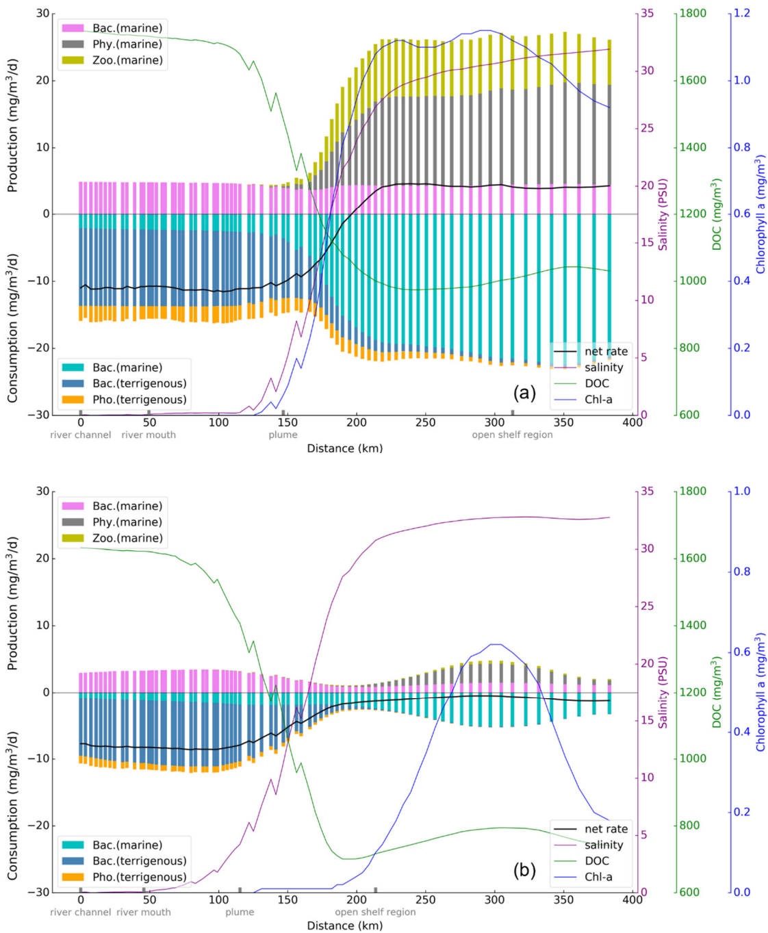
290 Figure 9. Vertical average production and consumption rates of DOC along the transect from the river channel to the shelf in summer (a) and winter (b).
