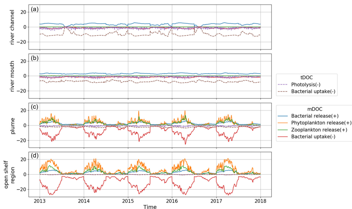
Figure 7. Daily vertical average rate (Units: \text{mg m}^{-3} \text{d}^{-1} ) of production (source) and consumption (sink) of tDOC (dashed lines) and mDOC (solid lines) in the four sub-regions. Positive values indicate sources, while negative values indicate sinks.
