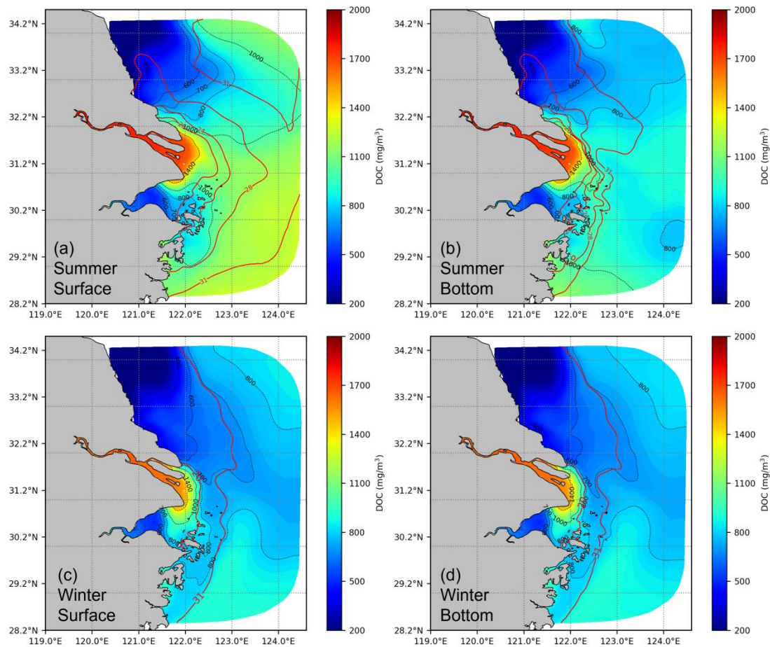
Figure S2. The simulated average distribution of DOC concentration for both the surface and bottom layer in summer and winter.
