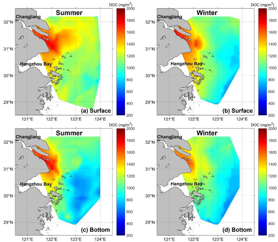
Figure S1. The observational average distribution of DOC concentration for both the surface and bottom layer in summer and winter.
